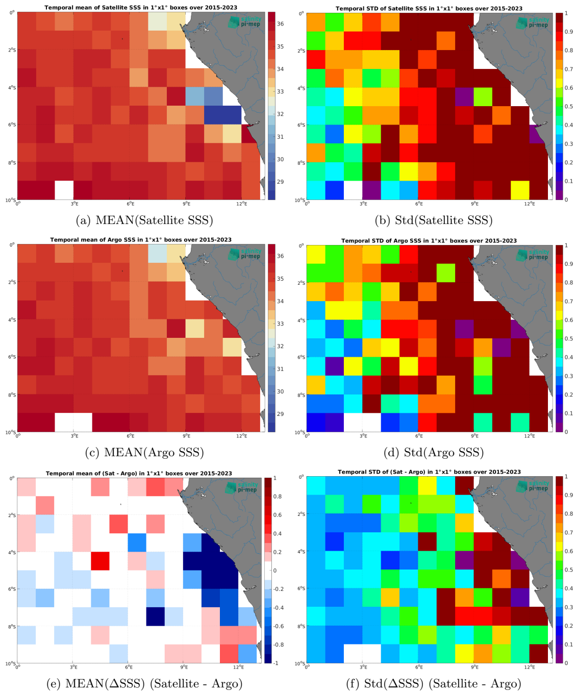
Figure 6: Temporal mean (left) and Std (right) of SSS from SMAP SSS L2 v5 (RSS) (top), Argo (middle), and of \Delta SSS (Satellite - Argo). Only match-up pairs are used to generate these maps.
