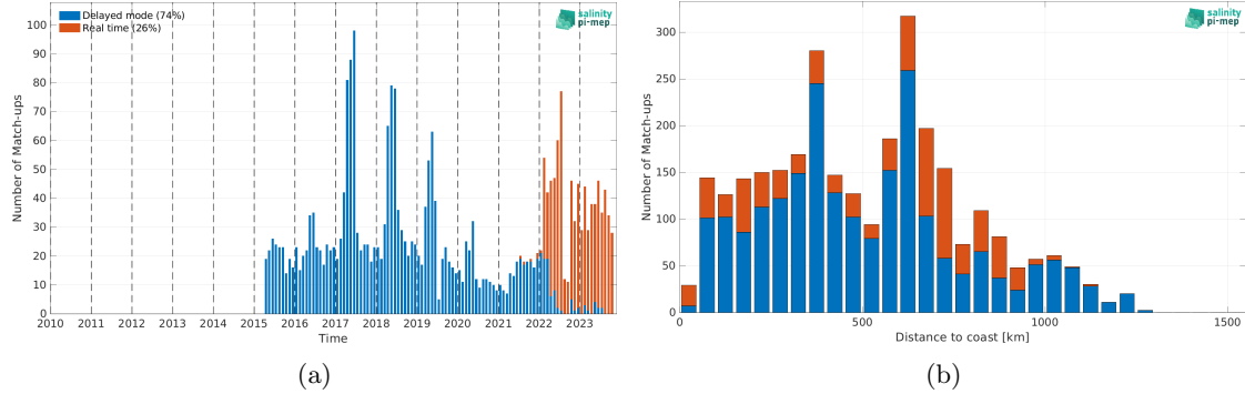
Figure 1: Number of match-ups between Argo and SMAP SSS L2 v5 (RSS) SSS as a function of time (a) and as function of the distance to coast (b) over the Congo river plume Pi-MEP region and for the full satellite product period.
