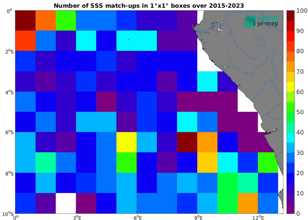
Figure 4: Number of SSS match-ups between Argo SSS and the SMAP SSS L2 v5 (RSS) SSS product for the Congo river plume Pi-MEP region over 1^{\circ} \times 1^{\circ} boxes and for the full satellite product period.
