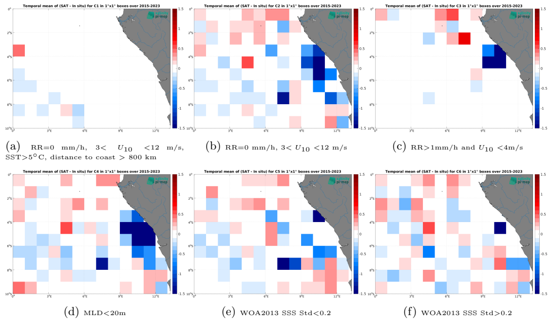
Figure 12: Temporal mean gridded over spatial boxes of size 1^\circ \times 1^\circ of \Delta SSS (SMAP SSS L2 v5 (RSS) - Argo) for 6 different subdatasets corresponding to:RR=0 mm/h, 3 < U_{10} < 12 m/s, SST > 5^\circ\text{C} , distance to coast > 800 km (a), RR=0 mm/h, 3 < U_{10} < 12 m/s (b), RR > 1 mm/h and U_{10} < 4 m/s (c),MLD < 20 m (d),WOA2013 SSS Std < 0.2 (e),WOA2013 SSS Std > 0.2 (f).
