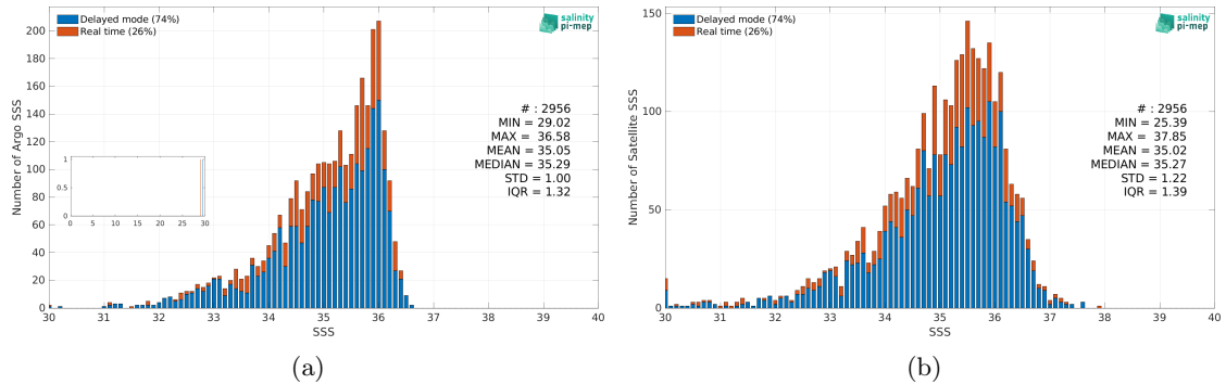
Figure 2: Histograms of SSS from Argo (a) and SMAP SSS L2 v5 (RSS) (b) considering all match-up pairs per bins of 0.1 over the Congo river plume Pi-MEP region and for the full satellite product period.
