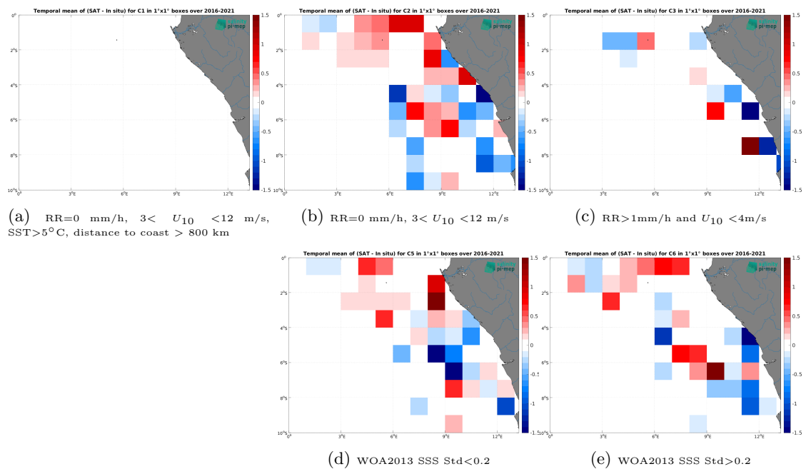
Figure 14: Temporal mean gridded over spatial boxes of size 1^\circ \times 1^\circ of \Delta SSS (SMAP SSS L2 v5.3 (RSS) - TSG (LEGOS-DM)) for 5 different subdatasets corresponding to:RR=0 mm/h, 3 < U_{10} < 12 m/s, SST > 5^\circ C , distance to coast > 800 km (a), RR=0 mm/h, 3 < U_{10} < 12 m/s (b), RR>1mm/h and U_{10} < 4 m/s (c), WOA2013 SSS Std<0.2 (d), WOA2013 SSS Std>0.2 (e).
