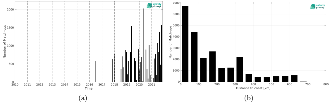
Figure 2: Number of match-ups between TSG (LEGOS-DM) and SMAP SSS L2 v5.3 (RSS) SSS as a function of time (a) and as function of the distance to coast (b) over the Congo river plume Pi-MEP region and for the full satellite product period.
