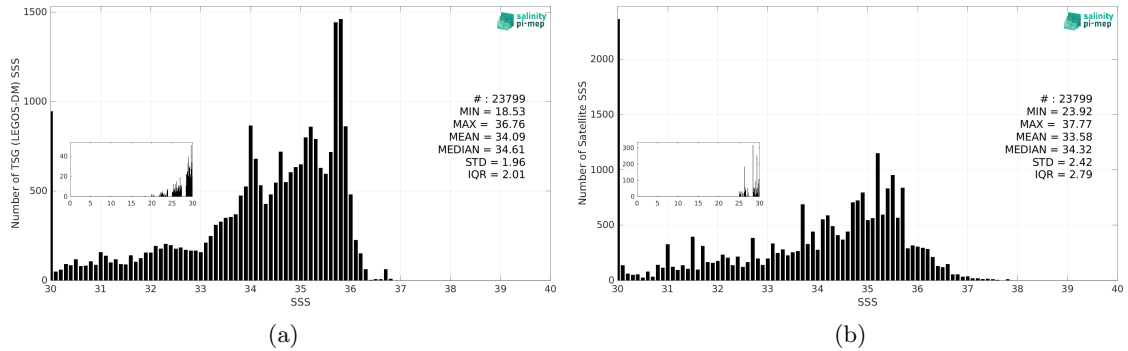
Figure 3: Histograms of SSS from TSG (LEGOS-DM) (a) and SMAP SSS L2 v5.3 (RSS) (b) considering all match-up pairs per bins of 0.1 over the Congo river plume Pi-MEP region and for the full satellite product period.
