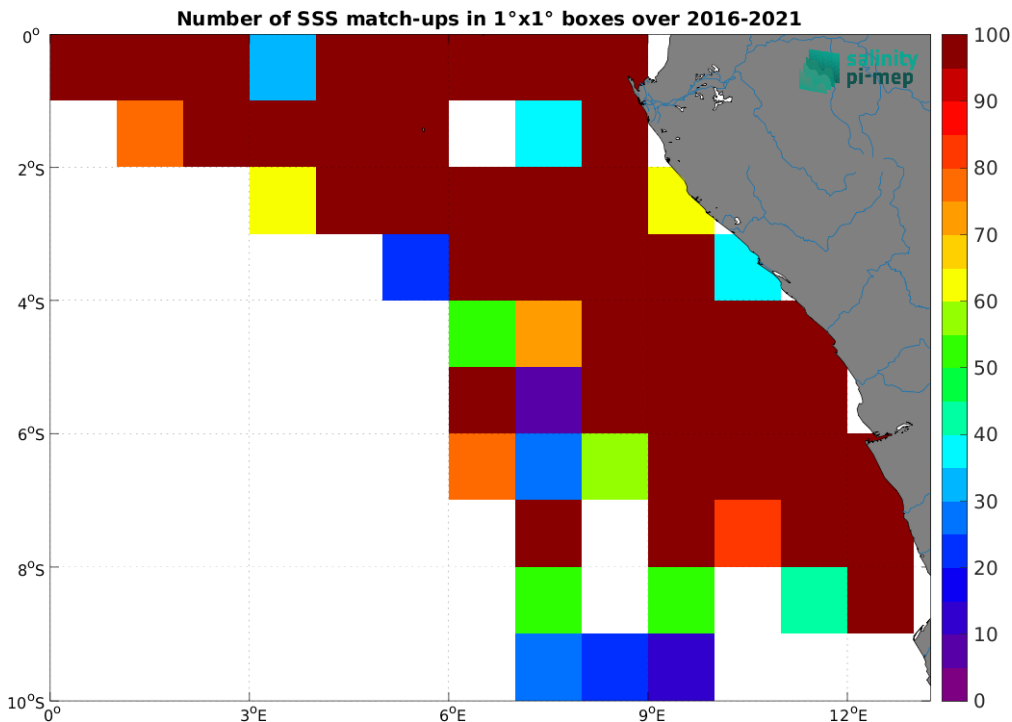
Figure 5: Number of SSS match-ups between TSG (LEGOS-DM) SSS and the SMAP SSS L2 v5.3 (RSS) SSS product for the Congo river plume Pi-MEP region over 1^\circ \times 1^\circ boxes and for the full satellite product period.
