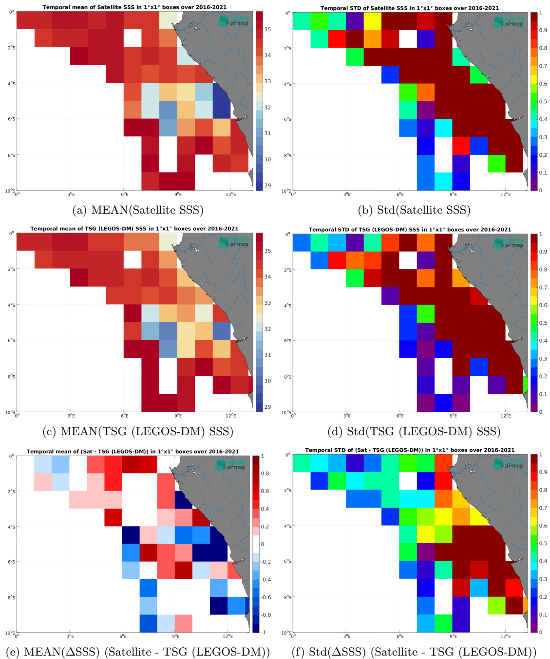
Figure 7: Temporal mean (left) and Std (right) of SSS from SMAP SSS L2 v5.3 (RSS), TSG (LEGOS-DM) (middle), and of \Delta SSS (Satellite - TSG (LEGOS-DM)). Only match-up pairs are used to generate these maps.
