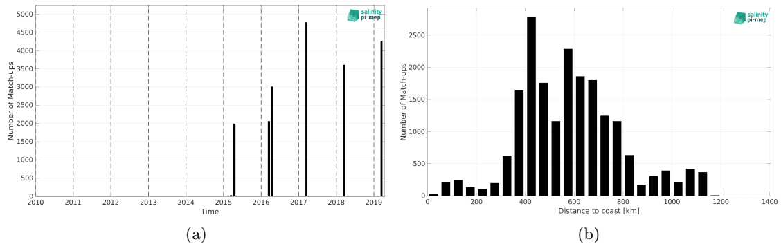
Figure 2: Number of match-ups between TSG (GOSUD-Research-vessel) and SMAP SSS L2 v5.3 (RSS) SSS as a function of time (a) and as function of the distance to coast (b) over the Congo river plume Pi-MEP region and for the full satellite product period.
