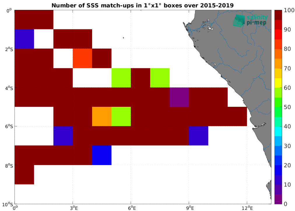
Figure 5: Number of SSS match-ups between TSG (GOSUD-Research-vessel) SSS and the SMAP SSS L2 v5.3 (RSS) SSS product for the Congo river plume Pi-MEP region over 1^{\circ} \times 1^{\circ} boxes and for the full satellite product period.
