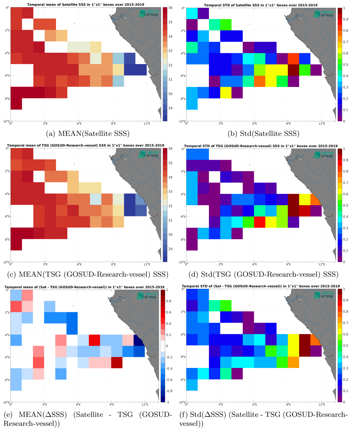
Figure 7: Temporal mean (left) and Std (right) of SSS from SMAP SSS L2 v5.3 (RSS) (top), TSG (GOSUD-Research-vessel) (middle), and of \Delta SSS (Satellite - TSG (GOSUD-Research-vessel)). Only match-up pairs are used to generate these maps.
