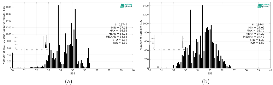
Figure 3: Histograms of SSS from TSG (GOSUD-Research-vessel) (a) and SMAP SSS L2 v5.3 (RSS) (b) considering all match-up pairs per bins of 0.1 over the Congo river plume Pi-MEP region and for the full satellite product period.
