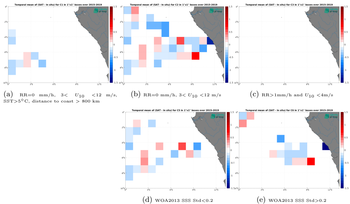
Figure 14: Temporal mean gridded over spatial boxes of size 1^\circ \times 1^\circ of \Delta SSS (SMAP SSS L2 v5.3 (RSS) - TSG (GOSUD-Research-vessel)) for 5 different subdatasets corresponding to: RR=0 mm/h, 3 < U_{10} < 12 m/s, SST > 5°C, distance to coast > 800 km (a), RR=0 mm/h, 3 < U_{10} < 12 m/s (b), RR > 1mm/h and U_{10} < 4 m/s (c), WOA2013 SSS Std < 0.2 (d), WOA2013 SSS Std > 0.2 (e).
