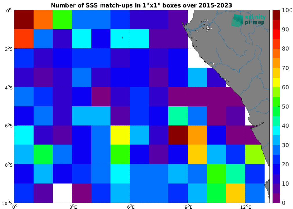
Figure 5: Number of SSS match-ups between Argo SSS and the SMAP SSS L2 v5.3 (RSS) SSS product for the Congo river plume Pi-MEP region over 1^\circ \times 1^\circ boxes and for the full satellite product period.
