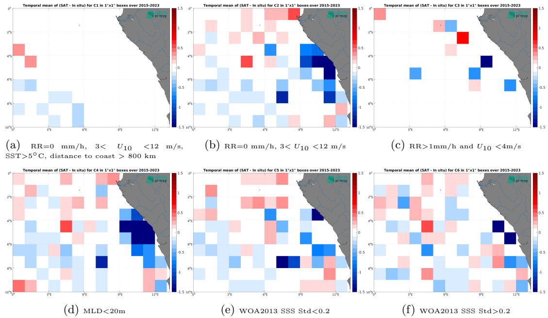
Figure 14: Temporal mean gridded over spatial boxes of size 1^\circ \times 1^\circ of \Delta SSS (SMAP SSS L2 v5.3 (RSS) - Argo) for 6 different subdatasets corresponding to:RR=0 mm/h, 3 < U_{10} < 12 m/s, SST>5°C, distance to coast > 800 km (a), RR=0 mm/h, 3 < U_{10} < 12 m/s (b), RR>1mm/h and U_{10} < 4 m/s (c),MLD<20m (d),WOA2013 SSS Std<0.2 (e),WOA2013 SSS Std>0.2 (f).
