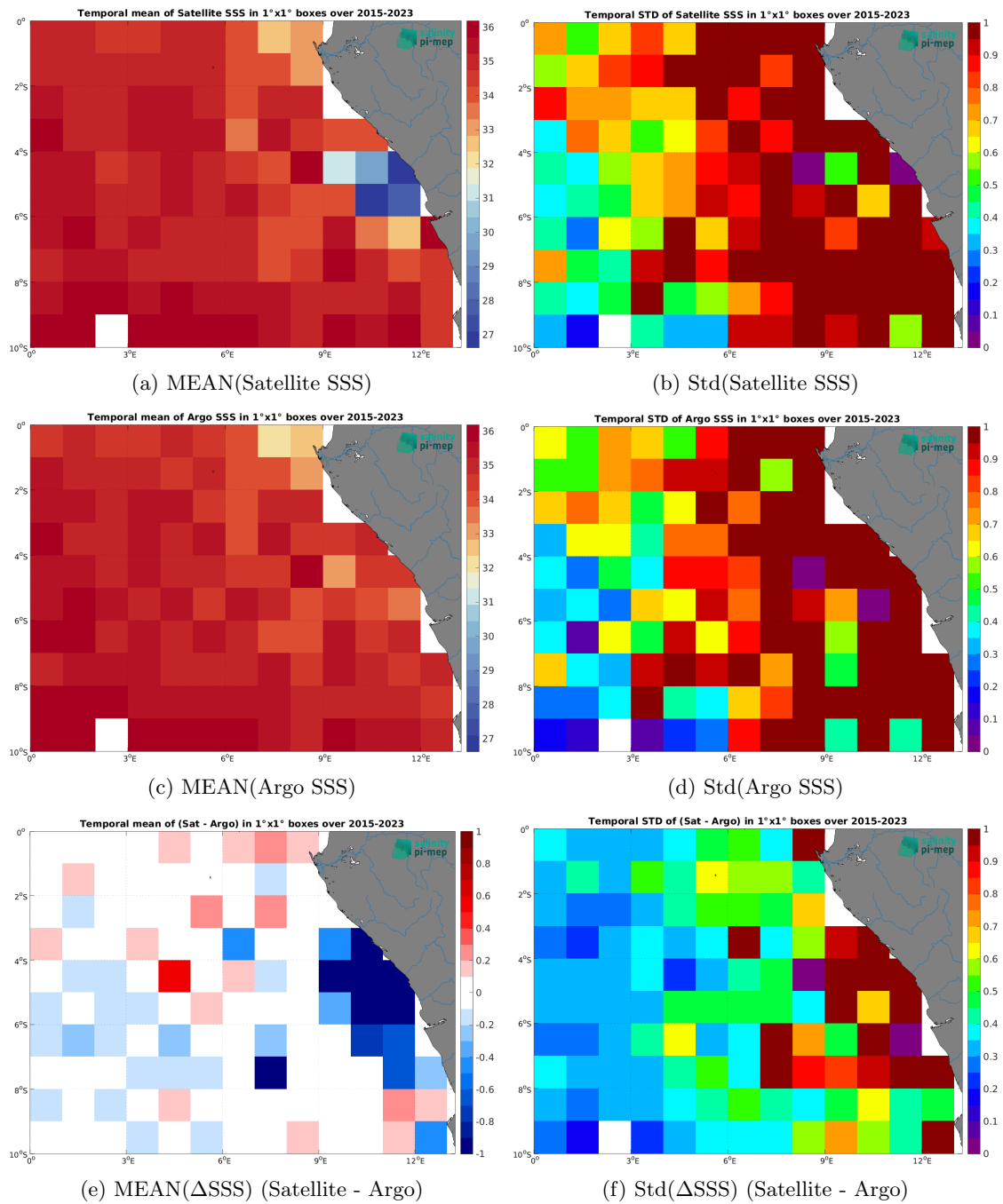
Figure 7: Temporal mean (left) and Std (right) of SSS from SMAP SSS L2 v5.3 (RSS) (top), Argo (middle), and of \Delta SSS (Satellite - Argo). Only match-up pairs are used to generate these maps.
