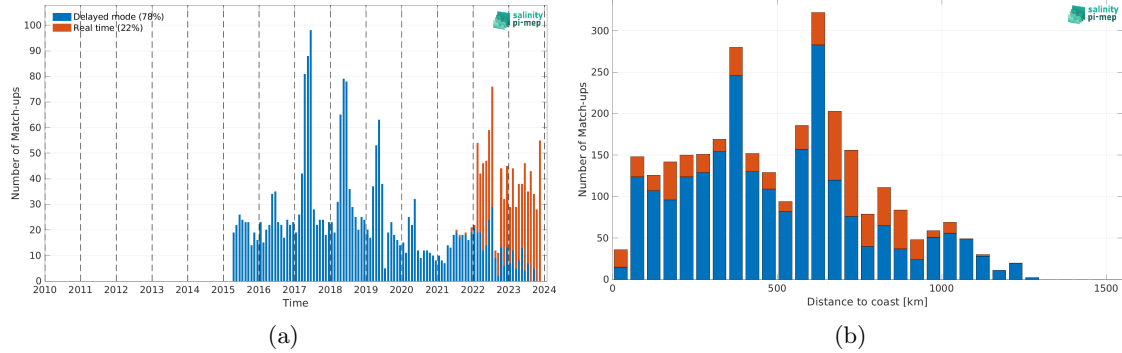
Figure 2: Number of match-ups between Argo and SMAP SSS L2 v5.3 (RSS) SSS as a function of time (a) and as function of the distance to coast (b) over the Congo river plume Pi-MEP region and for the full satellite product period.
