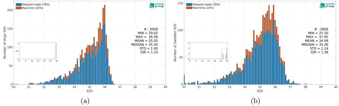
Figure 3: Histograms of SSS from Argo (a) and SMAP SSS L2 v5.3 (RSS) (b) considering all match-up pairs per bins of 0.1 over the Congo river plume Pi-MEP region and for the full satellite product period.
