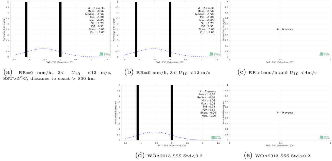
Figure 13: Normalized histogram of \Delta\text{SSS} (SMAP SSS L2 v5 - 40 km (RSS) - TSG (Polarstern)) for 5 different subdatasets corresponding to: RR=0 mm/h, 3 < U_{10} < 12 m/s, SST > 5^\circ\text{C} , distance to coast > 800 km (a), RR=0 mm/h, 3 < U_{10} < 12 m/s (b), RR > 1\text{mm/h} and U_{10} < 4\text{m/s} (c), WOA2013 SSS Std < 0.2 (d), WOA2013 SSS Std > 0.2 (e).
