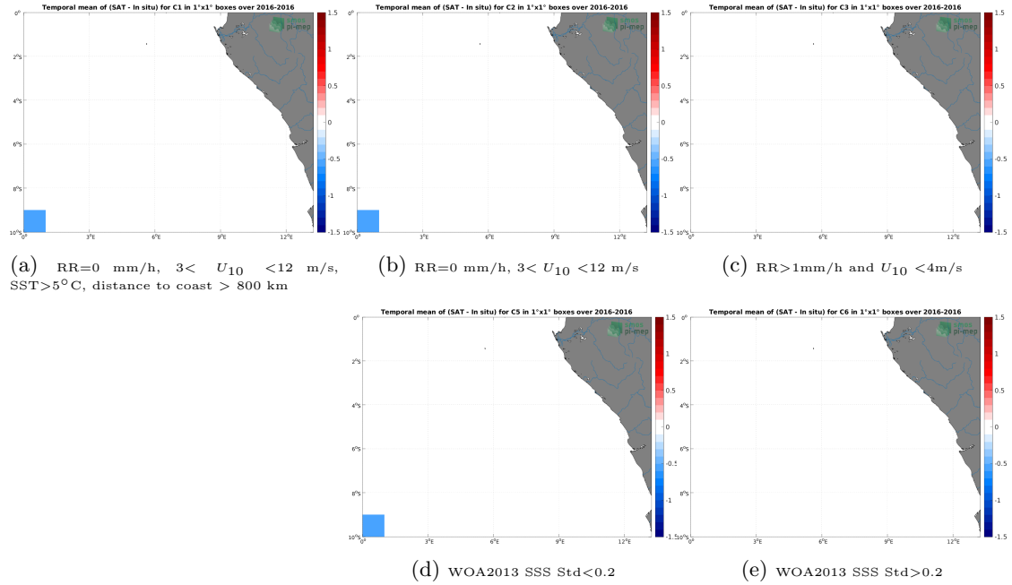
Figure 12: Temporal mean gridded over spatial boxes of size 1^{\circ}\times 1^{\circ} of \Delta\text{SSS} (SMAP SSS L2 v5 - 40 km (RSS) - TSG (Polarstern)) for 5 different subdatasets corresponding to:RR=0 mm/h, 3 < U_{10} < 12 m/s, SST >5^{\circ}\text{C} , distance to coast > 800 km (a), RR=0 mm/h, 3 < U_{10} < 12 m/s (b), RR >1 mm/h and U_{10} < 4 m/s (c), WOA2013 SSS Std <0.2 (d), WOA2013 SSS Std >0.2 (e).
