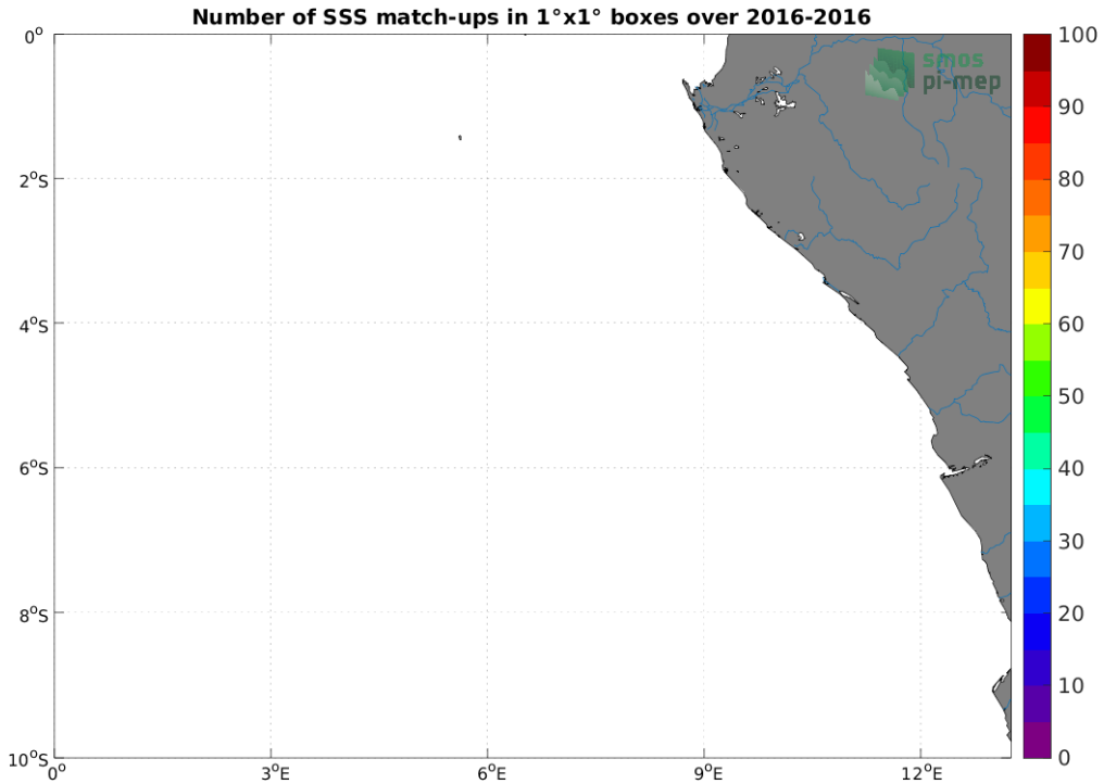
Figure 4: Number of SSS match-ups between TSG (Polarstern) SSS and the SMAP SSS L2 v5 - 40 km (RSS) SSS product for the Congo river plume Pi-MEP region over 1°×1° boxes and for the full satellite product period.
