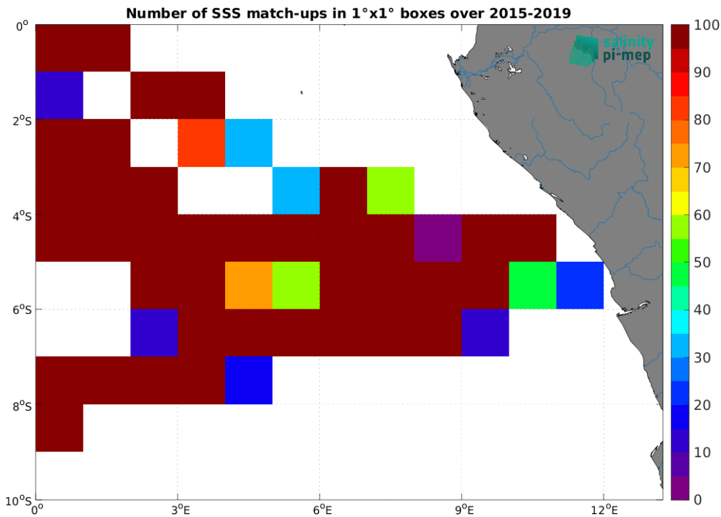
Figure 4: Number of SSS match-ups between TSG (GOSUD-Research-vessel) SSS and the SMAP SSS L2 v5 - 40 km (RSS) SSS product for the Congo river plume Pi-MEP region over 1°x1° boxes and for the full satellite product period.
