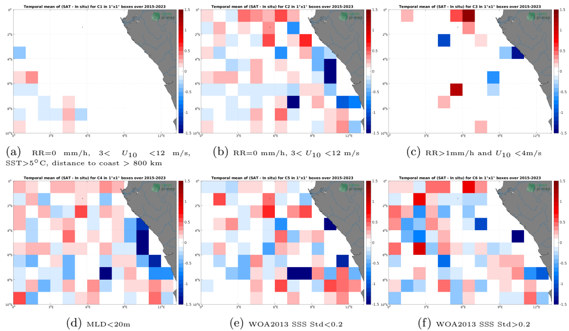
Figure 12: Temporal mean gridded over spatial boxes of size 1^\circ \times 1^\circ of \Delta SSS (SMAP SSS L2 v5 - 40 km (RSS) - Argo) for 6 different subdatasets corresponding to:RR=0 mm/h, 3 < U_{10} < 12 m/s, SST >5^\circ C, distance to coast > 800 km (a), RR=0 mm/h, 3 < U_{10} < 12 m/s (b), RR >1 mm/h and U_{10} < 4 m/s (c),MLD <20 m (d),WOA2013 SSS Std <0.2 (e),WOA2013 SSS Std >0.2 (f).
