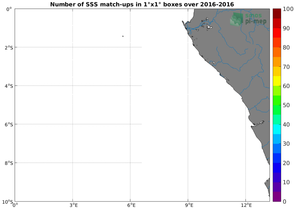
Figure 4: Number of SSS match-ups between TSG (Polarstern) SSS and the SMAP SSS L2 v4 (RSS) SSS product for the Congo river plume Pi-MEP region over 1°×1° boxes and for the full satellite product period.
