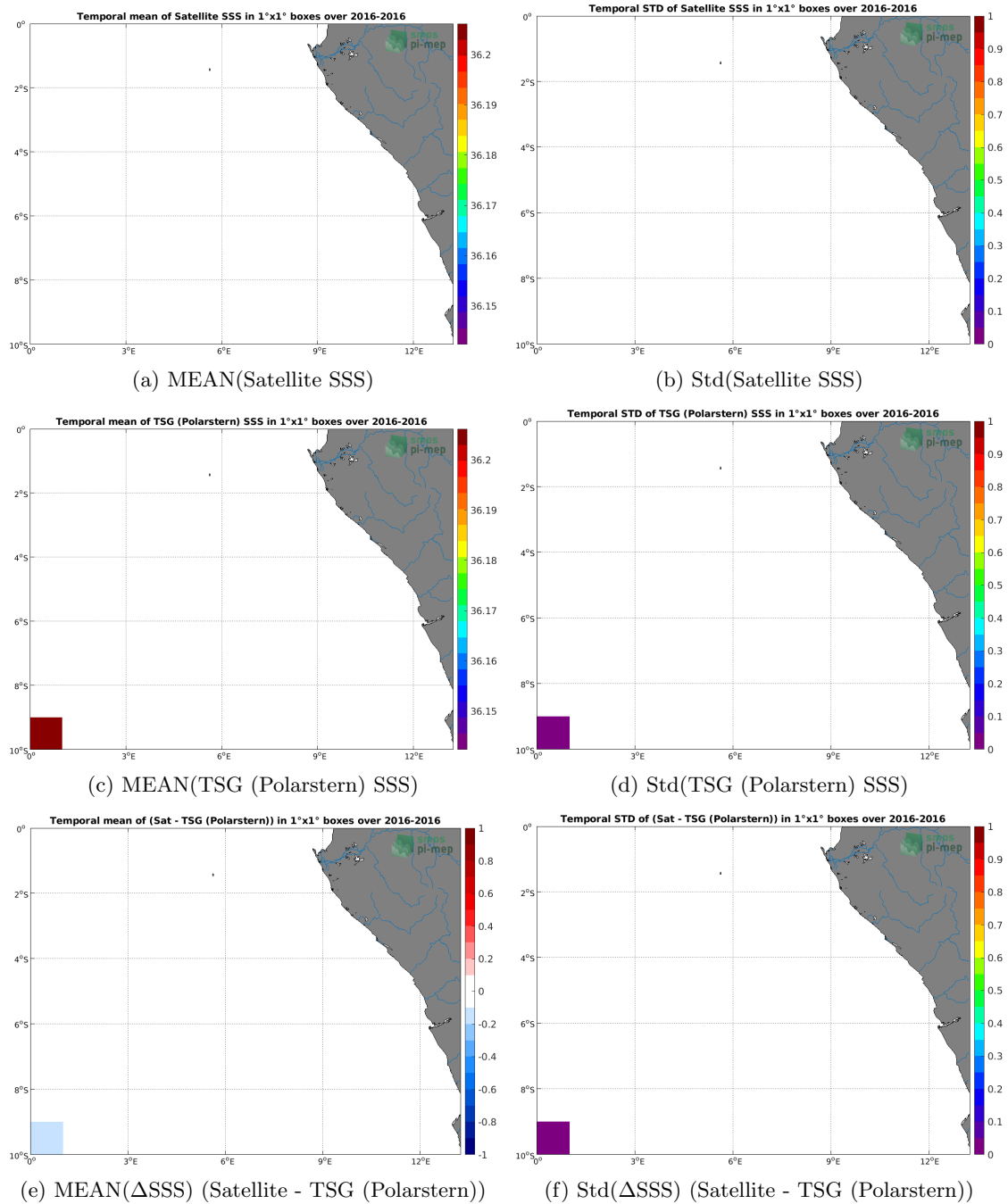
Figure 6: Temporal mean (left) and Std (right) of SSS from SMAP SSS L2 v4 (RSS) (top), TSG (Polarstern) (middle), and of \Delta SSS (Satellite - TSG (Polarstern)). Only match-up pairs are used to generate these maps.
