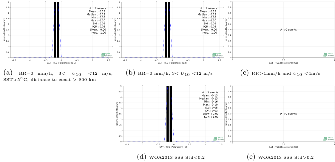
Figure 13: Normalized histogram of \Delta\text{SSS} (SMAP SSS L2 v4 (RSS) - TSG (Polarstern)) for 5 different subdatasets corresponding to: RR=0 mm/h, 3 < U_{10} < 12 m/s, SST > 5^\circ\text{C} , distance to coast > 800 km (a), RR=0 mm/h, 3 < U_{10} < 12 m/s (b), RR > 1\text{mm/h} and U_{10} < 4\text{m/s} (c), WOA2013 SSS Std < 0.2 (d), WOA2013 SSS Std > 0.2 (e).
