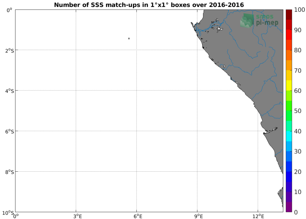
Figure 4: Number of SSS match-ups between TSG (Polarstern) SSS and the SMAP SSS L2 v4 (RSS) SSS product for the Congo river plume Pi-MEP region over 1^\circ \times 1^\circ boxes and for the full satellite product period.
