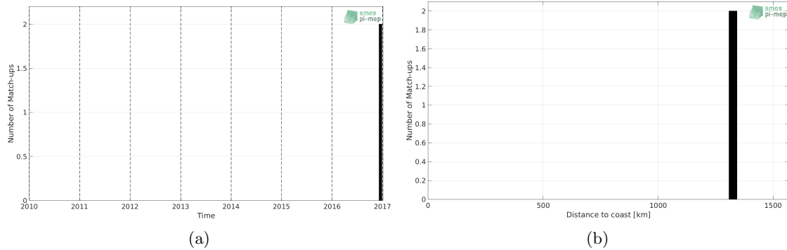
Figure 1: Number of match-ups between TSG (Polarstern) and SMAP SSS L2 v4 (RSS) SSS as a function of time (a) and as function of the distance to coast (b) over the Congo river plume Pi-MEP region and for the full satellite product period.
