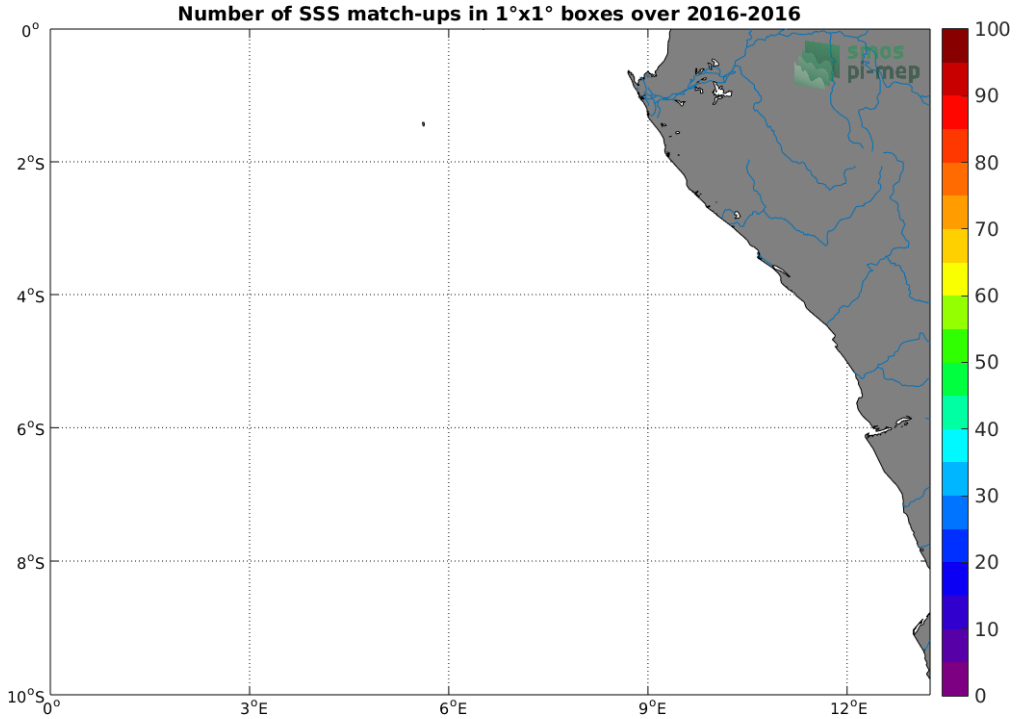
Figure 4: Number of SSS match-ups between TSG (Polarstern) SSS and the SMAP SSS L2 v4 (RSS) SSS product for the Congo river plume Pi-MEP region over 1°x1° boxes and for the full satellite product period.
