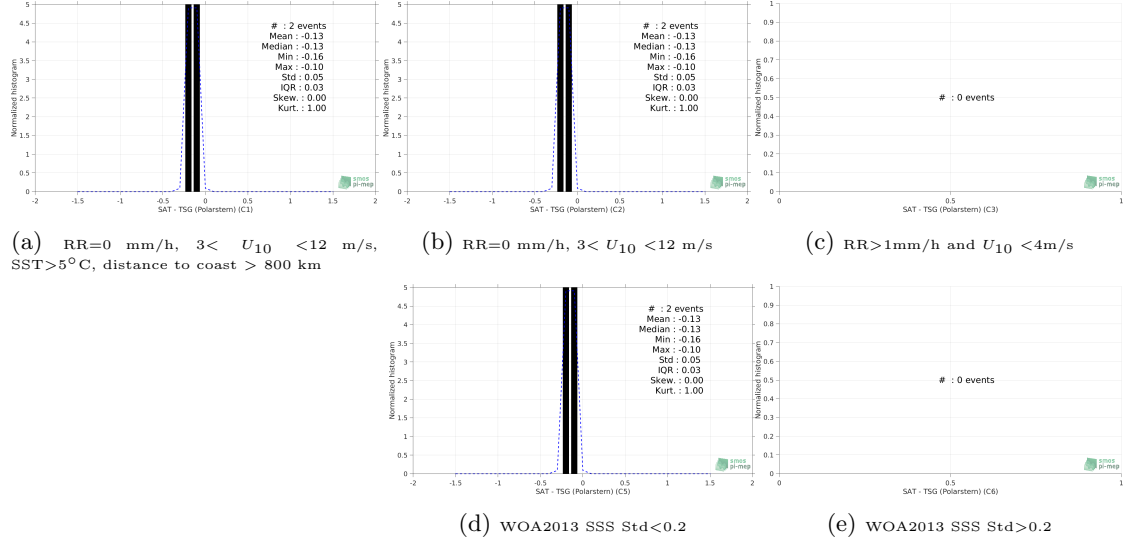
Figure 13: Normalized histogram of \Delta\text{SSS} (SMAP SSS L2 v4 (RSS) - TSG (Polarstern)) for 5 different subdatasets corresponding to: RR=0 mm/h, 3 < U_{10} < 12 m/s, SST > 5^\circ\text{C} , distance to coast > 800 km (a), RR=0 mm/h, 3 < U_{10} < 12 m/s (b), RR > 1\text{mm/h} and U_{10} < 4\text{m/s} (c), WOA2013 SSS Std < 0.2 (d), WOA2013 SSS Std > 0.2 (e).
