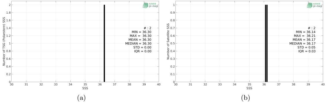
Figure 2: Histograms of SSS from TSG (Polarstern) (a) and SMAP SSS L2 v4 (RSS) (b) considering all match-up pairs per bins of 0.1 over the Congo river plume Pi-MEP region and for the full satellite product period.
