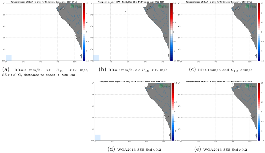
Figure 12: Temporal mean gridded over spatial boxes of size 1^{\circ}\times 1^{\circ} of \Delta\text{SSS} (SMAP SSS L2 v4 (RSS) - TSG (Polarstern)) for 5 different subdatasets corresponding to:RR=0 mm/h, 3 < U_{10} < 12 m/s, SST >5^{\circ}\text{C} , distance to coast > 800 km (a), RR=0 mm/h, 3 < U_{10} < 12 m/s (b), RR >1 mm/h and U_{10} < 4 m/s (c), WOA2013 SSS Std <0.2 (d), WOA2013 SSS Std >0.2 (e).
