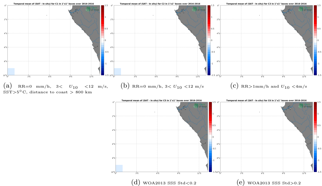
Figure 12: Temporal mean gridded over spatial boxes of size 1^{\circ}\times 1^{\circ} of \Delta\text{SSS} (SMAP-L2-RSS-V4 - TSG-POLARSTERN) for 5 different subdatasets corresponding to:RR=0 mm/h, 3 < U_{10} < 12 m/s, SST >5^{\circ}\text{C} , distance to coast > 800 km (a), RR=0 mm/h, 3 < U_{10} < 12 m/s (b), RR >1 mm/h and U_{10} < 4 m/s (c), WOA2013 SSS Std <0.2 (d), WOA2013 SSS Std >0.2 (e).
