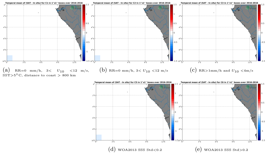
Figure 12: Temporal mean gridded over spatial boxes of size 1^\circ \times 1^\circ of \Delta SSS (SMAP-L2-RSS-V4 - TSG-POLARSTERN) for 5 different subdatasets corresponding to: RR=0 mm/h, 3 < U_{10} < 12 m/s, SST > 5^\circ\text{C} , distance to coast > 800 km (a), RR=0 mm/h, 3 < U_{10} < 12 m/s (b), RR > 1 mm/h and U_{10} < 4 m/s (c), WOA2013 SSS Std < 0.2 (d), WOA2013 SSS Std > 0.2 (e).
