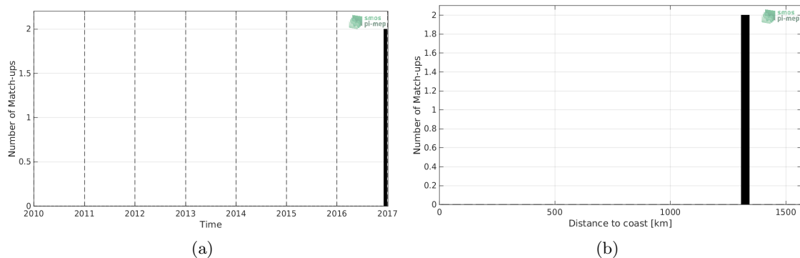
Figure 1: Number of match-ups between TSG-POLARSTERN and SMAP-L2-RSS-V4 SSS as a function of time (a) and as function of the distance to coast (b) over the Congo river plume Pi-MEP region and for the full satellite product period.
