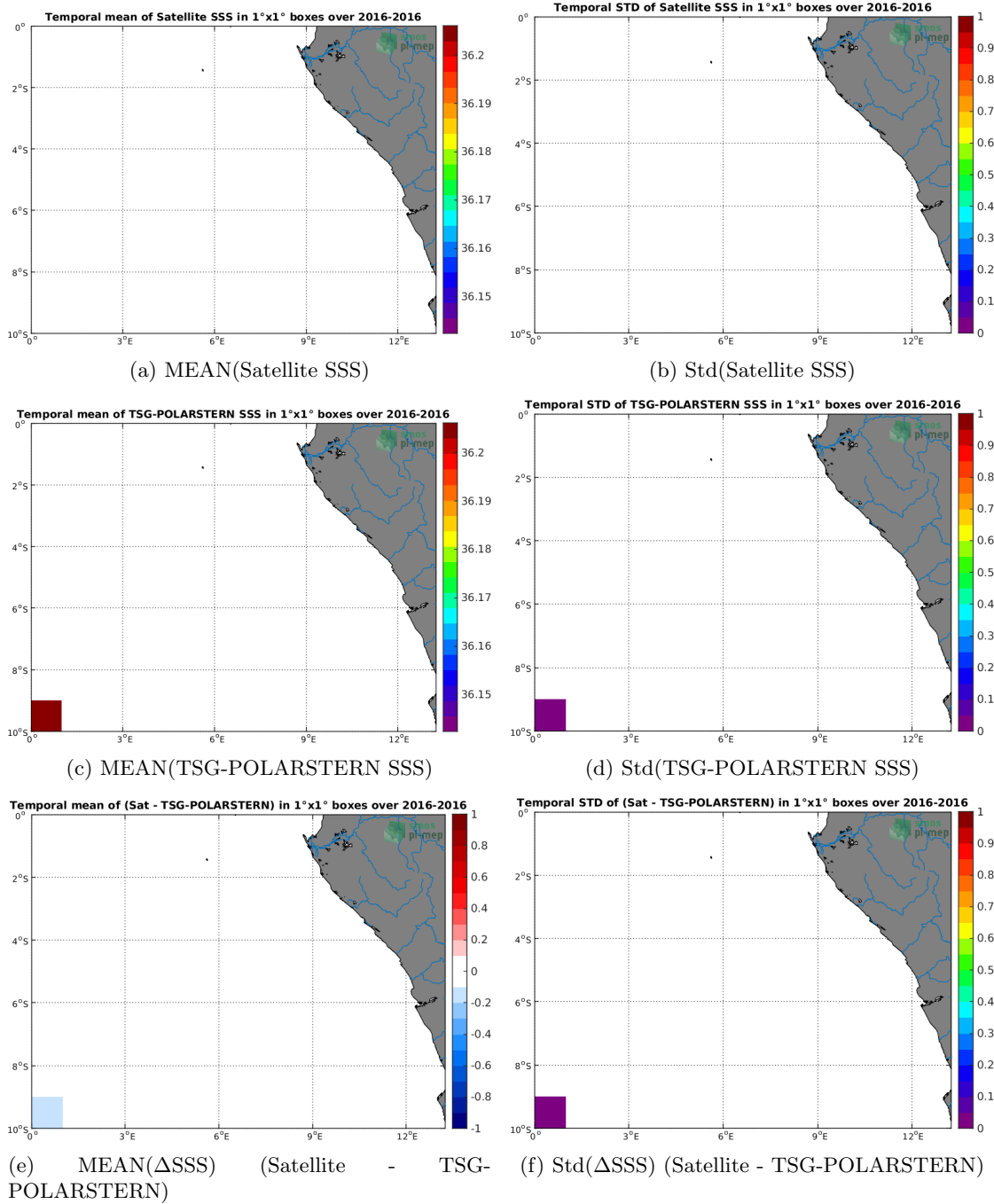
Figure 6: Temporal mean (left) and Std (right) of SSS from SMAP-L2-RSS-V4 (top), TSG-POLARSTERN (middle), and of \Delta SSS (Satellite - TSG-POLARSTERN). Only match-up pairs are used to generate these maps.
