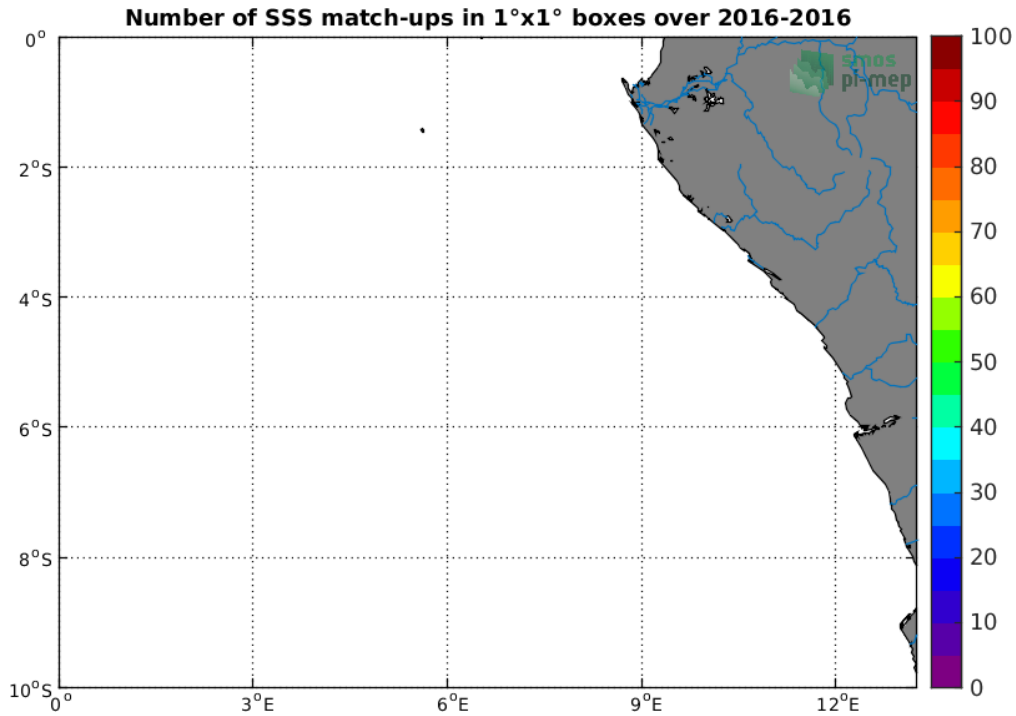
Figure 4: Number of SSS match-ups between TSG-POLARSTERN SSS and the SMAP-L2-RSS-V4 SSS product for the Congo river plume Pi-MEP region over 1°x1° boxes and for the full satellite product period.
