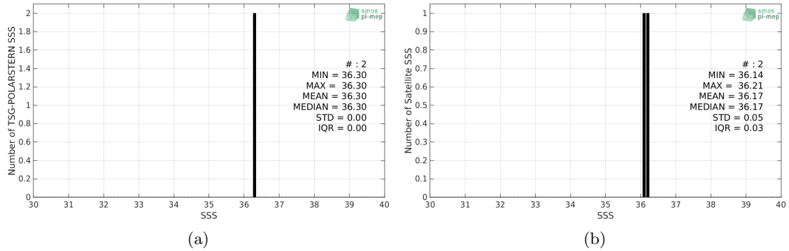
Figure 2: Histograms of SSS from TSG-POLARSTERN (a) and SMAP-L2-RSS-V4 (b) considering all match-up pairs per bins of 0.1 over the Congo river plume Pi-MEP region and for the full satellite product period.
