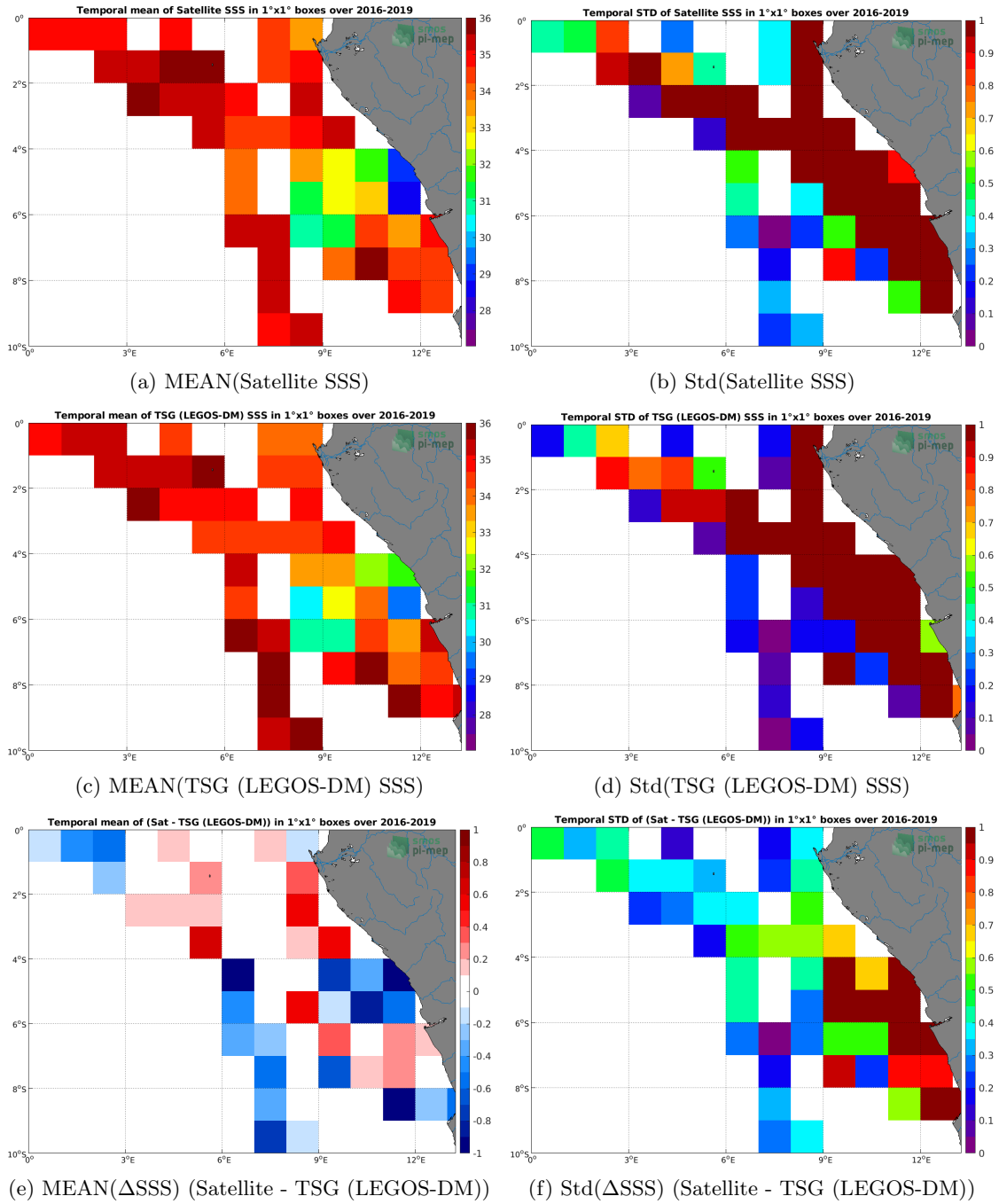
Figure 6: Temporal mean (left) and Std (right) of SSS from SMAP SSS L2 v4 (RSS) (top), TSG (LEGOS-DM) (middle), and of \Delta SSS (Satellite - TSG (LEGOS-DM)). Only match-up pairs are used to generate these maps.
