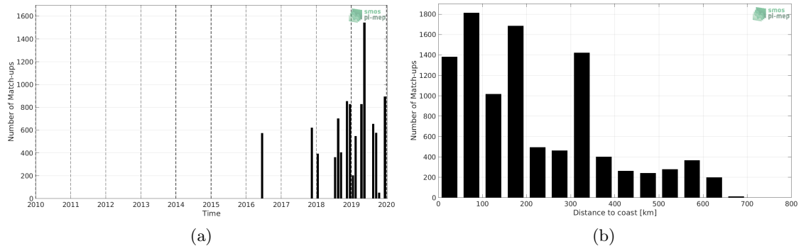
Figure 1: Number of match-ups between TSG (LEGOS-DM) and SMAP SSS L2 v4 (RSS) SSS as a function of time (a) and as function of the distance to coast (b) over the Congo river plume Pi-MEP region and for the full satellite product period.
