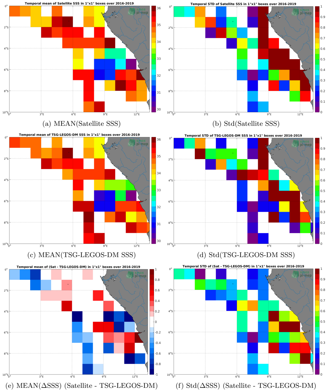
Figure 6: Temporal mean (left) and Std (right) of SSS from SMAP-L2-RSS-V4 (top), TSG-LEGOS-DM (middle), and of \Delta SSS (Satellite - TSG-LEGOS-DM). Only match-up pairs are used to generate these maps.
