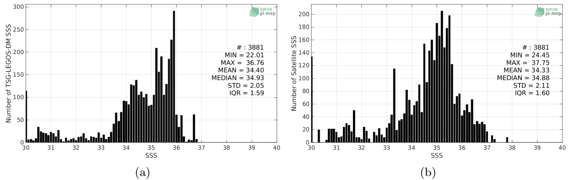
Figure 2: Histograms of SSS from TSG-LEGOS-DM (a) and SMAP-L2-RSS-V4 (b) considering all match-up pairs per bins of 0.1 over the Congo river plume Pi-MEP region and for the full satellite product period.
