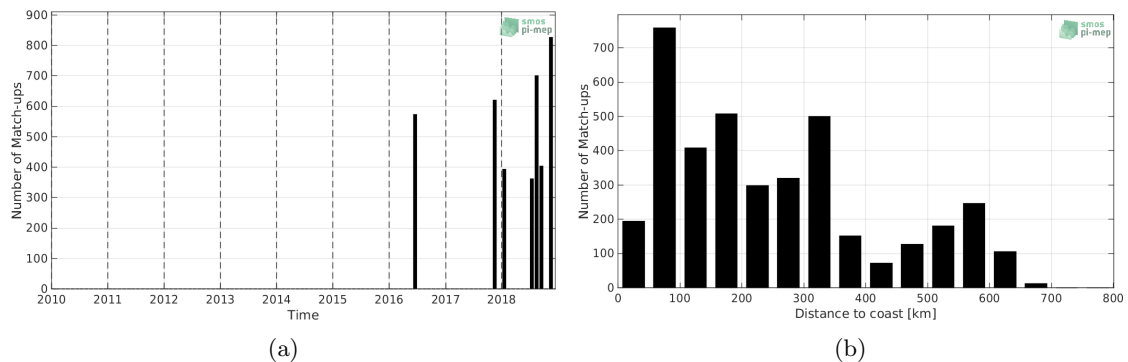
Figure 1: Number of match-ups between TSG-LEGOS-DM and SMAP-L2-RSS-V4 SSS as a function of time (a) and as function of the distance to coast (b) over the Congo river plume Pi-MEP region and for the full satellite product period.
