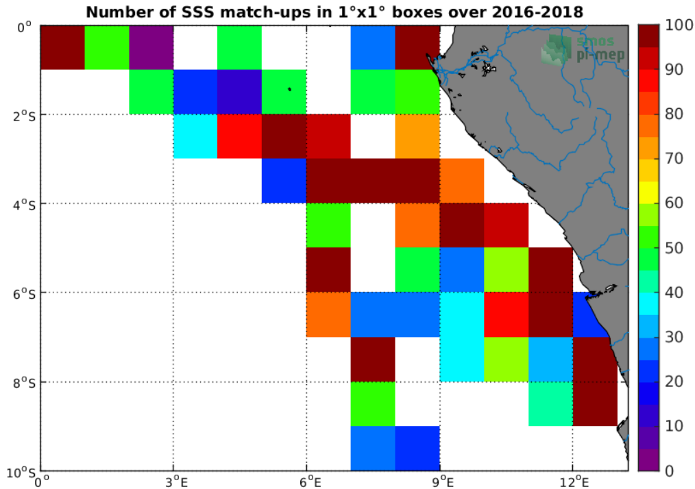
Figure 4: Number of SSS match-ups between TSG-LEGOS-DM SSS and the SMAP-L2-RSS-V4 SSS product for the Congo river plume Pi-MEP region over 1°x1° boxes and for the full satellite product period.
