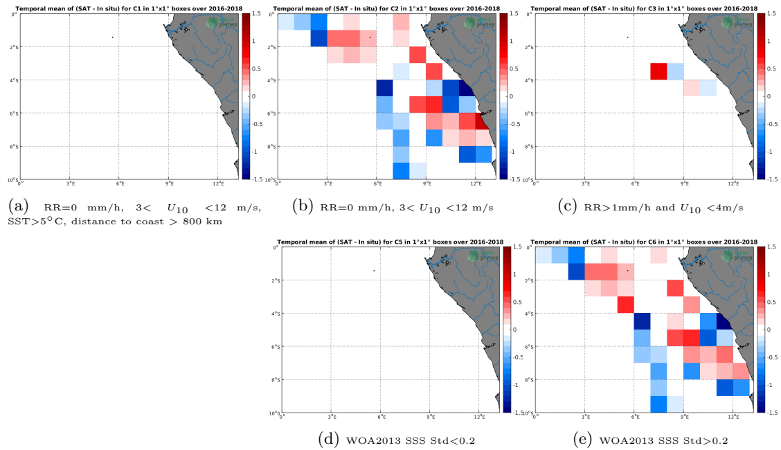
Figure 12: Temporal mean gridded over spatial boxes of size 1^\circ \times 1^\circ of \Delta SSS (SMAP-L2-RSS-V4 - TSG-LEGOS-DM) for 5 different subdatasets corresponding to:RR=0 mm/h, 3 < U_{10} < 12 m/s, SST >5^\circ C, distance to coast > 800 km (a), RR=0 mm/h, 3 < U_{10} < 12 m/s (b), RR >1 mm/h and U_{10} < 4 m/s (c), WOA2013 SSS Std <0.2 (d), WOA2013 SSS Std >0.2 (e).
