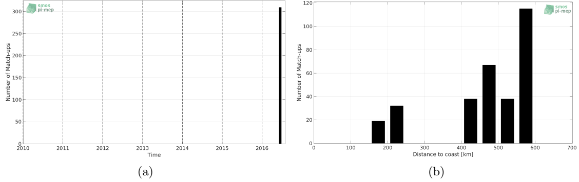
Figure 1: Number of match-ups between TSG-LEGOS-DM and SMAP-L2-RSS-V3-70KM SSS as a function of time (a) and as function of the distance to coast (b) over the Congo river plume Pi-MEP region and for the full satellite product period.
