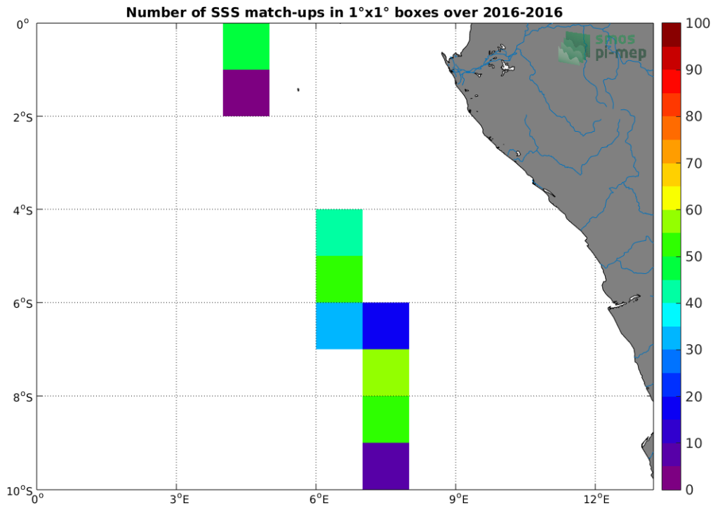
Figure 4: Number of SSS match-ups between TSG-LEGOS-DM SSS and the SMAP-L2-RSS-V3-70KM SSS product for the Congo river plume Pi-MEP region over 1^\circ \times 1^\circ boxes and for the full satellite product period.
