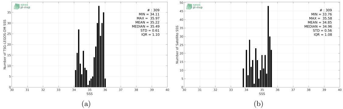
Figure 2: Histograms of SSS from TSG-LEGOS-DM (a) and SMAP-L2-RSS-V3-70KM (b) considering all match-up pairs per bins of 0.1 over the Congo river plume Pi-MEP region and for the full satellite product period.
