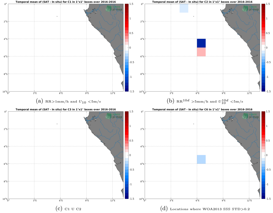
Figure 12: Temporal mean gridded over spatial boxes of size 1^\circ \times 1^\circ of \Delta SSS (SMAP-L2-RSS-V3-70KM - TSG-LEGOS-DM) for 4 different subdatasets corresponding to: RR > 1\text{mm/h} and U_{10} < 5\text{m/s} (a), RR^{10d} > 5\text{mm/h} and U_{10}^{10d} < 5\text{m/s} (b), C1 \cup C2 (c), Locations where WOA2013 SSS STD > 0.2 (d).
