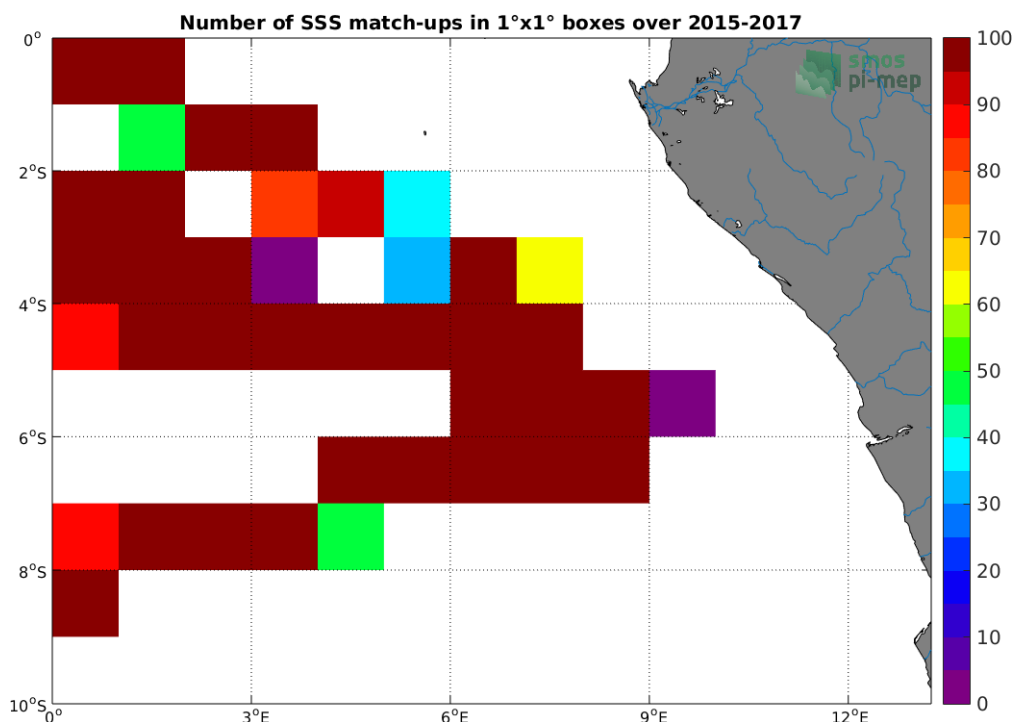
Figure 4: Number of SSS match-ups between TSG-GOSUD-Research-vessel SSS and the SMAP-L2-RSS-V3-70KM SSS product for the Congo river plume Pi-MEP region over 1°x1° boxes and for the full satellite product period.
