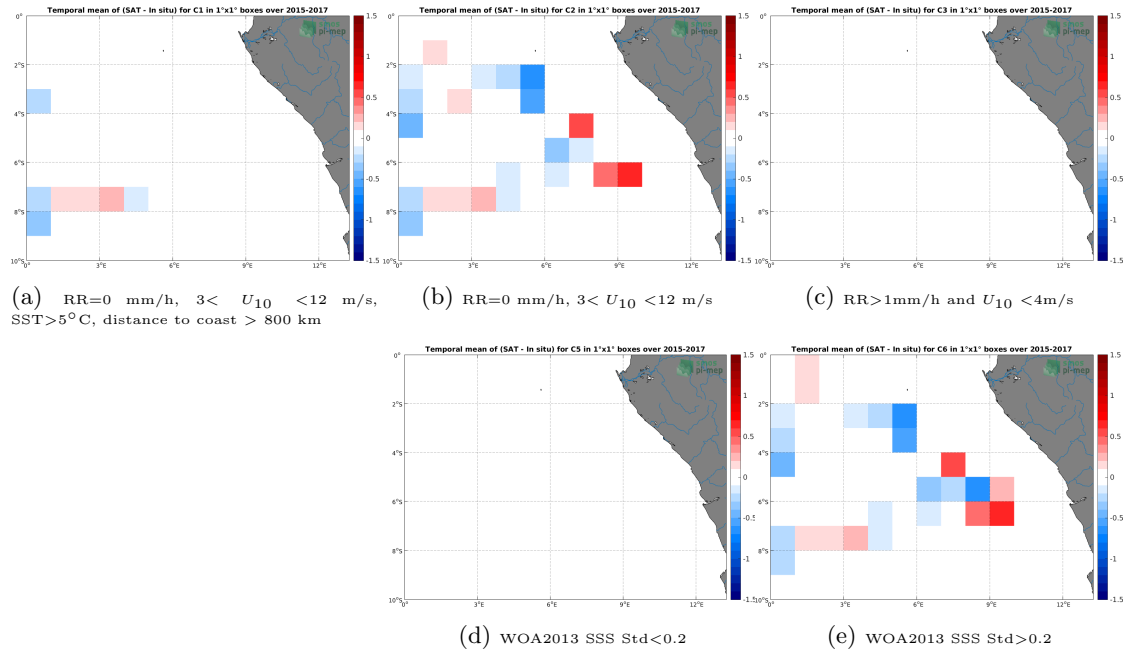
Figure 12: Temporal mean gridded over spatial boxes of size 1^\circ \times 1^\circ of \Delta SSS (SMAP-L2-RSS-V3-70KM - TSG-GOSUD-Research-vessel) for 5 different subdatasets corresponding to:RR=0 mm/h, 3 < U_{10} < 12 m/s, SST > 5^\circ\text{C} , distance to coast > 800 km (a), RR=0 mm/h, 3 < U_{10} < 12 m/s (b), RR > 1 mm/h and U_{10} < 4 m/s (c), WOA2013 SSS Std < 0.2 (d), WOA2013 SSS Std > 0.2 (e).
