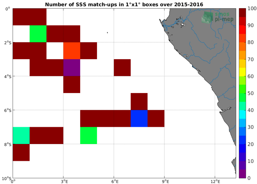
Figure 4: Number of SSS match-ups between TSG-GOSUD-Research-vessel SSS and the SMAP-L2-RSS-V3-70KM SSS product for the Congo river plume Pi-MEP region over 1^{\circ} \times 1^{\circ} boxes and for the full satellite product period.
