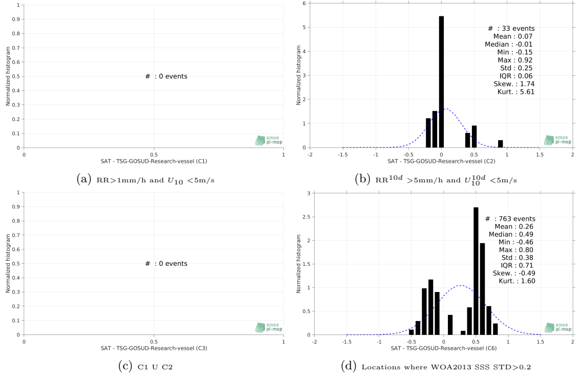
Figure 13: Normalized histogram of \Delta\text{SSS} (SMAP-L2-RSS-V3-70KM - TSG-GOSUD-Research-vessel) for 6 different subdatasets corresponding to: RR > 1\text{mm/h} and U_{10} < 5\text{m/s} (a), RR^{10d} > 5\text{mm/h} and U_{10}^{10d} < 5\text{m/s} (b), C1 \cup C2 (c), Locations where WOA2013 SSS STD > 0.2 (d).
