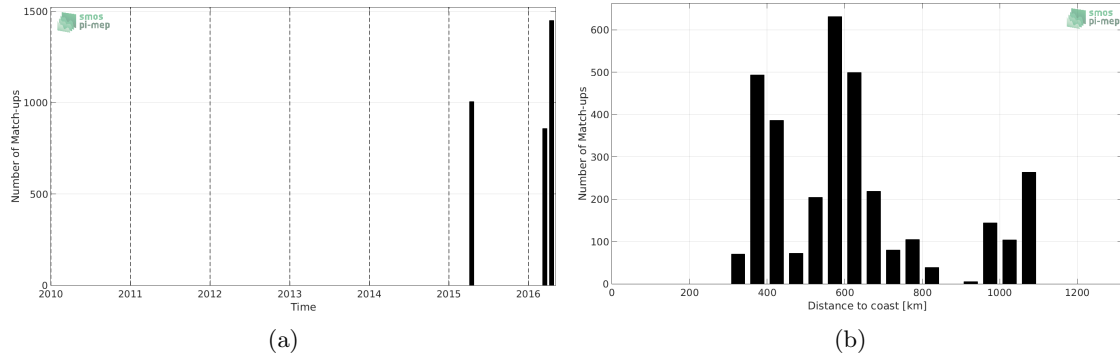
Figure 1: Number of match-ups between TSG-GOSUD-Research-vessel and SMAP-L2-RSS-V3-70KM SSS as a function of time (a) and as function of the distance to coast (b) over the Congo river plume Pi-MEP region and for the full satellite product period.
