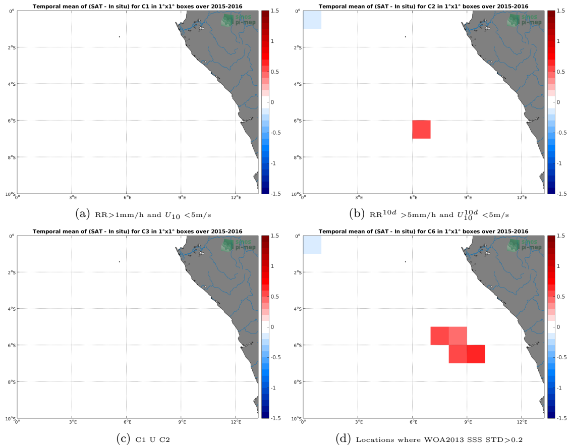
Figure 12: Temporal mean gridded over spatial boxes of size 1^\circ \times 1^\circ of \Delta SSS (SMAP-L2-RSS-V3-70KM - TSG-GOSUD-Research-vessel) for 4 different subdatasets corresponding to: RR > 1\text{mm/h} and U_{10} < 5\text{m/s} (a), RR^{10d} > 5\text{mm/h} and U_{10}^{10d} < 5\text{m/s} (b), C1 \cup C2 (c), Locations where WOA2013 SSS STD > 0.2 (d).
