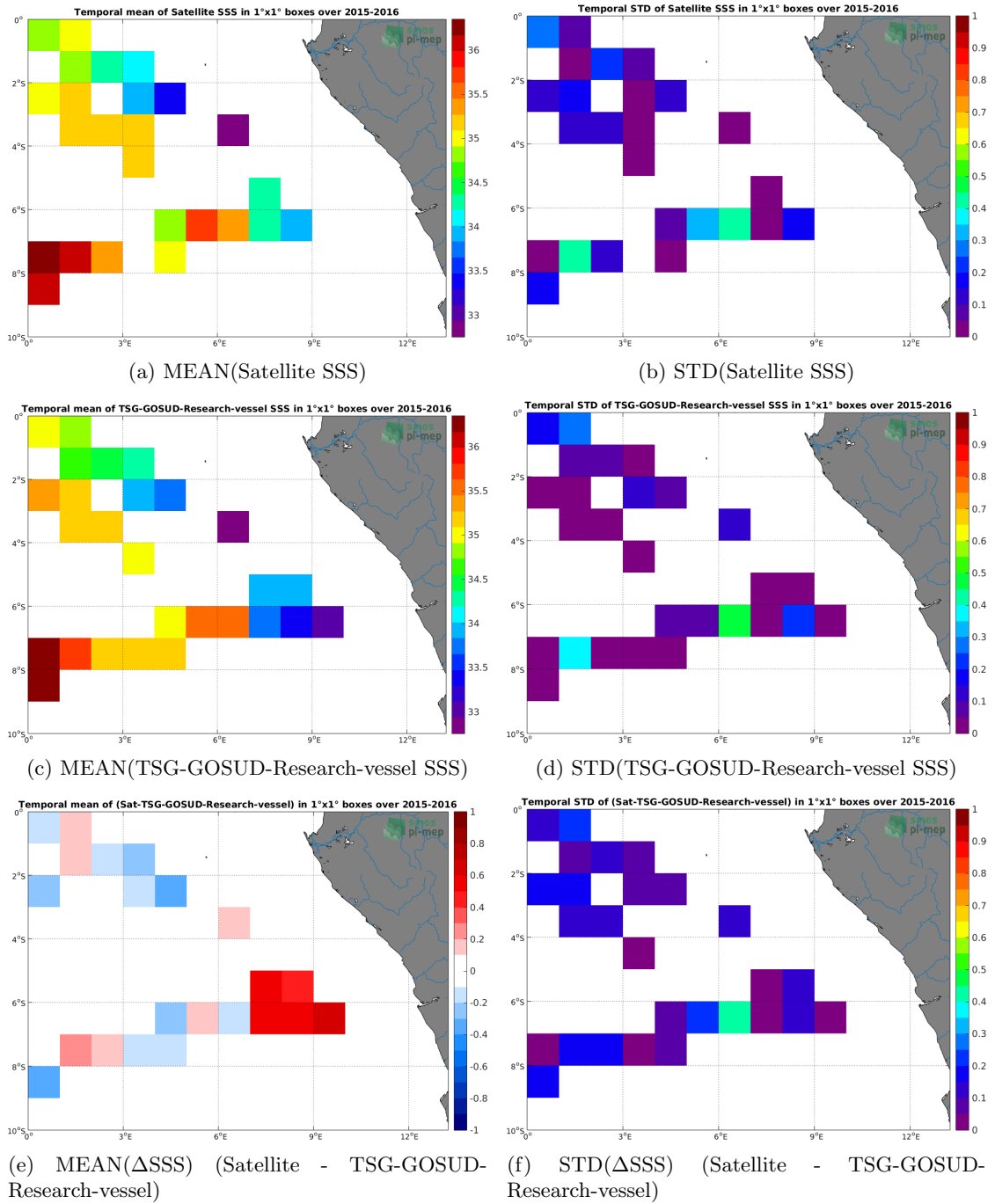
Figure 6: Temporal mean (left) and STD (right) of SSS from SMAP-L2-RSS-V3-70KM (top), TSG-GOSUD-Research-vessel (middle), and of \Delta SSS (Satellite - TSG-GOSUD-Research-vessel). Only match-up pairs are used to generate these maps.
