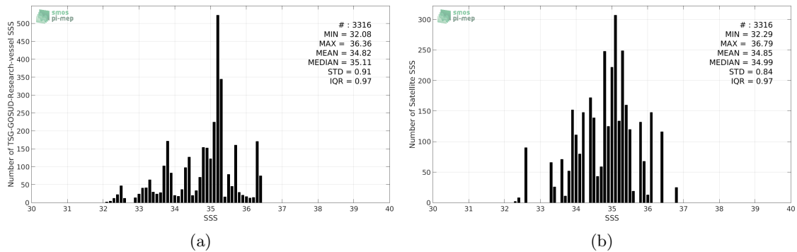
Figure 2: Histograms of SSS from TSG-GOSUD-Research-vessel (a) and SMAP-L2-RSS-V3-70KM (b) considering all match-up pairs per bins of 0.1 over the Congo river plume Pi-MEP region and for the full satellite product period.
