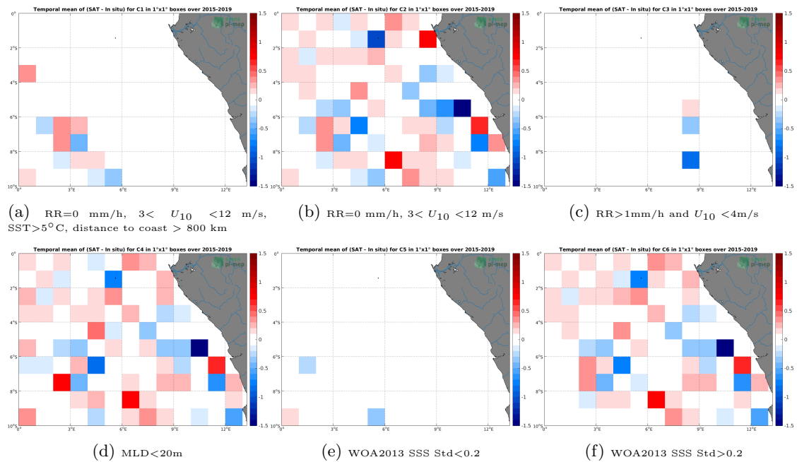
Figure 12: Temporal mean gridded over spatial boxes of size 1^\circ \times 1^\circ of \Delta SSS (SMAP-L2-RSS-V3-70KM - Argo) for 6 different subdatasets corresponding to:RR=0 mm/h, 3 < U_{10} < 12 m/s, SST >5^\circ C, distance to coast > 800 km (a), RR=0 mm/h, 3 < U_{10} < 12 m/s (b), RR >1 mm/h and U_{10} < 4 m/s (c),MLD <20 m (d),WOA2013 SSS Std <0.2 (e),WOA2013 SSS Std >0.2 (f).
