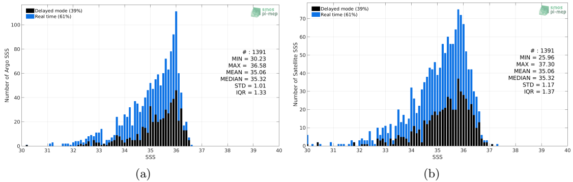
Figure 2: Histograms of SSS from Argo (a) and SMAP-L2-RSS-V3-70KM (b) considering all match-up pairs per bins of 0.1 over the Congo river plume Pi-MEP region and for the full satellite product period.
