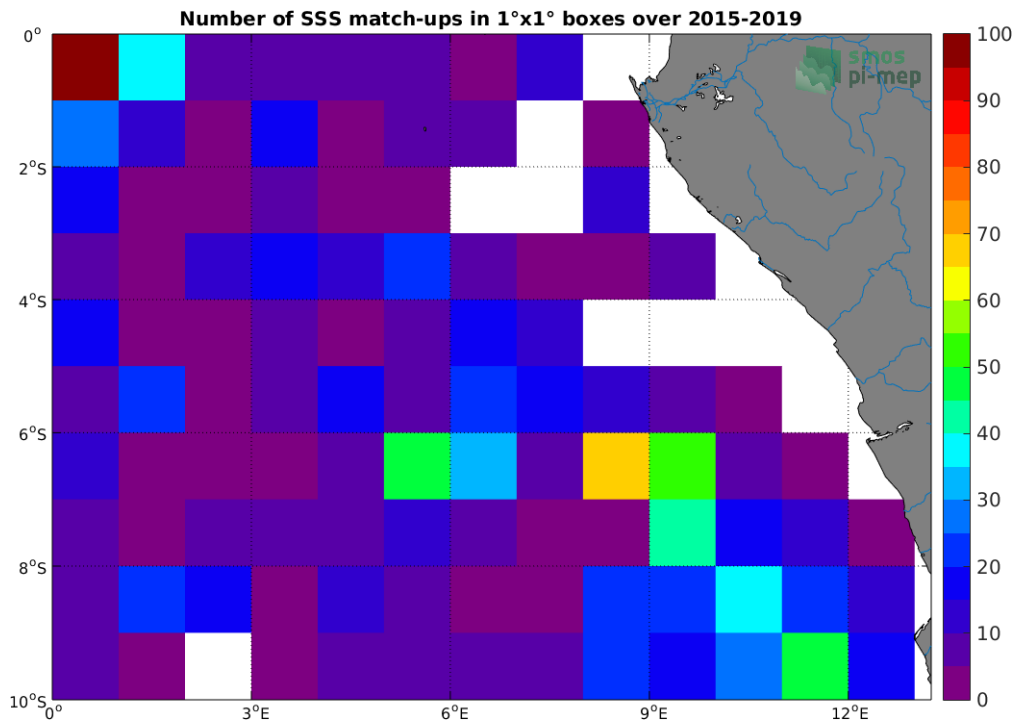
Figure 4: Number of SSS match-ups between Argo SSS and the SMAP-L2-RSS-V3-70KM SSS product for the Congo river plume Pi-MEP region over 1°x1° boxes and for the full satellite product period.
