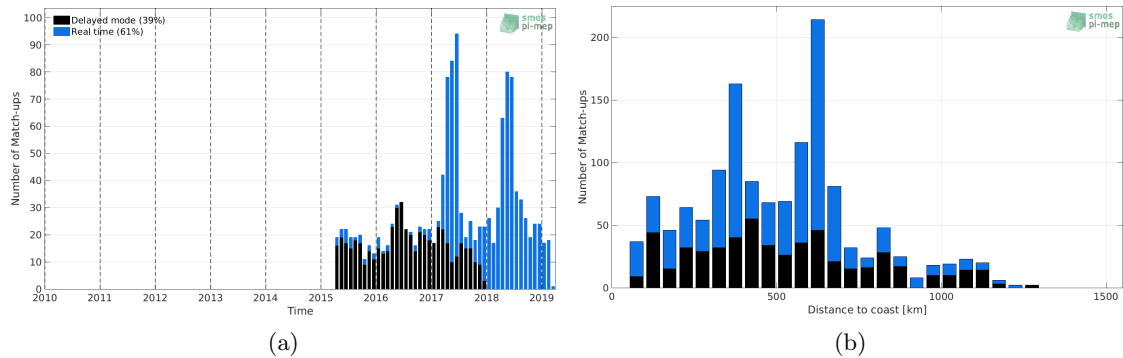
Figure 1: Number of match-ups between Argo and SMAP-L2-RSS-V3-70KM SSS as a function of time (a) and as function of the distance to coast (b) over the Congo river plume Pi-MEP region and for the full satellite product period.
