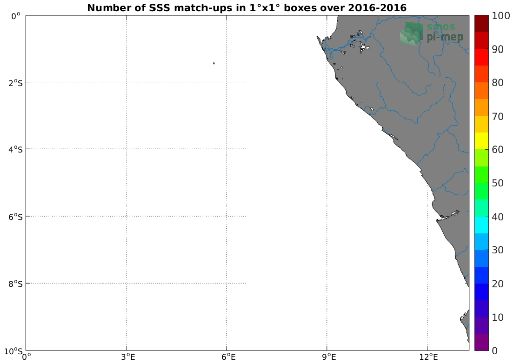
Figure 4: Number of SSS match-ups between TSG (Polarstern) SSS and the SMAP SSS L2 v5.0 (JPL) SSS product for the Congo river plume Pi-MEP region over 1°×1° boxes and for the full satellite product period.
