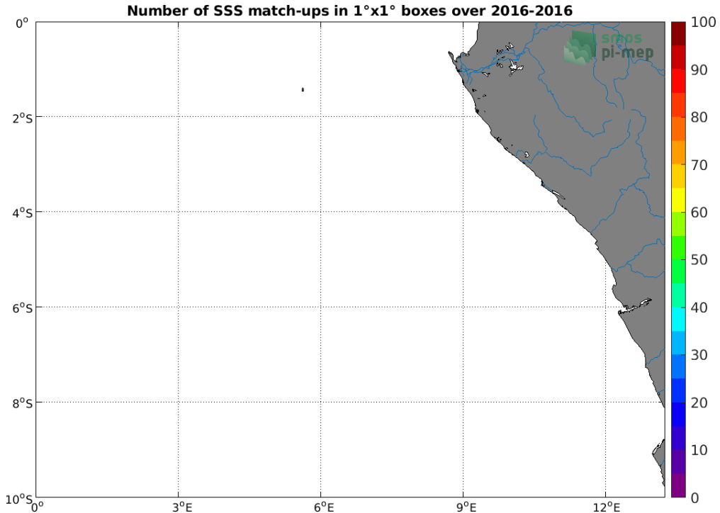
Figure 4: Number of SSS match-ups between TSG (Polarstern) SSS and the SMAP SSS L2 v5.0 (JPL) SSS product for the Congo river plume Pi-MEP region over 1°x1° boxes and for the full satellite product period.
