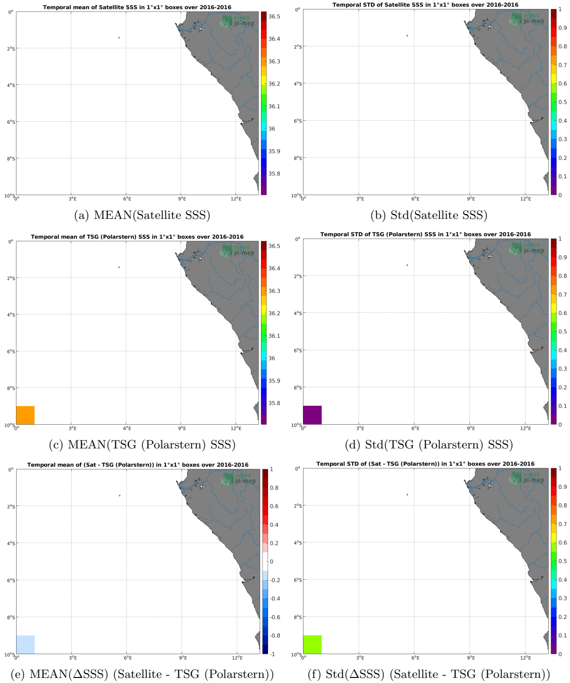
Figure 6: Temporal mean (left) and Std (right) of SSS from SMAP SSS L2 v5.0 (JPL) (top), TSG (Polarstern) (middle), and of \Delta SSS (Satellite - TSG (Polarstern)). Only match-up pairs are used to generate these maps.
