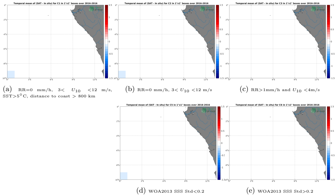
Figure 12: Temporal mean gridded over spatial boxes of size 1^{\circ}\times 1^{\circ} of \Delta\text{SSS} (SMAP SSS L2 v5.0 (JPL) - TSG (Polarstern)) for 5 different subdatasets corresponding to:RR=0 mm/h, 3 < U_{10} < 12 m/s, SST > 5^{\circ}\text{C} , distance to coast > 800 km (a), RR=0 mm/h, 3 < U_{10} < 12 m/s (b), RR > 1 mm/h and U_{10} < 4 m/s (c), WOA2013 SSS Std < 0.2 (d), WOA2013 SSS Std > 0.2 (e).
