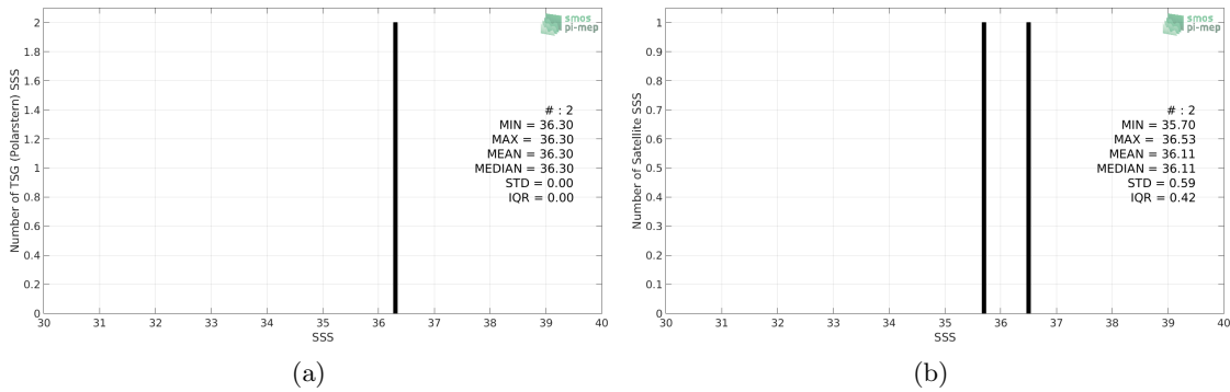
Figure 2: Histograms of SSS from TSG (Polarstern) (a) and SMAP SSS L2 v5.0 (JPL) (b) considering all match-up pairs per bins of 0.1 over the Congo river plume Pi-MEP region and for the full satellite product period.
