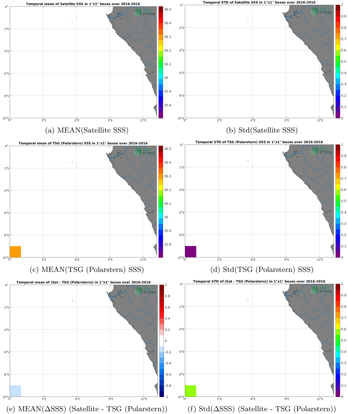
Figure 6: Temporal mean (left) and Std (right) of SSS from SMAP SSS L2 v5.0 (JPL) (top), TSG (Polarstern) (middle), and of \Delta SSS (Satellite - TSG (Polarstern)). Only match-up pairs are used to generate these maps.
