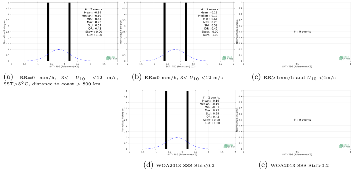
Figure 13: Normalized histogram of \Delta SSS (SMAP SSS L2 v5.0 (JPL) - TSG (Polarstern)) for 5 different subdatasets corresponding to: RR=0 mm/h, 3 < U_{10} < 12 m/s, SST>5°C, distance to coast > 800 km (a), RR=0 mm/h, 3 < U_{10} < 12 m/s (b), RR>1mm/h and U_{10} < 4 m/s (c), WOA2013 SSS Std<0.2 (d), WOA2013 SSS Std>0.2 (e).
