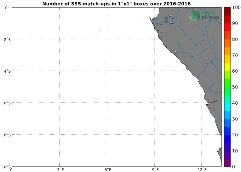
Figure 4: Number of SSS match-ups between TSG (Polarstern) SSS and the SMAP SSS L2 v5.0 (JPL) SSS product for the Congo river plume Pi-MEP region over 1^\circ \times 1^\circ boxes and for the full satellite product period.
