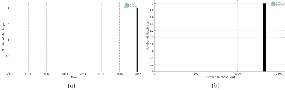
Figure 1: Number of match-ups between TSG (Polarstern) and SMAP SSS L2 v5.0 (JPL) SSS as a function of time (a) and as function of the distance to coast (b) over the Congo river plume Pi-MEP region and for the full satellite product period.
