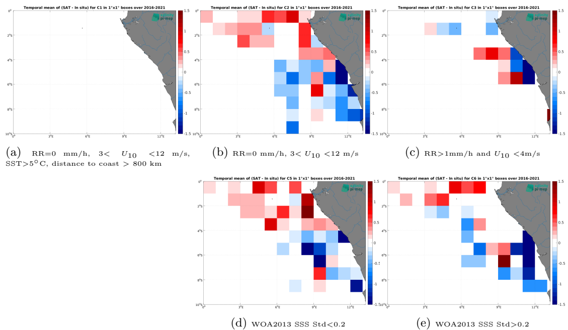
Figure 14: Temporal mean gridded over spatial boxes of size 1^\circ \times 1^\circ of \Delta SSS (SMAP SSS L2 v5.0 (JPL) - TSG (LEGOS-DM)) for 5 different subdatasets corresponding to: RR=0 mm/h, 3 < U_{10} < 12 m/s, SST > 5°C, distance to coast > 800 km (a), RR=0 mm/h, 3 < U_{10} < 12 m/s (b), RR > 1mm/h and U_{10} < 4 m/s (c), WOA2013 SSS Std < 0.2 (d), WOA2013 SSS Std > 0.2 (e).
