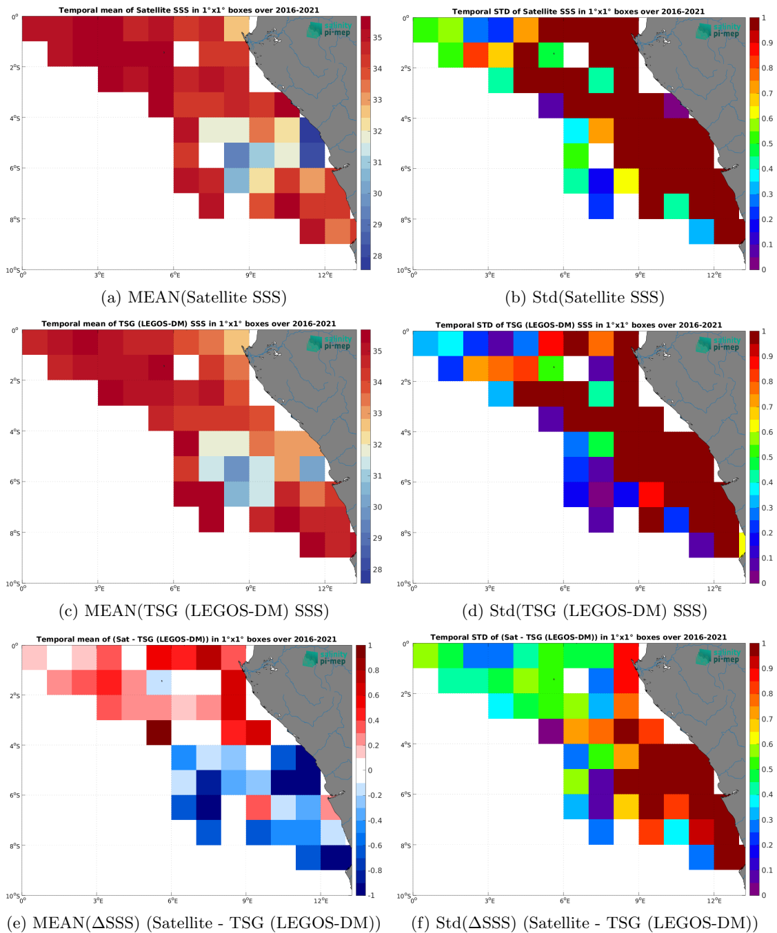
Figure 7: Temporal mean (left) and Std (right) of SSS from SMAP SSS L2 v5.0 (JPL) (top), TSG (LEGOS-DM) (middle), and of \Delta SSS (Satellite - TSG (LEGOS-DM)). Only match-up pairs are used to generate these maps.
