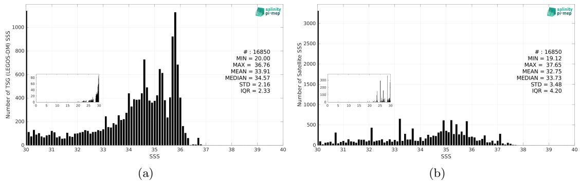
Figure 3: Histograms of SSS from TSG (LEGOS-DM) (a) and SMAP SSS L2 v5.0 (JPL) (b) considering all match-up pairs per bins of 0.1 over the Congo river plume Pi-MEP region and for the full satellite product period.
