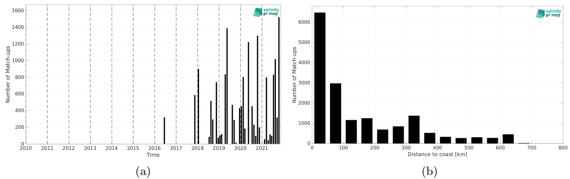
Figure 2: Number of match-ups between TSG (LEGOS-DM) and SMAP SSS L2 v5.0 (JPL) SSS as a function of time (a) and as function of the distance to coast (b) over the Congo river plume Pi-MEP region and for the full satellite product period.
