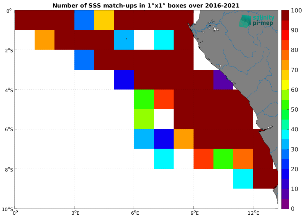
Figure 5: Number of SSS match-ups between TSG (LEGOS-DM) SSS and the SMAP SSS L2 v5.0 (JPL) SSS product for the Congo river plume Pi-MEP region over 1^\circ \times 1^\circ boxes and for the full satellite product period.
