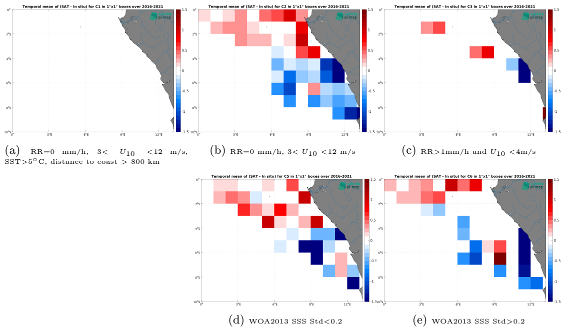
Figure 14: Temporal mean gridded over spatial boxes of size 1^\circ \times 1^\circ of \Delta SSS (SMAP SSS L2 v5.0 (JPL) - TSG (LEGOS-DM)) for 5 different subdatasets corresponding to:RR=0 mm/h, 3 < U_{10} < 12 m/s, SST>5°C, distance to coast > 800 km (a), RR=0 mm/h, 3 < U_{10} < 12 m/s (b), RR>1mm/h and U_{10} < 4 m/s (c), WOA2013 SSS Std<0.2 (d), WOA2013 SSS Std>0.2 (e).
