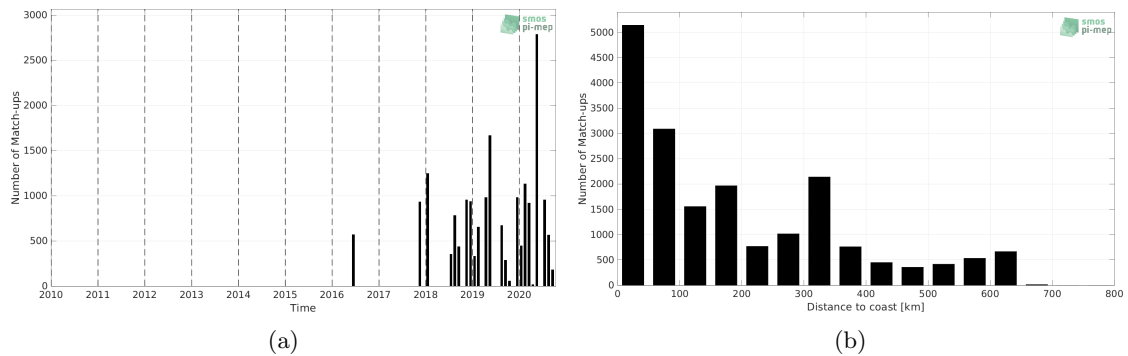
Figure 1: Number of match-ups between TSG (LEGOS-DM) and SMAP SSS L2 v5.0 (JPL) SSS as a function of time (a) and as function of the distance to coast (b) over the Congo river plume Pi-MEP region and for the full satellite product period.
