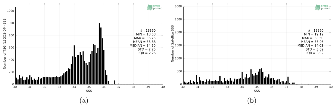
Figure 2: Histograms of SSS from TSG (LEGOS-DM) (a) and SMAP SSS L2 v5.0 (JPL) (b) considering all match-up pairs per bins of 0.1 over the Congo river plume Pi-MEP region and for the full satellite product period.
