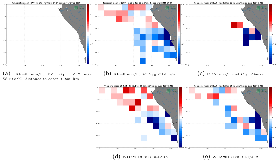
Figure 12: Temporal mean gridded over spatial boxes of size 1^\circ \times 1^\circ of \Delta SSS (SMAP SSS L2 v5.0 (JPL) - TSG (LEGOS-DM)) for 5 different subdatasets corresponding to:RR=0 mm/h, 3 < U_{10} < 12 m/s, SST > 5^\circ\text{C} , distance to coast > 800 km (a), RR=0 mm/h, 3 < U_{10} < 12 m/s (b), RR > 1 mm/h and U_{10} < 4 m/s (c), WOA2013 SSS Std < 0.2 (d), WOA2013 SSS Std > 0.2 (e).
