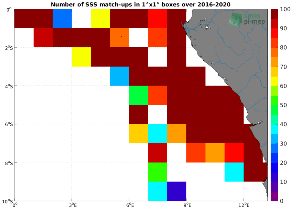
Figure 4: Number of SSS match-ups between TSG (LEGOS-DM) SSS and the SMAP SSS L2 v5.0 (JPL) SSS product for the Congo river plume Pi-MEP region over 1^{\circ} \times 1^{\circ} boxes and for the full satellite product period.
