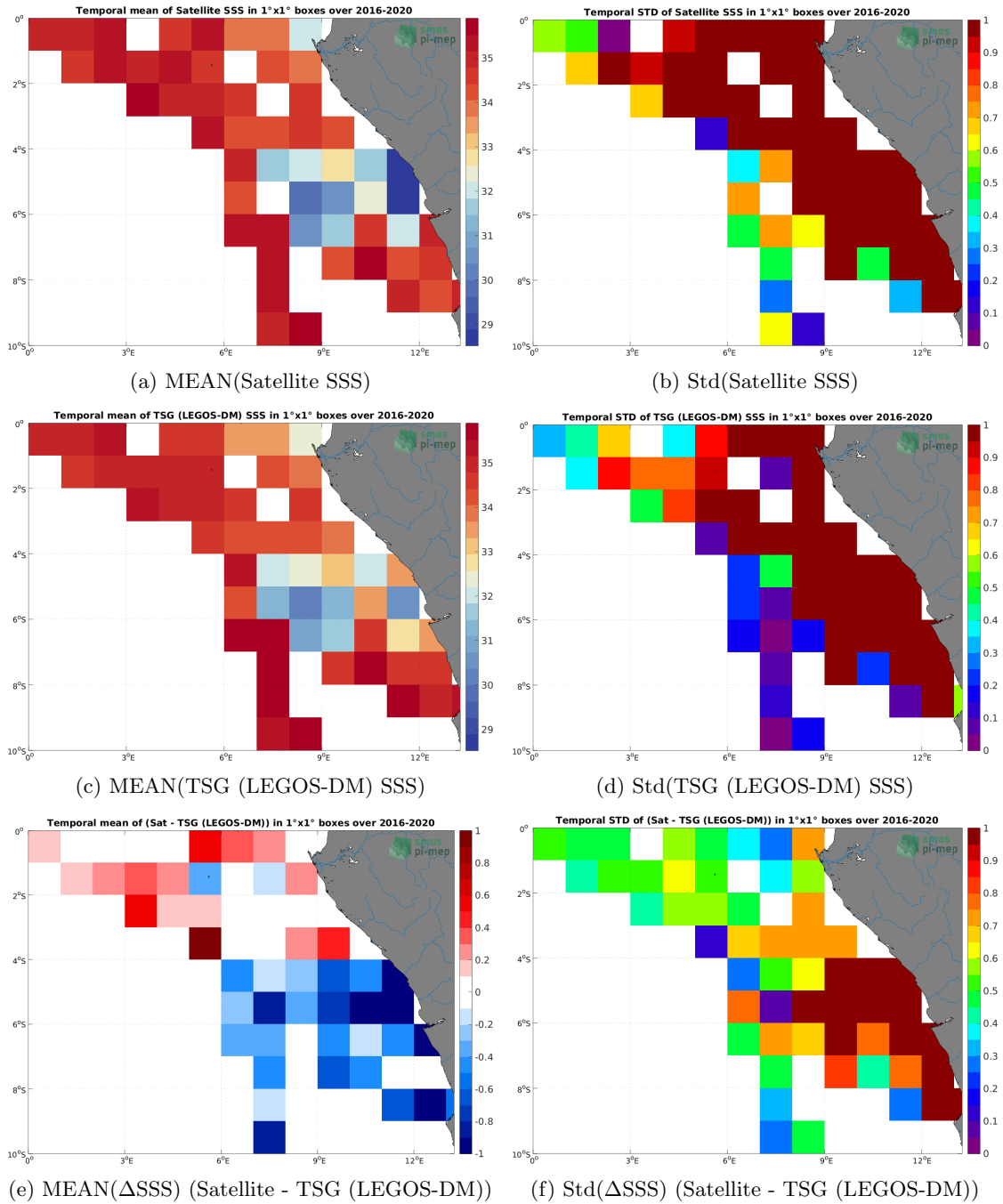
Figure 6: Temporal mean (left) and Std (right) of SSS from SMAP SSS L2 v5.0 (JPL) (top), TSG (LEGOS-DM) (middle), and of \Delta SSS (Satellite - TSG (LEGOS-DM)). Only match-up pairs are used to generate these maps.
