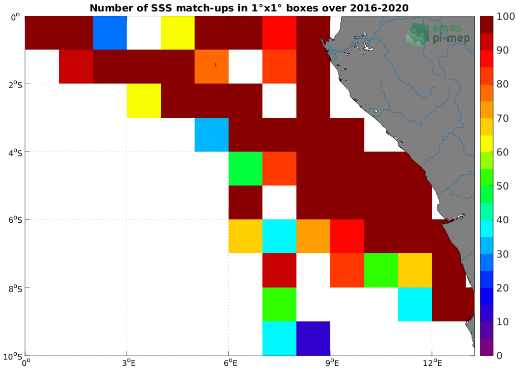
Figure 4: Number of SSS match-ups between TSG (LEGOS-DM) SSS and the SMAP SSS L2 v5.0 (JPL) SSS product for the Congo river plume Pi-MEP region over 1^\circ \times 1^\circ boxes and for the full satellite product period.
