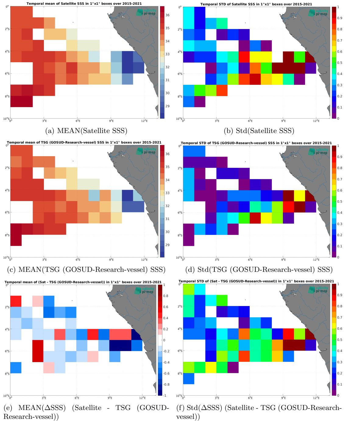
Figure 7: Temporal mean (left) and Std (right) of SSS from SMAP SSS L2 v5.0 (JPL) (top), TSG (GOSUD-Research-vessel) (middle), and of \Delta SSS (Satellite - TSG (GOSUD-Research-vessel)). Only match-up pairs are used to generate these maps.
