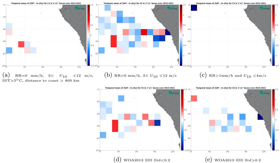
Figure 14: Temporal mean gridded over spatial boxes of size 1^\circ \times 1^\circ of \Delta SSS (SMAP SSS L2 v5.0 (JPL) - TSG (GOSUD-Research-vessel)) for 5 different subdatasets corresponding to:RR=0 mm/h, 3 < U_{10} < 12 m/s, SST>5°C, distance to coast > 800 km (a), RR=0 mm/h, 3 < U_{10} < 12 m/s (b), RR>1mm/h and U_{10} < 4 m/s (c), WOA2013 SSS Std<0.2 (d), WOA2013 SSS Std>0.2 (e).
