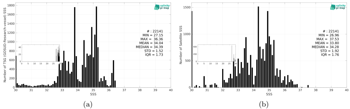
Figure 3: Histograms of SSS from TSG (GOSUD-Research-vessel) (a) and SMAP SSS L2 v5.0 (JPL) (b) considering all match-up pairs per bins of 0.1 over the Congo river plume Pi-MEP region and for the full satellite product period.
