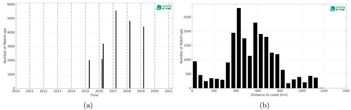
Figure 2: Number of match-ups between TSG (GOSUD-Research-vessel) and SMAP SSS L2 v5.0 (JPL) SSS as a function of time (a) and as function of the distance to coast (b) over the Congo river plume Pi-MEP region and for the full satellite product period.
