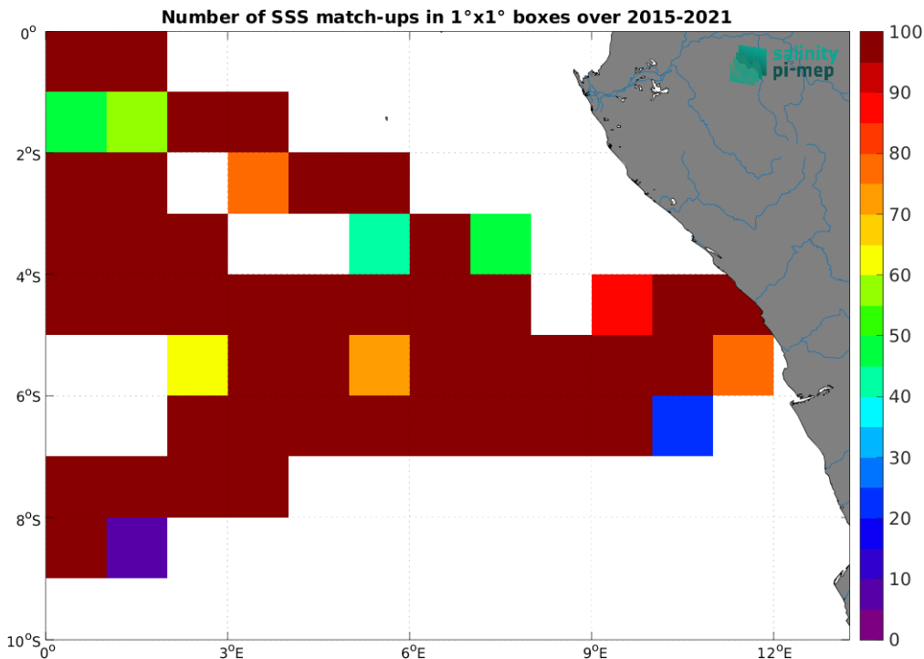
Figure 5: Number of SSS match-ups between TSG (GOSUD-Research-vessel) SSS and the SMAP SSS L2 v5.0 (JPL) SSS product for the Congo river plume Pi-MEP region over 1^\circ \times 1^\circ boxes and for the full satellite product period.
