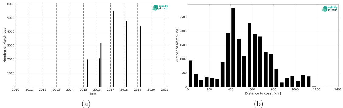
Figure 1: Number of match-ups between TSG (GOSUD-Research-vessel) and SMAP SSS L2 v5.0 (JPL) SSS as a function of time (a) and as function of the distance to the coast (b) over the Congo river plume Pi-MEP region and for the full satellite product period.
