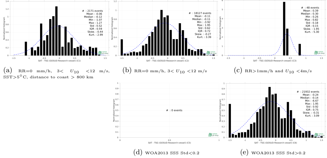
Figure 13: Normalized histogram of \Delta SSS (SMAP SSS L2 v5.0 (JPL) - TSG (GOSUD-Research-vessel)) for 5 different subdatasets corresponding to: RR=0 mm/h, 3 < U_{10} < 12 m/s, SST > 5°C, distance to coast > 800 km (a), RR=0 mm/h, 3 < U_{10} < 12 m/s (b), RR > 1mm/h and U_{10} < 4 m/s (c), WOA2013 SSS Std < 0.2 (d), WOA2013 SSS Std > 0.2 (e).
