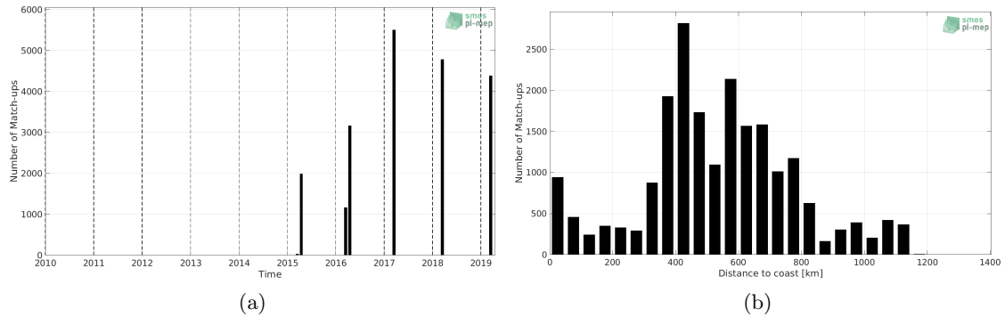
Figure 1: Number of match-ups between TSG (GOSUD-Research-vessel) and SMAP SSS L2 v5.0 (JPL) SSS as a function of time (a) and as function of the distance to coast (b) over the Congo river plume Pi-MEP region and for the full satellite product period.
