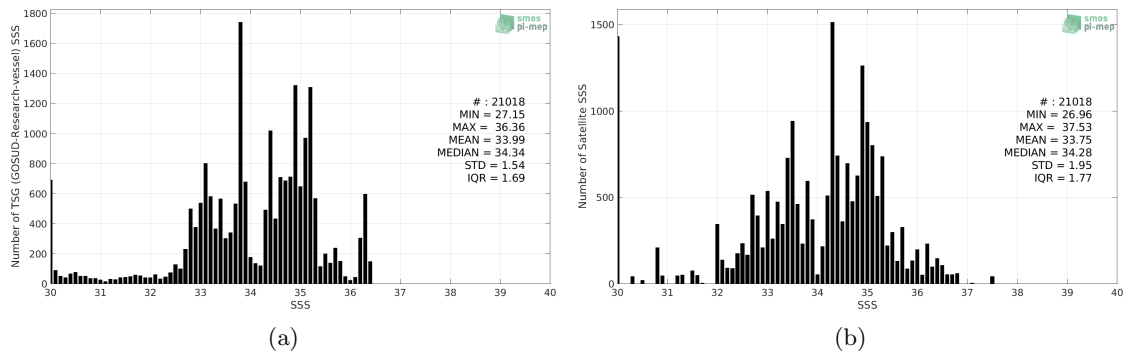
Figure 2: Histograms of SSS from TSG (GOSUD-Research-vessel) (a) and SMAP SSS L2 v5.0 (JPL) (b) considering all match-up pairs per bins of 0.1 over the Congo river plume Pi-MEP region and for the full satellite product period.
