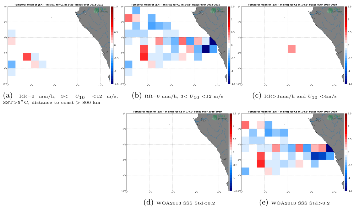
Figure 12: Temporal mean gridded over spatial boxes of size 1^\circ \times 1^\circ of \Delta SSS (SMAP SSS L2 v5.0 (JPL) - TSG (GOSUD-Research-vessel)) for 5 different subdatasets corresponding to: RR=0 mm/h, 3 < U_{10} < 12 m/s, SST > 5°C, distance to coast > 800 km (a), RR=0 mm/h, 3 < U_{10} < 12 m/s (b), RR > 1mm/h and U_{10} < 4 m/s (c), WOA2013 SSS Std < 0.2 (d), WOA2013 SSS Std > 0.2 (e).
