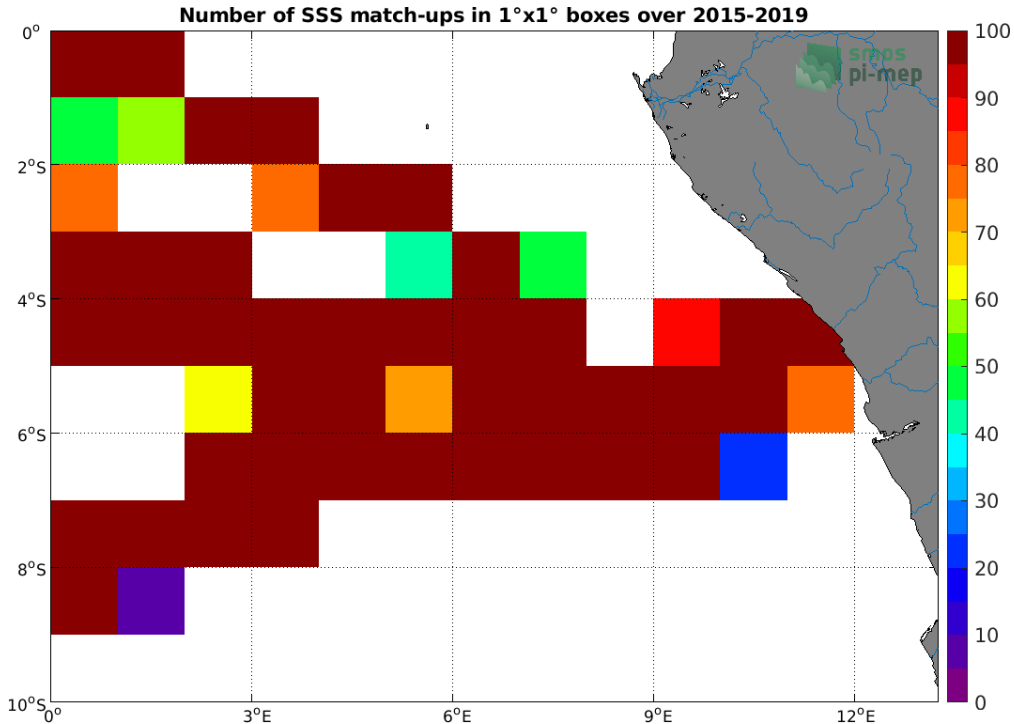
Figure 4: Number of SSS match-ups between TSG (GOSUD-Research-vessel) SSS and the SMAP SSS L2 v5.0 (JPL) SSS product for the Congo river plume Pi-MEP region over 1^\circ \times 1^\circ boxes and for the full satellite product period.
