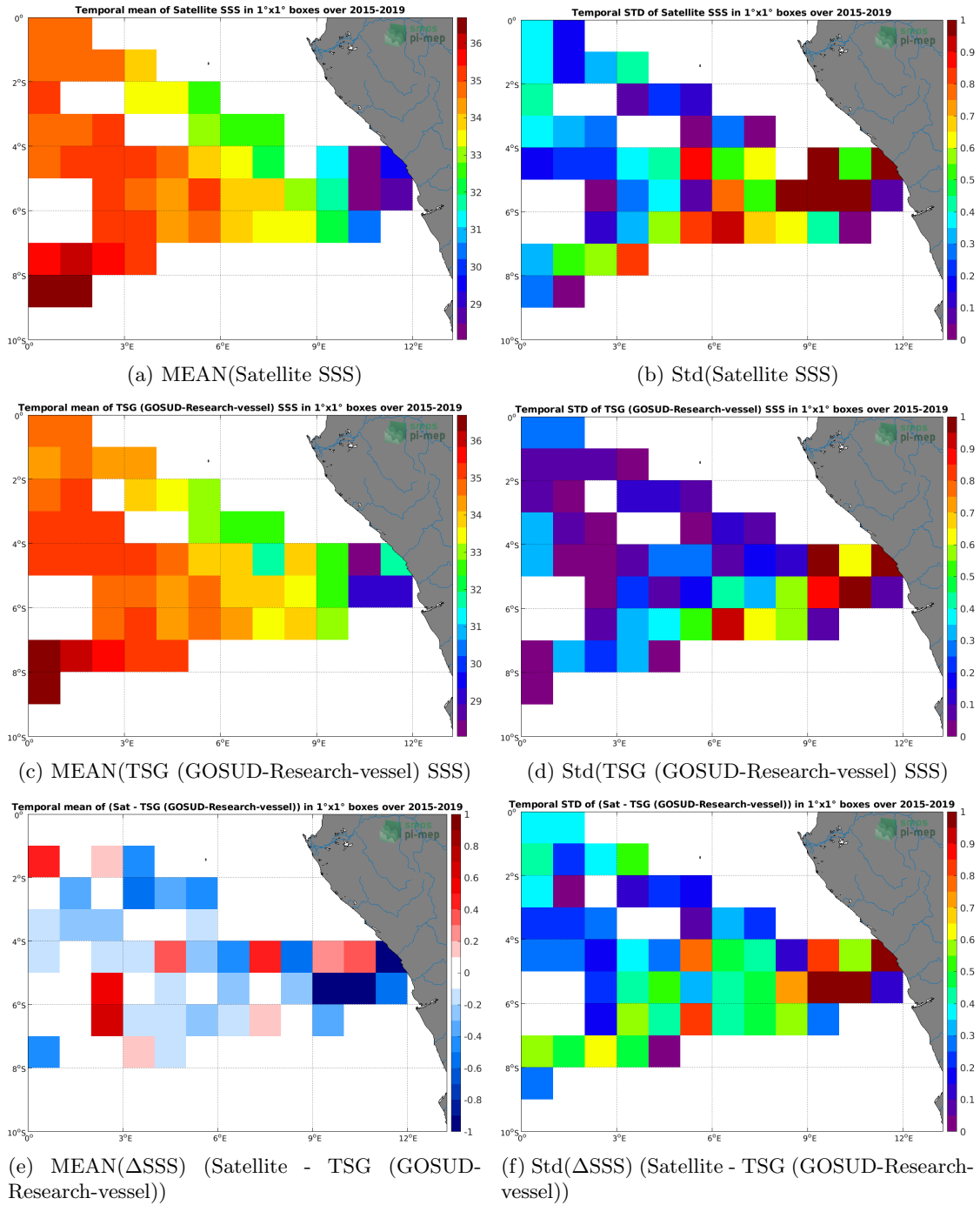
Figure 6: Temporal mean (left) and Std (right) of SSS from SMAP SSS L2 v5.0 (JPL) (top), TSG (GOSUD-Research-vessel) (middle), and of \Delta SSS (Satellite - TSG (GOSUD-Research-vessel)). Only match-up pairs are used to generate these maps.
