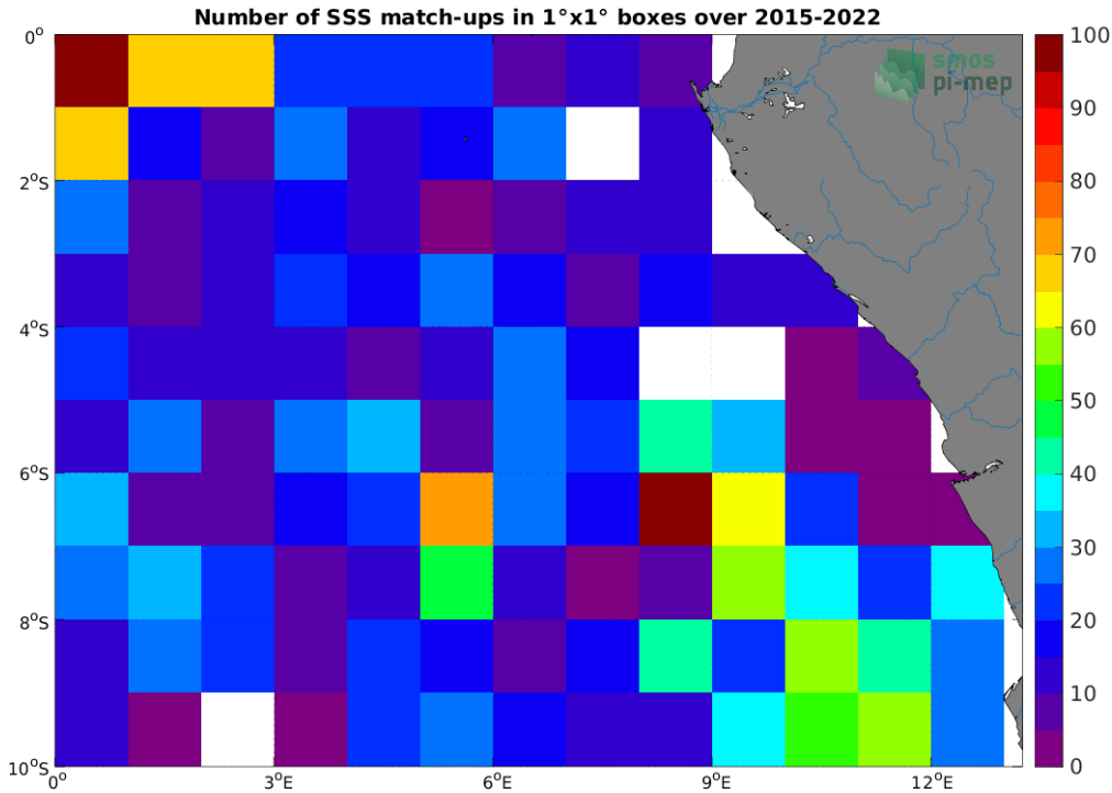
Figure 4: Number of SSS match-ups between Argo SSS and the SMAP SSS L2 v5.0 (JPL) SSS product for the Congo river plume Pi-MEP region over 1^\circ \times 1^\circ boxes and for the full satellite product period.
