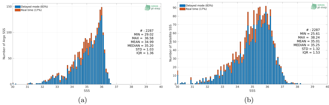
Figure 2: Histograms of SSS from Argo (a) and SMAP SSS L2 v5.0 (JPL) (b) considering all match-up pairs per bins of 0.1 over the Congo river plume Pi-MEP region and for the full satellite product period.
