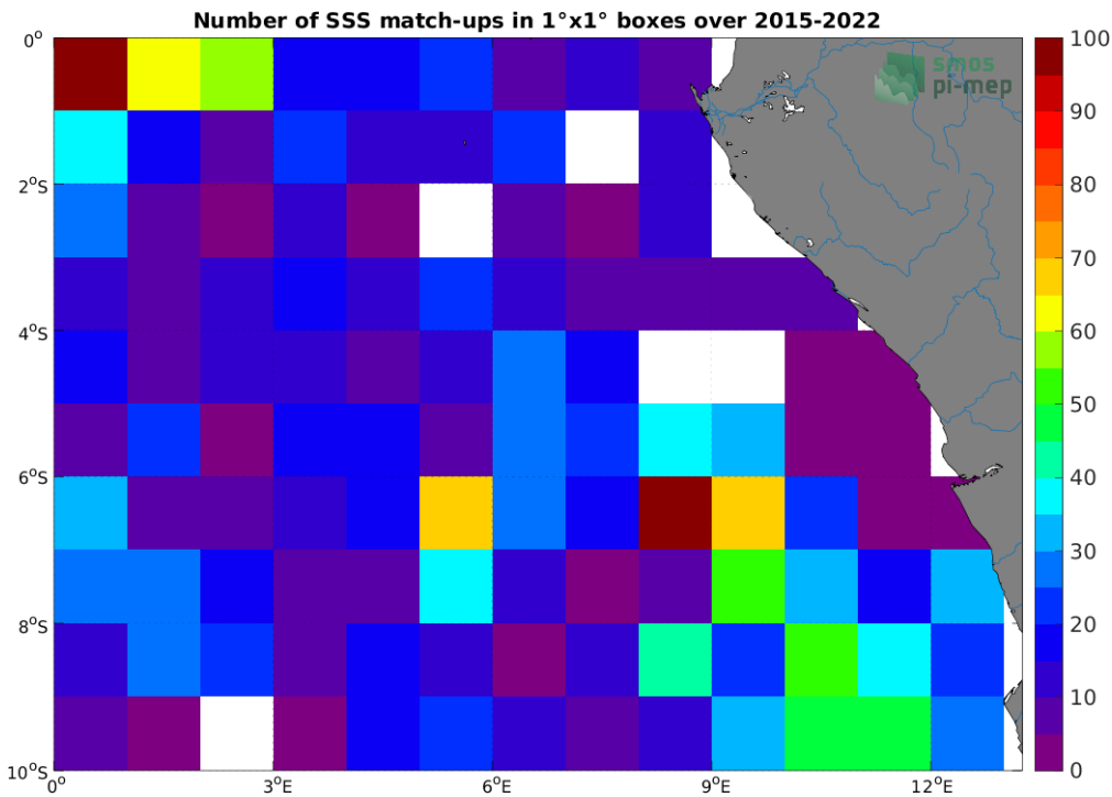
Figure 4: Number of SSS match-ups between Argo SSS and the SMAP SSS L2 v5.0 (JPL) SSS product for the Congo river plume Pi-MEP region over 1^{\circ} \times 1^{\circ} boxes and for the full satellite product period.
