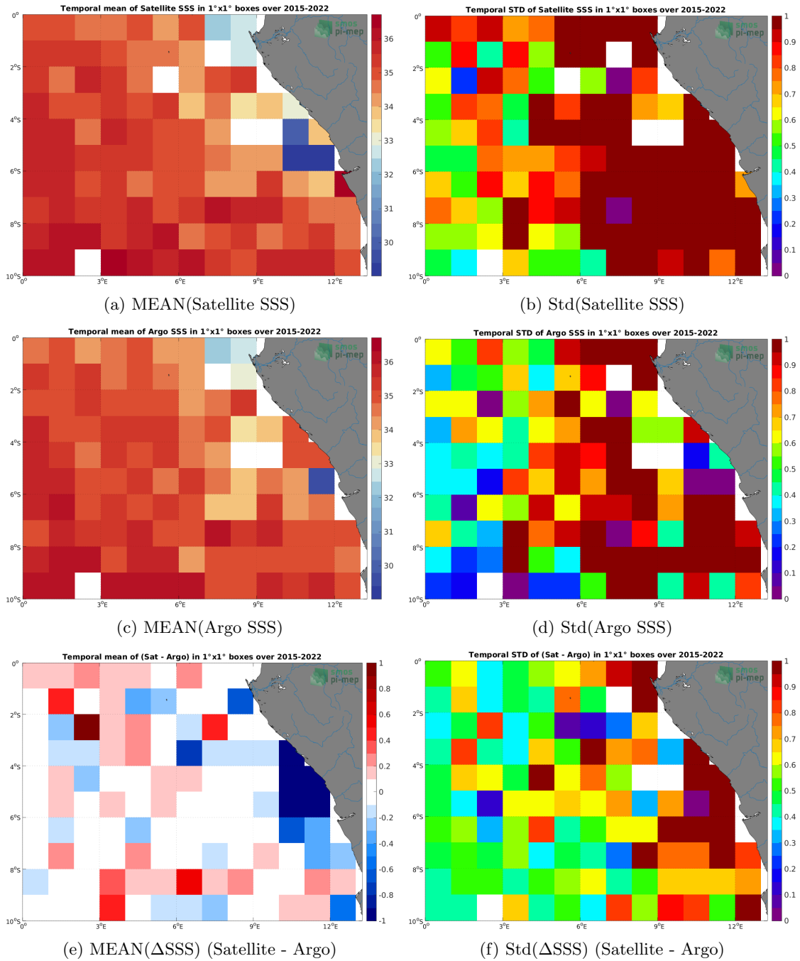
Figure 6: Temporal mean (left) and Std (right) of SSS from SMAP SSS L2 v5.0 (JPL) (top), Argo (middle), and of \Delta SSS (Satellite - Argo). Only match-up pairs are used to generate these maps.
