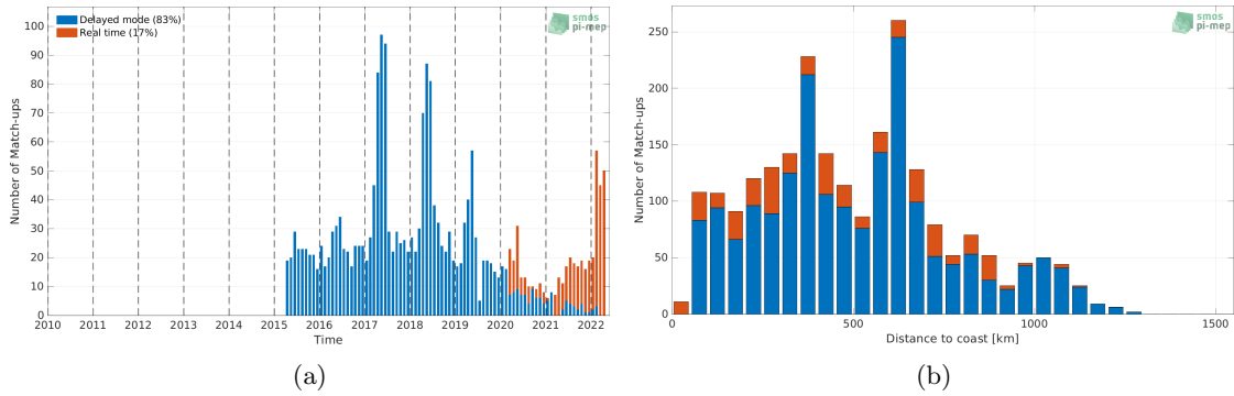
Figure 1: Number of match-ups between Argo and SMAP SSS L2 v5.0 (JPL) SSS as a function of time (a) and as function of the distance to coast (b) over the Congo river plume Pi-MEP region and for the full satellite product period.
