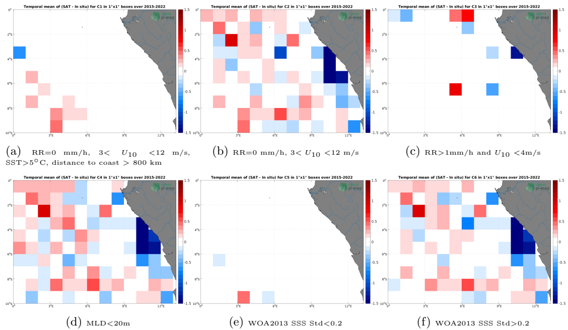
Figure 12: Temporal mean gridded over spatial boxes of size 1^\circ \times 1^\circ of \Delta SSS (SMAP SSS L2 v5.0 (JPL) - Argo) for 6 different subdatasets corresponding to:RR=0 mm/h, 3 < U_{10} < 12 m/s, SST >5^\circ C, distance to coast > 800 km (a), RR=0 mm/h, 3 < U_{10} < 12 m/s (b), RR >1 mm/h and U_{10} < 4 m/s (c),MLD <20 m (d),WOA2013 SSS Std <0.2 (e),WOA2013 SSS Std >0.2 (f).
