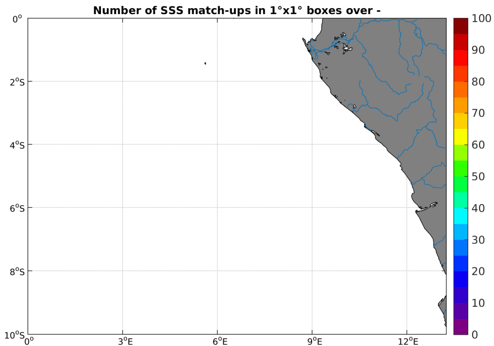
Figure 4: Number of SSS match-ups between TSG-SAMOS SSS and the SMAP-L2-JPL-V4 SSS product for the Congo river plume Pi-MEP region over 1^\circ \times 1^\circ boxes and for the full satellite product period.
