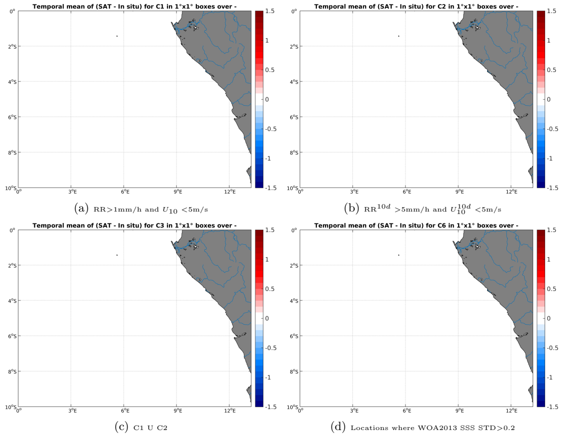
Figure 12: Temporal mean gridded over spatial boxes of size 1^\circ \times 1^\circ of \Delta SSS (SMAP-L2-JPL-V4 - TSG-SAMOS) for 4 different subdatasets corresponding to: RR > 1\text{mm/h} and U_{10} < 5\text{m/s} (a), RR^{10d} > 5\text{mm/h} and U_{10}^{10d} < 5\text{m/s} (b), C1 \cup C2 (c), Locations where WOA2013 SSS STD > 0.2 (d).
