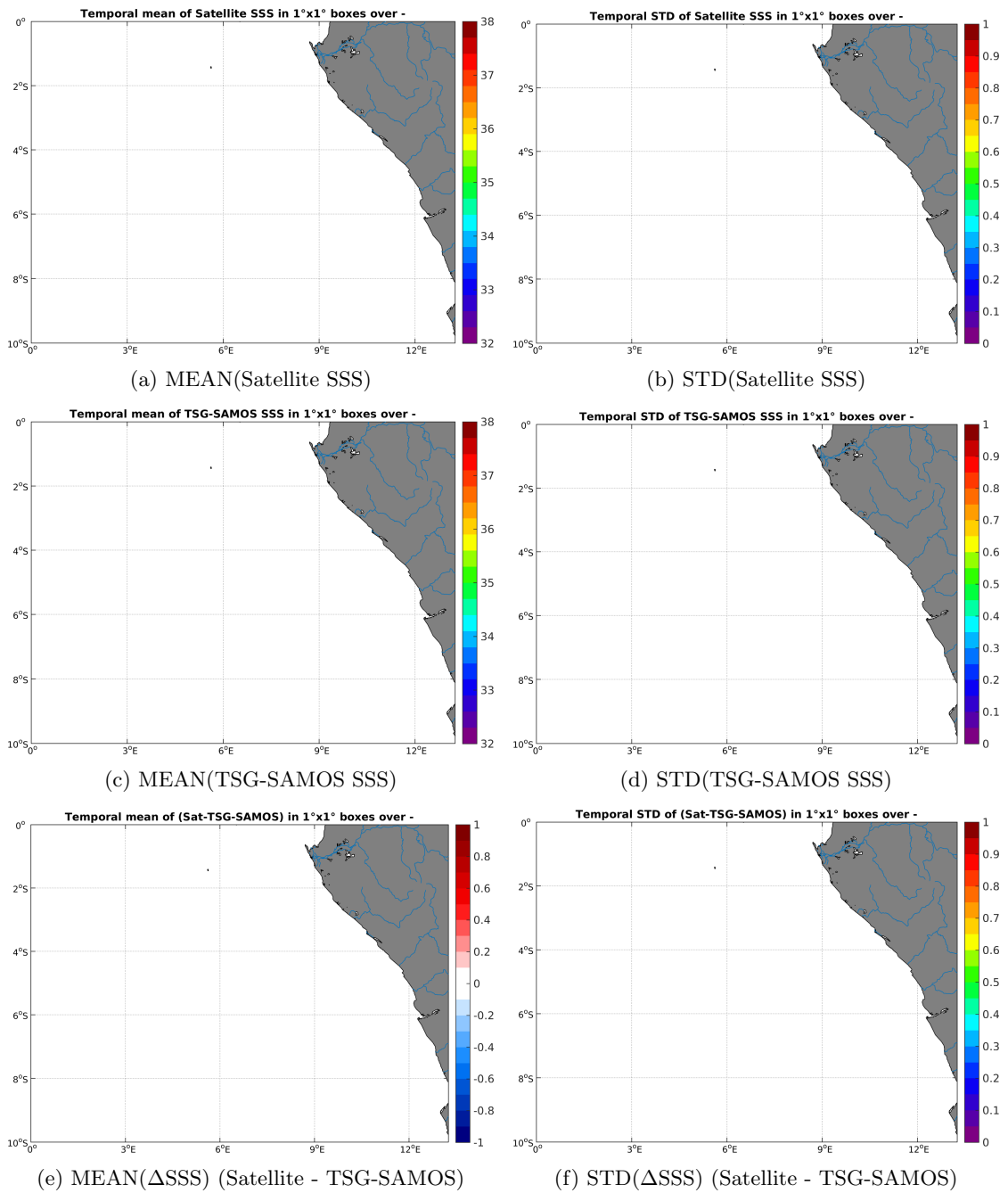
Figure 6: Temporal mean (left) and STD (right) of SSS from SMAP-L2-JPL-V4 (top), TSG-SAMOS (middle), and of \Delta SSS (Satellite - TSG-SAMOS). Only match-up pairs are used to generate these maps.
