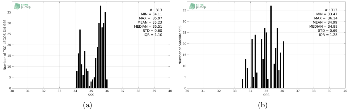
Figure 2: Histograms of SSS from TSG-LEGOS-DM (a) and SMAP-L2-JPL-V4 (b) considering all match-up pairs per bins of 0.1 over the Congo river plume Pi-MEP region and for the full satellite product period.
