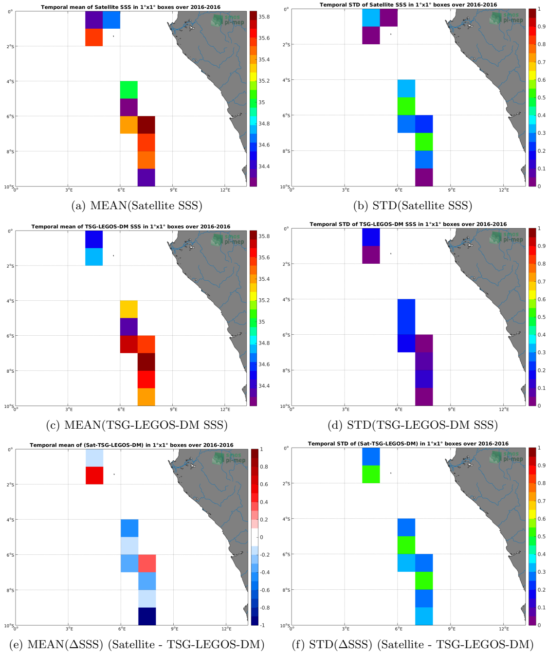
Figure 6: Temporal mean (left) and STD (right) of SSS from SMAP-L2-JPL-V4 (top), TSG-LEGOS-DM (middle), and of \Delta SSS (Satellite - TSG-LEGOS-DM). Only match-up pairs are used to generate these maps.
