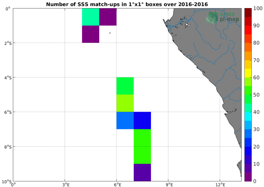
Figure 4: Number of SSS match-ups between TSG-LEGOS-DM SSS and the SMAP-L2-JPL-V4 SSS product for the Congo river plume Pi-MEP region over 1°x1° boxes and for the full satellite product period.
