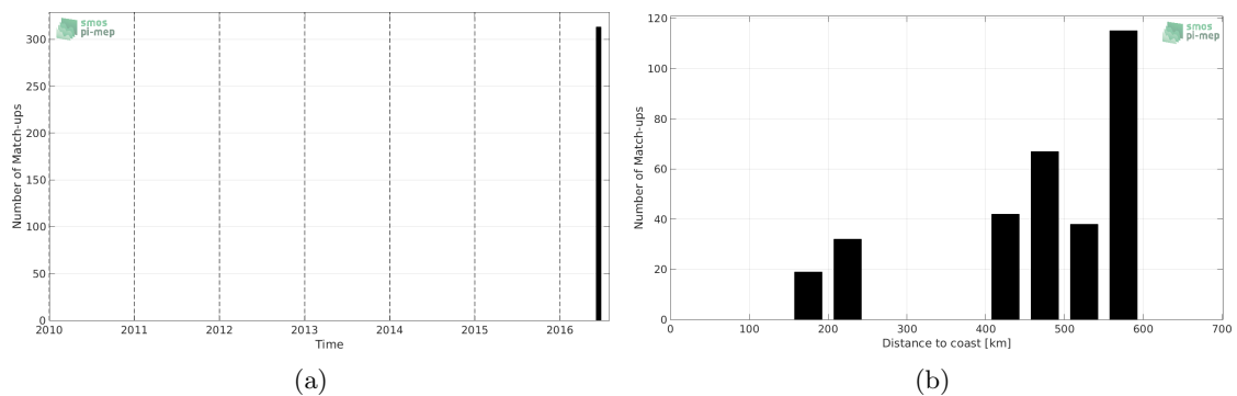
Figure 1: Number of match-ups between TSG-LEGOS-DM and SMAP-L2-JPL-V4 SSS as a function of time (a) and as function of the distance to coast (b) over the Congo river plume Pi-MEP region and for the full satellite product period.
