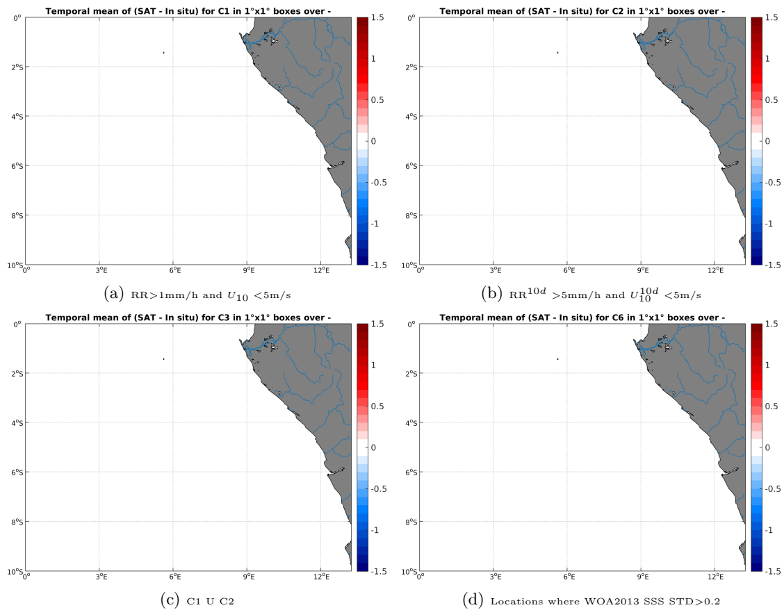
Figure 12: Temporal mean gridded over spatial boxes of size 1^\circ \times 1^\circ of \Delta SSS (SMAP-L2-JPL-V4 - TSG-GOSUD-Sailing-ship) for 4 different subdatasets corresponding to:RR >1 mm/h and U_{10} < 5 m/s (a), RR ^{10d} > 5 mm/h and U_{10}^{10d} < 5 m/s (b), C1 U C2 (c),Locations where WOA2013 SSS STD >0.2 (d).
