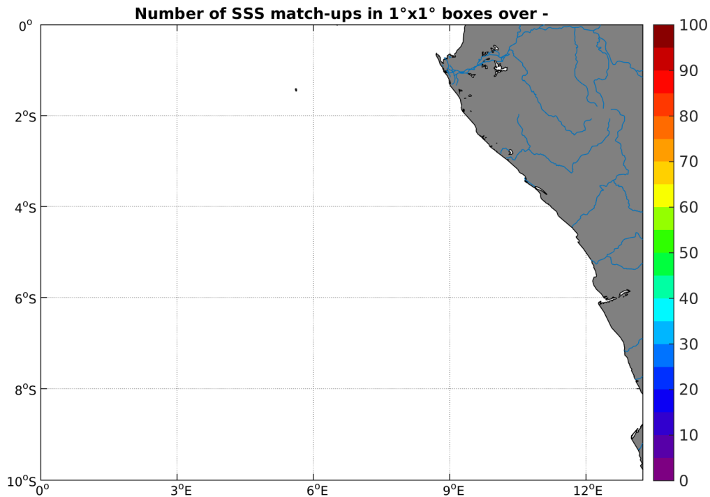
Figure 4: Number of SSS match-ups between TSG-GOSUD-Sailing-ship SSS and the SMAP-L2-JPL-V4 SSS product for the Congo river plume Pi-MEP region over 1^\circ \times 1^\circ boxes and for the full satellite product period.
