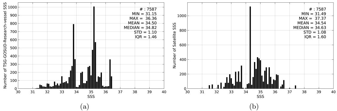
Figure 2: Histograms of SSS from TSG-GOSUD-Research-vessel (a) and SMAP-L2-JPL-V4 (b) considering all match-up pairs per bins of 0.1 over the Congo river plume Pi-MEP region and for the full satellite product period.
