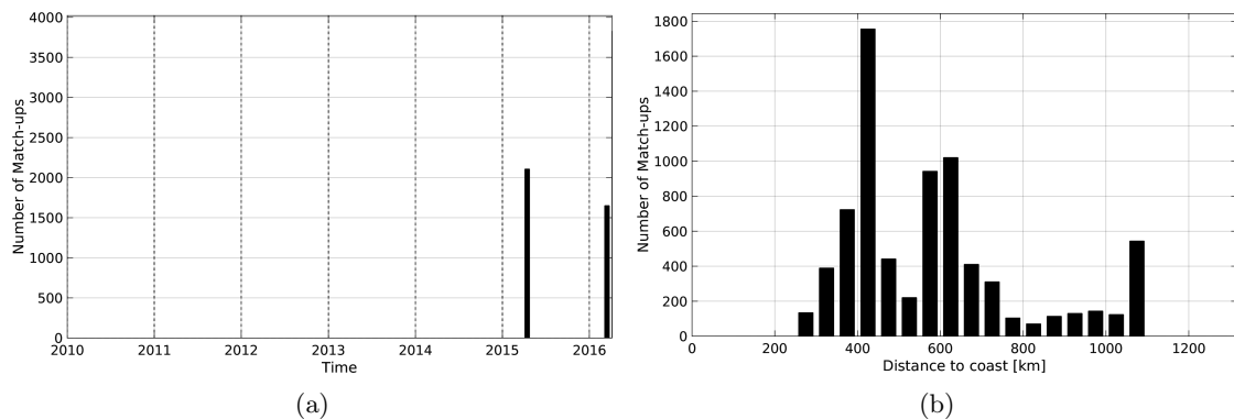
Figure 1: Number of match-ups between TSG-GOSUD-Research-vessel and SMAP-L2-JPL-V4 SSS as a function of time (a) and as function of the distance to coast (b) over the Congo river plume Pi-MEP region and for the full satellite product period.
