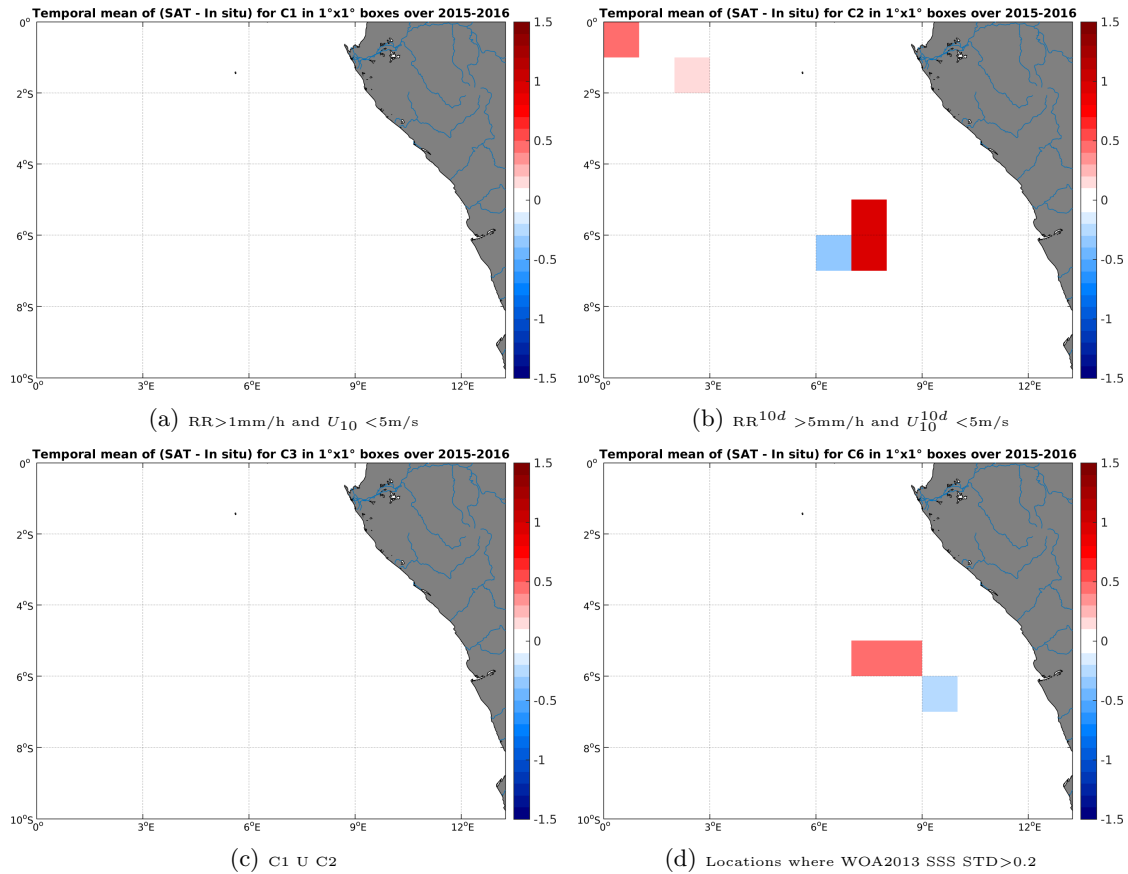
Figure 12: Temporal mean gridded over spatial boxes of size 1^\circ \times 1^\circ of \Delta SSS (SMAP-L2-JPL-V4 - TSG-GOSUD-Research-vessel) for 4 different subdatasets corresponding to:RR >1 mm/h and U_{10} < 5 m/s (a), RR^{10d} > 5 mm/h and U_{10}^{10d} < 5 m/s (b), C1 U C2 (c),Locations where WOA2013 SSS STD >0.2 (d).
