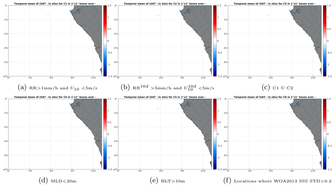
Figure 12: Temporal mean gridded over spatial boxes of size 1^\circ \times 1^\circ of \Delta SSS (SMAP-L2-JPL-V4 - Sea mammals) for 6 different subdatasets corresponding to: RR > 1mm/h and U_{10} < 5\text{m/s} (a), RR^{10d} > 5\text{mm/h} and U_{10}^{10d} < 5\text{m/s} (b), C1 U C2 (c), MLD < 20m (d), BLT > 10m (e), Locations where WOA2013 SSS STD > 0.2 (f).
