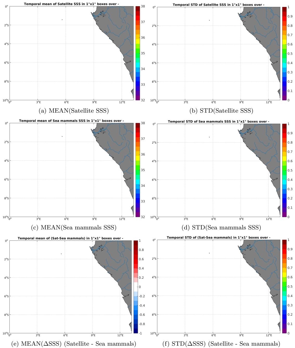
Figure 6: Temporal mean (left) and STD (right) of SSS from SMAP-L2-JPL-V4 (top), Sea mammals (middle), and of \Delta SSS (Satellite - Sea mammals). Only match-up pairs are used to generate these maps.
