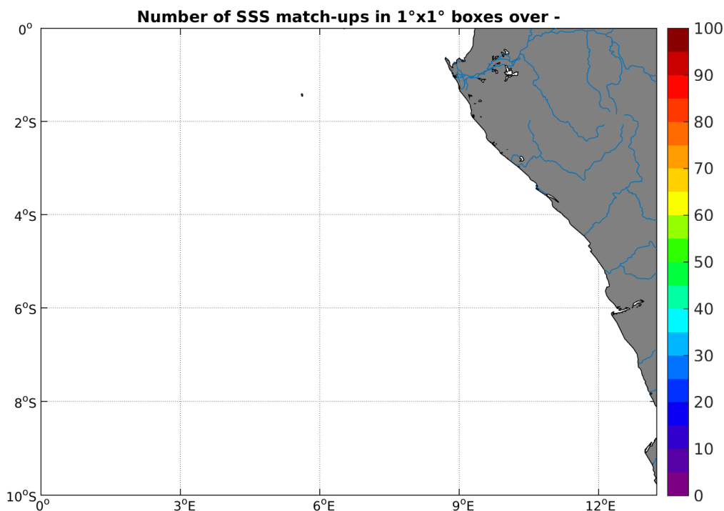
Figure 4: Number of SSS match-ups between Sea mammals SSS and the SMAP-L2-JPL-V4 SSS product for the Congo river plume Pi-MEP region over 1°x1° boxes and for the full satellite product period.
