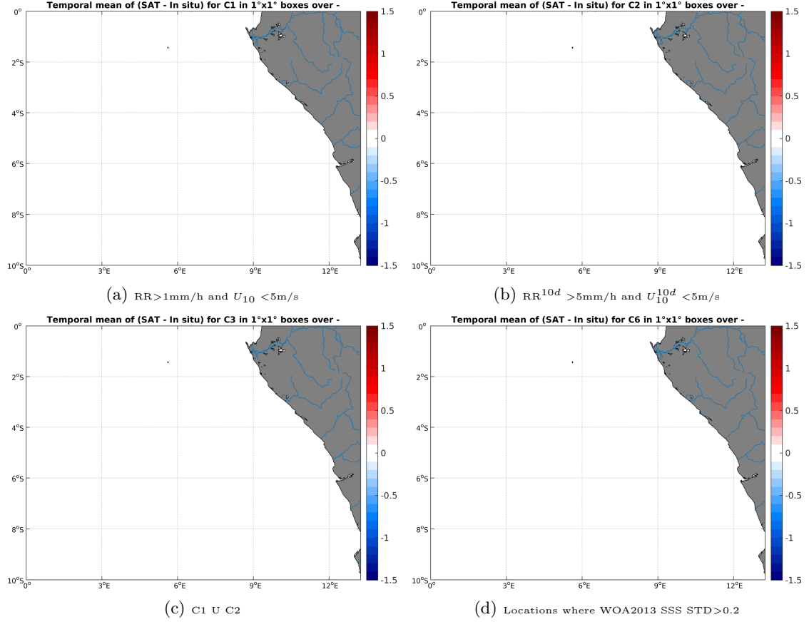
Figure 11: Temporal mean gridded over spatial boxes of size 1^\circ \times 1^\circ of \Delta SSS (SMAP-L2-JPL-V4 - Surface drifters) for 4 different subdatasets corresponding to: RR > 1\text{mm/h} and U_{10} < 5\text{m/s} (a), RR^{10d} > 5\text{mm/h} and U_{10}^{10d} < 5\text{m/s} (b), C1 \cup C2 (c), Locations where WOA2013 SSS STD > 0.2 (d).
