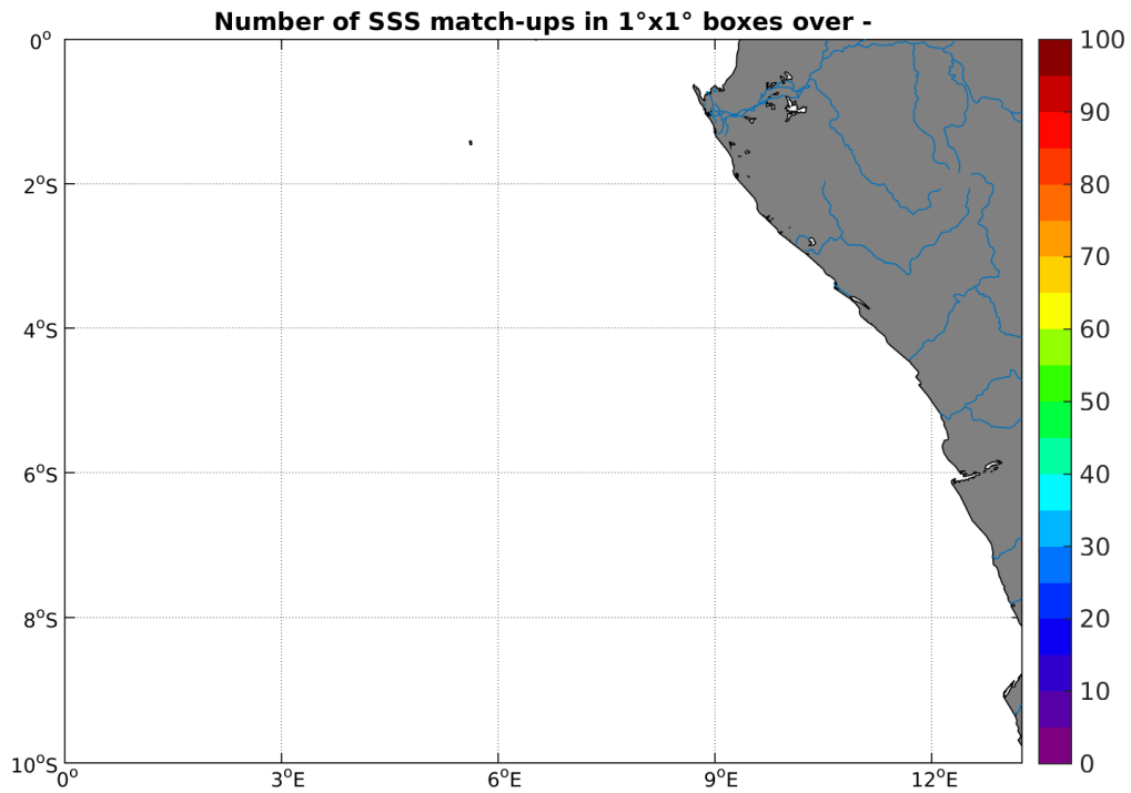
Figure 3: Number of SSS match-ups between Surface drifters SSS and the SMAP-L2-JPL-V4 SSS product for the Congo river plume Pi-MEP region over 1^\circ \times 1^\circ boxes and for the full satellite product period.
