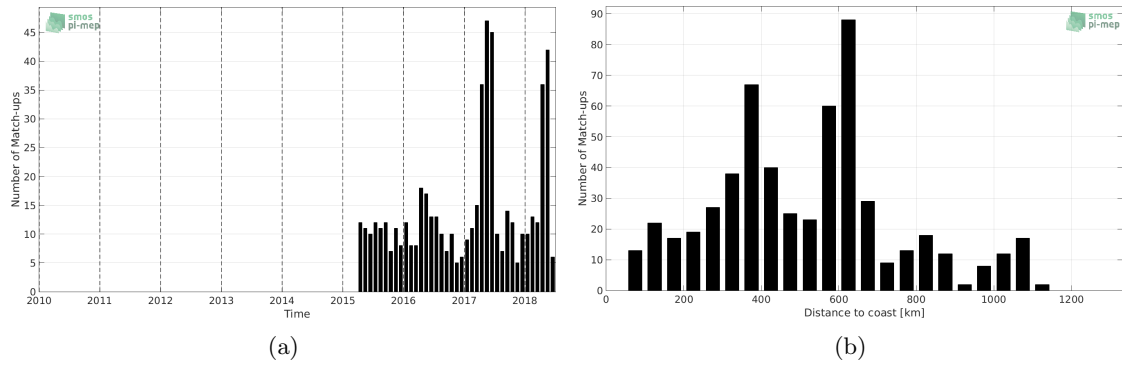
Figure 1: Number of match-ups between Argo and SMAP-L2-JPL-V4 SSS as a function of time (a) and as function of the distance to coast (b) over the Congo river plume Pi-MEP region and for the full satellite product period.
