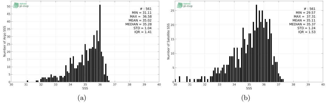
Figure 2: Histograms of SSS from Argo (a) and SMAP-L2-JPL-V4 (b) considering all match-up pairs per bins of 0.1 over the Congo river plume Pi-MEP region and for the full satellite product period.
