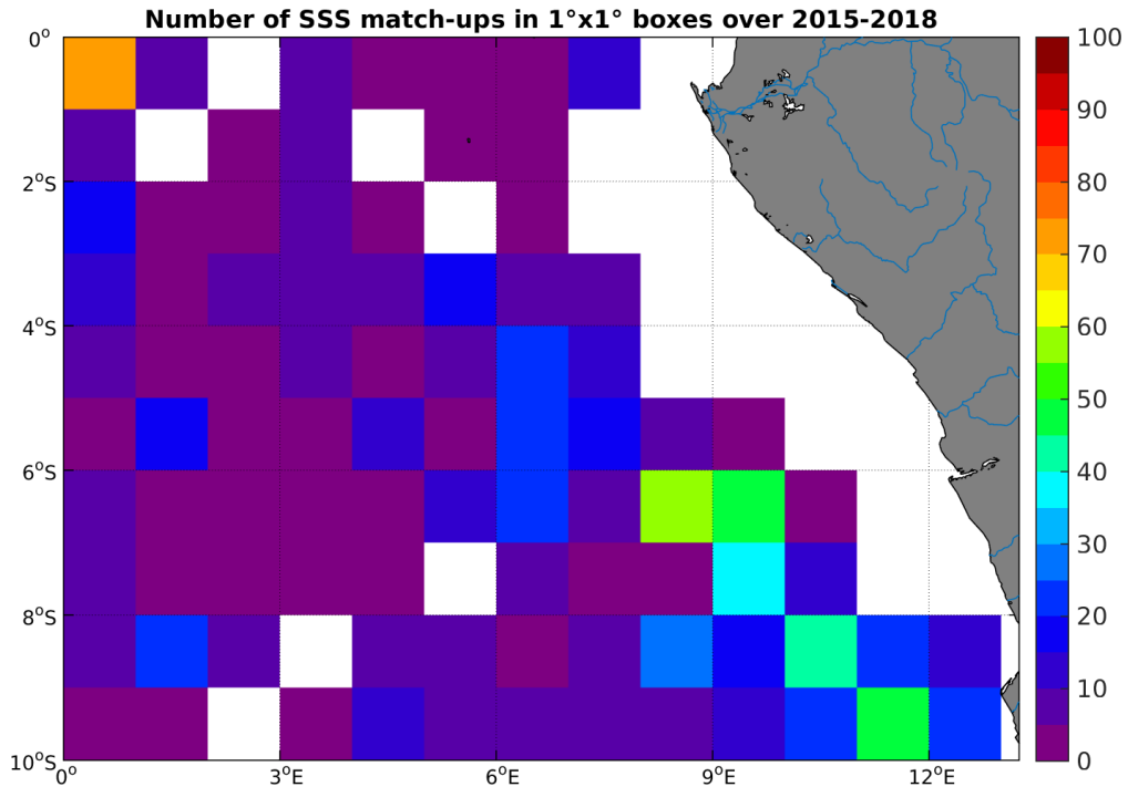
Figure 4: Number of SSS match-ups between Argo SSS and the SMAP-L2-JPL-V4 SSS product for the Congo river plume Pi-MEP region over 1^\circ \times 1^\circ boxes and for the full satellite product period.
