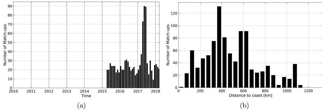
Figure 1: Number of match-ups between Argo and SMAP-L2-JPL-V4 SSS as a function of time (a) and as function of the distance to coast (b) over the Congo river plume Pi-MEP region and for the full satellite product period.
