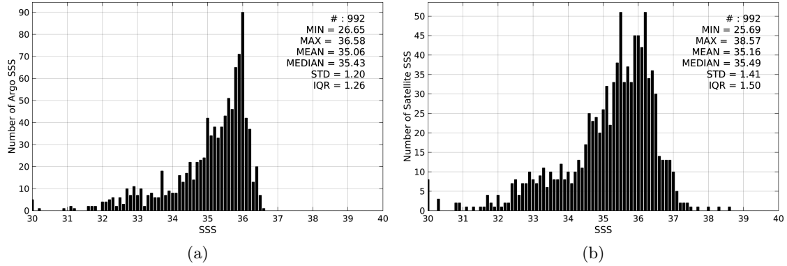
Figure 2: Histograms of SSS from Argo (a) and SMAP-L2-JPL-V4 (b) considering all match-up pairs per bins of 0.1 over the Congo river plume Pi-MEP region and for the full satellite product period.
