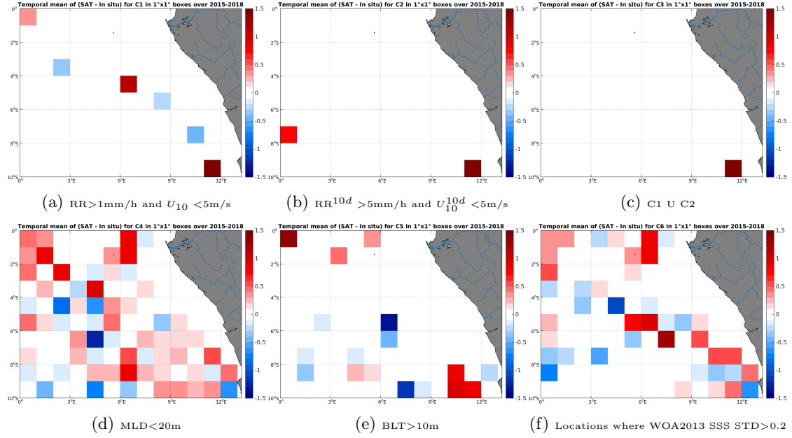
Figure 12: Temporal mean gridded over spatial boxes of size 1^\circ \times 1^\circ of \Delta\text{SSS} (SMAP-L2-JPL-V4 - Argo) for 6 different subdatasets corresponding to: \text{RR} > 1\text{mm/h} and U_{10} < 5\text{m/s} (a), \text{RR}^{10d} > 5\text{mm/h} and U_{10}^{10d} < 5\text{m/s} (b), C1 U C2 (c), \text{MLD} < 20\text{m} (d), \text{BLT} > 10\text{m} (e), Locations where WOA2013 SSS STD > 0.2 (f).
