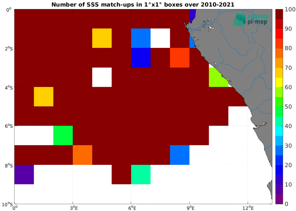
Figure 5: Number of SSS match-ups between TSG (GOSUD-Research-vessel) SSS and the ISAS v7 - Monthly (Ifremer-LOPS-CMEMS) SSS product for the Congo river plume Pi-MEP region over 1^\circ \times 1^\circ boxes and for the full satellite product period.
