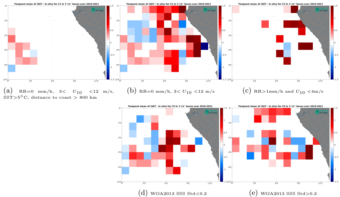
Figure 14: Temporal mean gridded over spatial boxes of size 1^\circ \times 1^\circ of \Delta SSS (ISAS v7 - Monthly (Ifremer-LOPS-CMEMS) - TSG (GOSUD-Research-vessel)) for 5 different subdatasets corresponding to:RR=0 mm/h, 3 < U_{10} < 12 m/s, SST>5°C, distance to coast > 800 km (a), RR=0 mm/h, 3 < U_{10} < 12 m/s (b), RR>1mm/h and U_{10} < 4 m/s (c), WOA2013 SSS Std<0.2 (d), WOA2013 SSS Std>0.2 (e).
