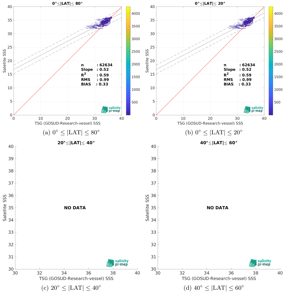
Figure 10: Contour maps of the concentration of ISAS v7 - Monthly (Ifremer-LOPS-CMEMS) SSS (y-axis) versus TSG (GOSUD-Research-vessel) SSS (x-axis) at match-up pairs for different latitude bands. For each plot, the red line shows x=y . The black thin and dashed lines indicate a linear fit through the data cloud and the \pm 95\% confidence levels, respectively. The number match-up pairs n , the slope and R^2 coefficient of the linear fit, the root mean square (RMS) and the mean bias between satellite and in situ data are indicated for each latitude band in each plots.
