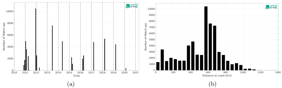
Figure 2: Number of match-ups between TSG (GOSUD-Research-vessel) and ISAS v7 - Monthly (Ifremer-LOPS-CMEMS) SSS as a function of time (a) and as function of the distance to coast (b) over the Congo river plume Pi-MEP region and for the full satellite product period.
