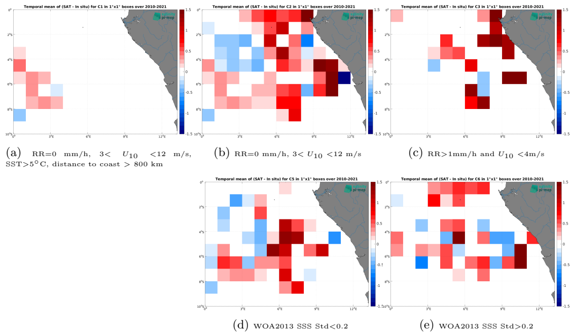
Figure 14: Temporal mean gridded over spatial boxes of size 1^\circ \times 1^\circ of \Delta SSS (ISAS - TSG (GOSUD-Research-vessel)) for 5 different subdatasets corresponding to:RR=0 mm/h, 3 < U_{10} < 12 m/s, SST>5°C, distance to coast > 800 km (a), RR=0 mm/h, 3 < U_{10} < 12 m/s (b), RR>1mm/h and U_{10} < 4 m/s (c), WOA2013 SSS Std<0.2 (d), WOA2013 SSS Std>0.2 (e).
