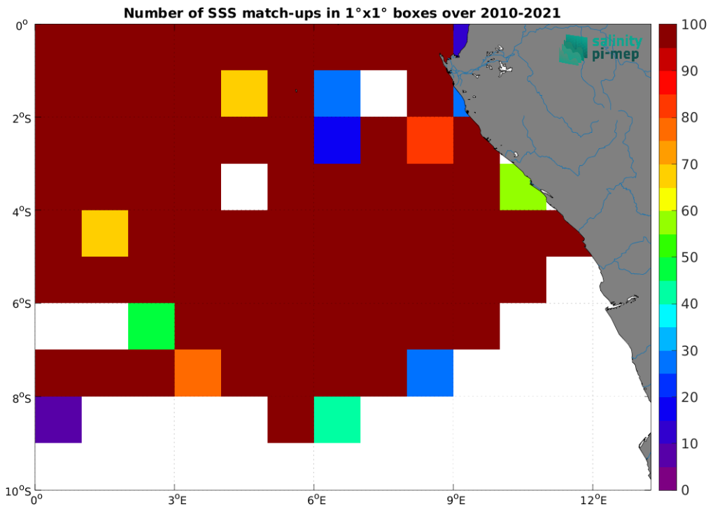
Figure 5: Number of SSS match-ups between TSG (GOSUD-Research-vessel) SSS and the ISAS SSS product for the Congo river plume Pi-MEP region over 1^\circ \times 1^\circ boxes and for the full satellite product period.
