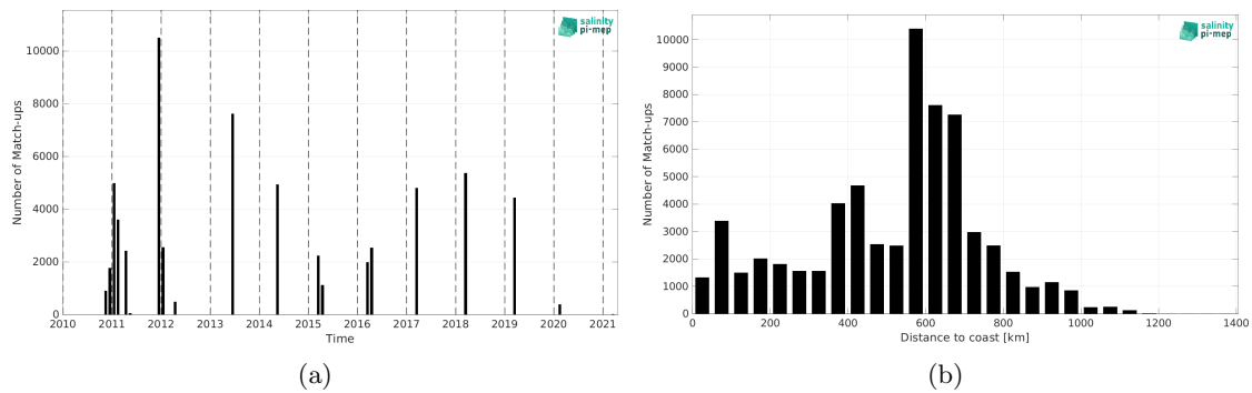
Figure 2: Number of match-ups between TSG (GOSUD-Research-vessel) and ISAS SSS as a function of time (a) and as function of the distance to coast (b) over the Congo river plume Pi-MEP region and for the full satellite product period.
