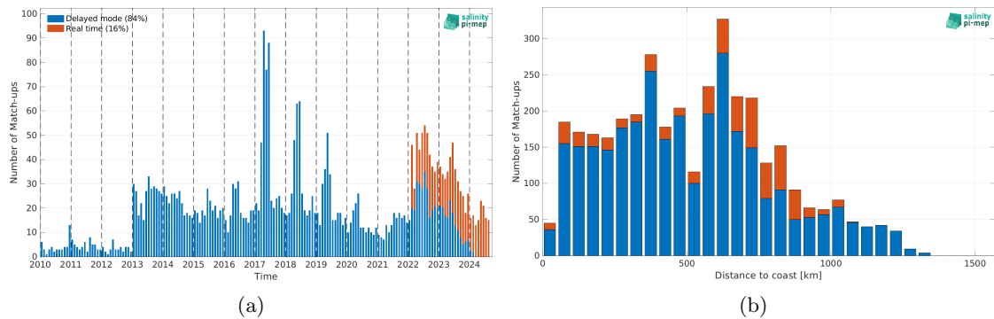
Figure 2: Number of match-ups between Argo and ISAS v7 - Monthly (Ifremer-LOPS-CMEMS) SSS as a function of time (a) and as function of the distance to coast (b) over the Congo river plume Pi-MEP region and for the full satellite product period.
