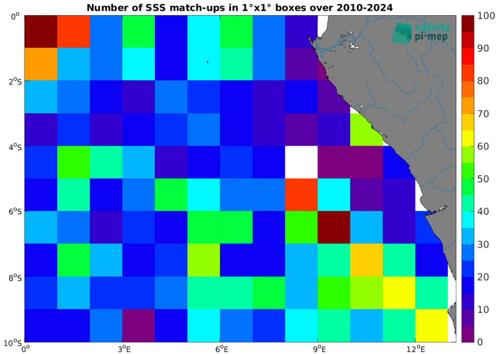
Figure 5: Number of SSS match-ups between Argo SSS and the ISAS v7 - Monthly (Ifremer-LOPS-CMEMS) SSS product for the Congo river plume Pi-MEP region over 1^\circ \times 1^\circ boxes and for the full satellite product period.
