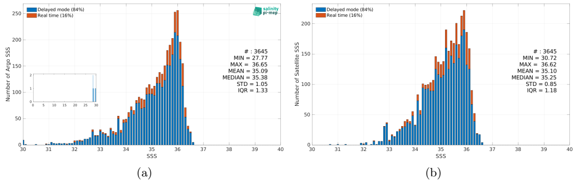
Figure 3: Histograms of SSS from Argo (a) and ISAS v7 - Monthly (Ifremer-LOPS-CMEMS) (b) considering all match-up pairs per bins of 0.1 over the Congo river plume Pi-MEP region and for the full satellite product period.
