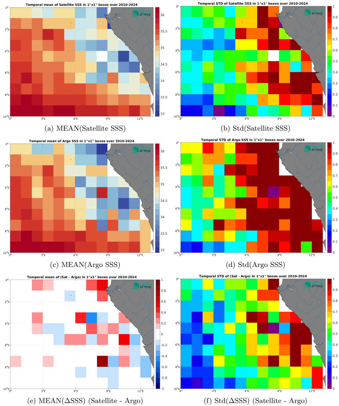
Figure 7: Temporal mean (left) and Std (right) of SSS from ISAS v7 - Monthly (Ifremer-LOPS-CMEMS) (top), Argo (middle), and of \Delta SSS (Satellite - Argo). Only match-up pairs are used to generate these maps.
