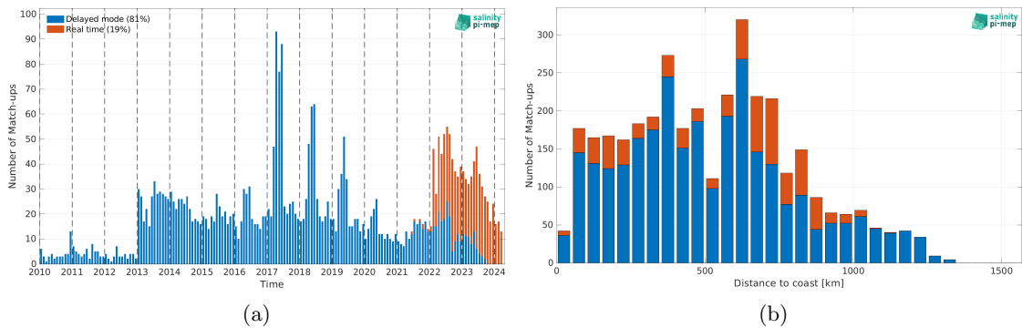
Figure 2: Number of match-ups between Argo and ISAS SSS as a function of time (a) and as function of the distance to coast (b) over the Congo river plume Pi-MEP region and for the full satellite product period.
