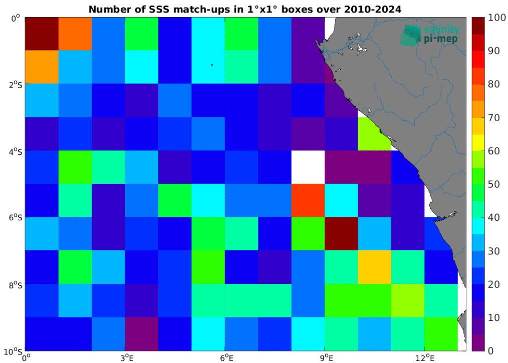
Figure 5: Number of SSS match-ups between Argo SSS and the ISAS SSS product for the Congo river plume Pi-MEP region over 1^{\circ} \times 1^{\circ} boxes and for the full satellite product period.
