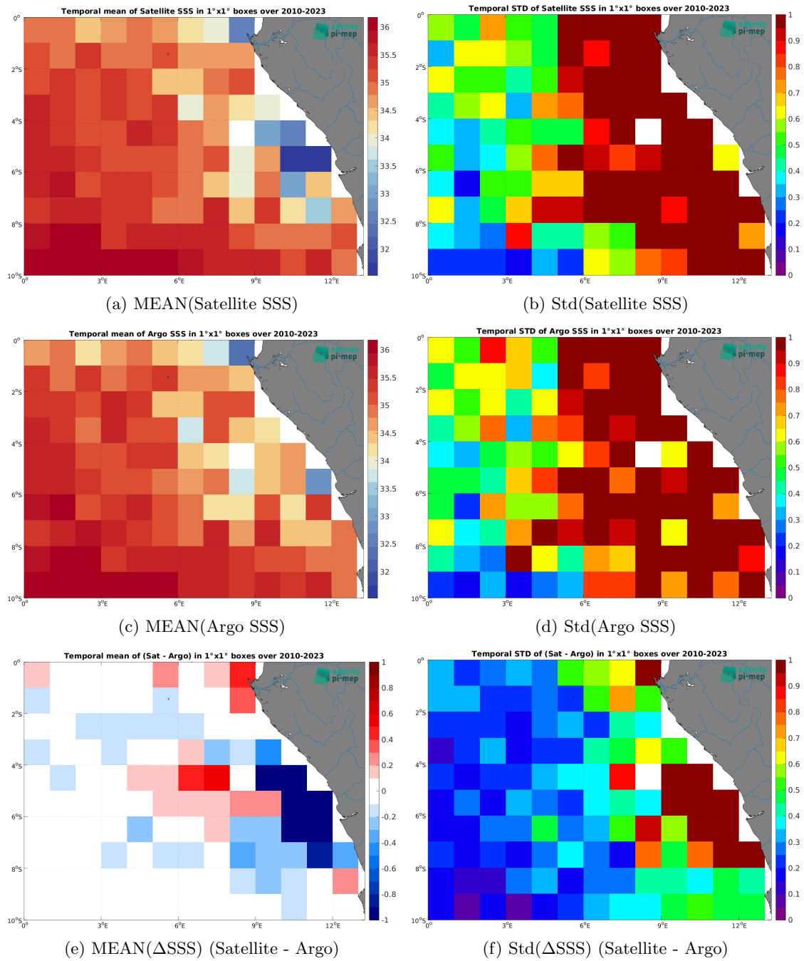
Figure 7: Temporal mean (left) and Std (right) of SSS from CCI SSS L4 Merged-OI v5.5 - 7-day running (ESA) (top), Argo (middle), and of \Delta SSS (Satellite - Argo). Only match-up pairs are used to generate these maps.
