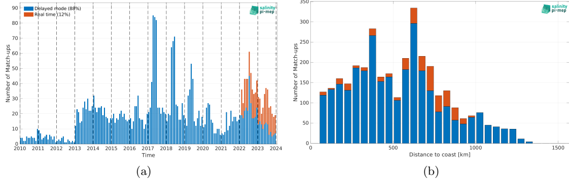
Figure 2: Number of match-ups between Argo and CCI SSS L4 Merged-OI v5.5 - 7-day running (ESA) SSS as a function of time (a) and as function of the distance to coast (b) over the Congo river plume Pi-MEP region and for the full satellite product period.
