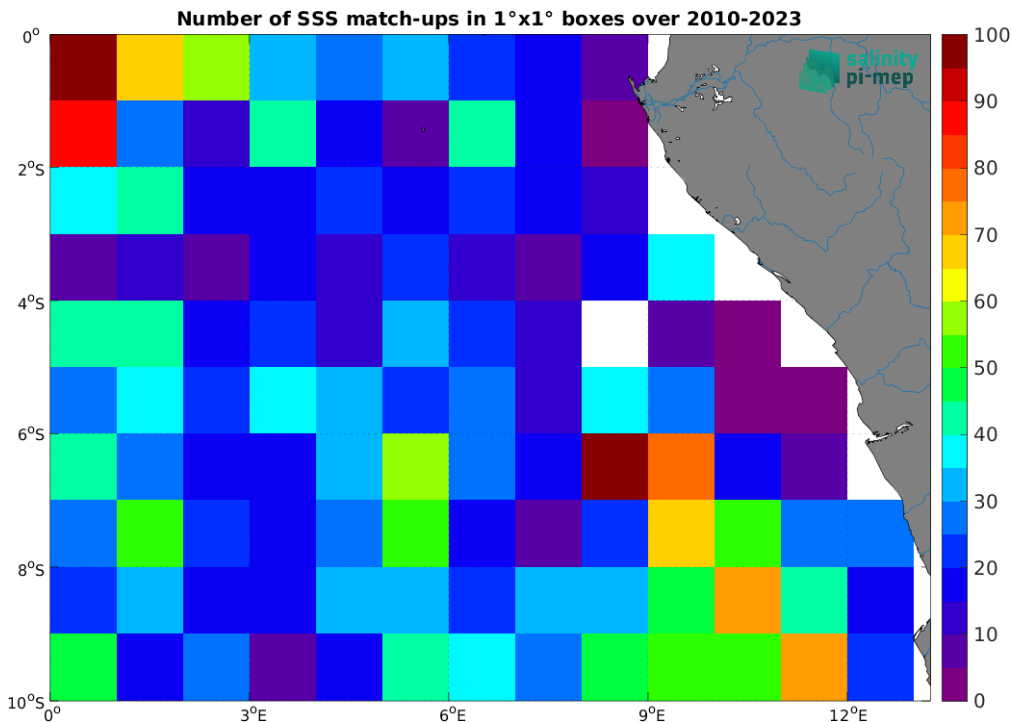
Figure 5: Number of SSS match-ups between Argo SSS and the CCI SSS L4 Merged-OI v5.5 - 7-day running (ESA) SSS product for the Congo river plume Pi-MEP region over 1^\circ \times 1^\circ boxes and for the full satellite product period.
