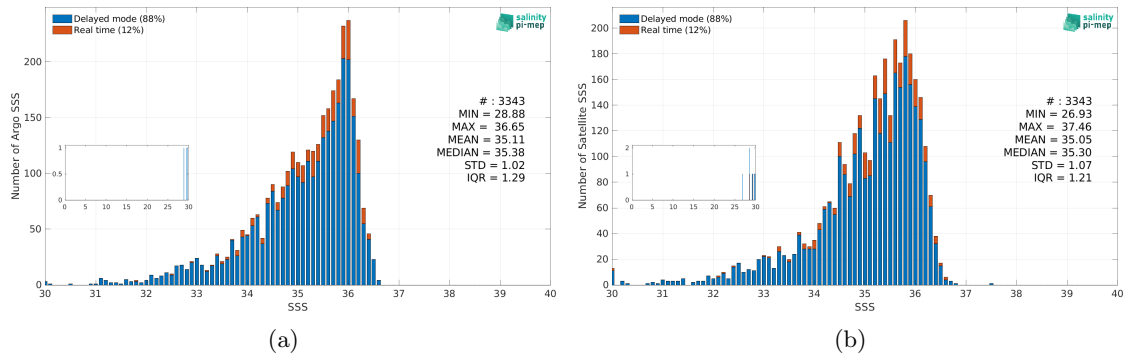
Figure 3: Histograms of SSS from Argo (a) and CCI SSS L4 Merged-OI v5.5 - 7-day running (ESA) (b) considering all match-up pairs per bins of 0.1 over the Congo river plume Pi-MEP region and for the full satellite product period.
