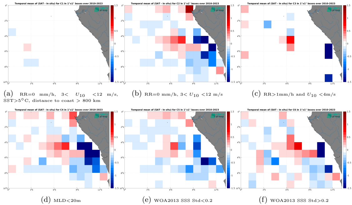
Figure 14: Temporal mean gridded over spatial boxes of size 1^\circ \times 1^\circ of \Delta\text{SSS} (CCI SSS L4 Merged-OI v5.5 - 7-day running (ESA) - Argo) for 6 different subdatasets corresponding to:RR=0 mm/h, 3 < U_{10} < 12 m/s, SST>5°C, distance to coast > 800 km (a), RR=0 mm/h, 3 < U_{10} < 12 m/s (b), RR>1mm/h and U_{10} < 4 m/s (c),MLD<20m (d),WOA2013 SSS Std<0.2 (e),WOA2013 SSS Std>0.2 (f).
