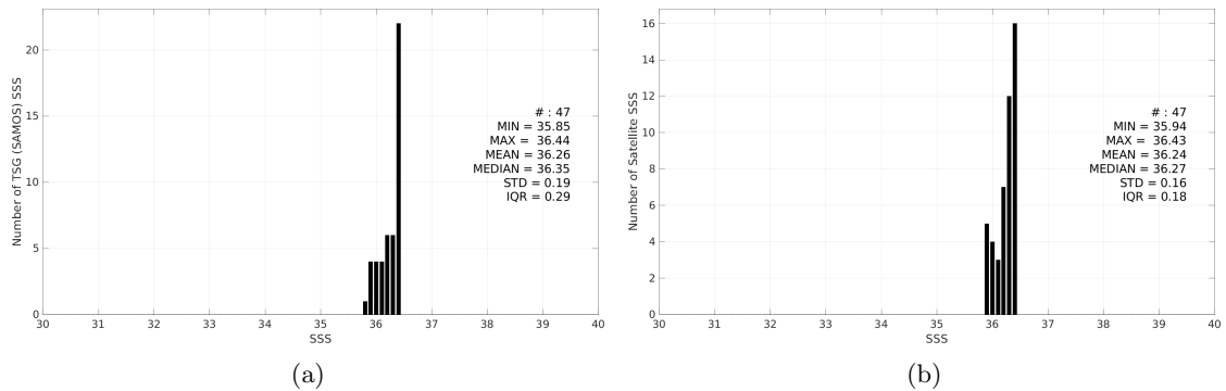
Figure 3: Histograms of SSS from TSG (SAMOS) (a) and CCI SSS L4 Merged-OI v5.5 - 30-day running (ESA) (b) considering all match-up pairs per bins of 0.1 over the Congo river plume Pi-MEP region and for the full satellite product period.
