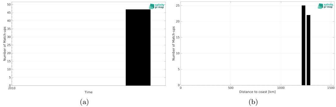
Figure 2: Number of match-ups between TSG (SAMOS) and CCI SSS L4 Merged-OI v5.5 - 30-day running (ESA) SSS as a function of time (a) and as function of the distance to coast (b) over the Congo river plume Pi-MEP region and for the full satellite product period.
