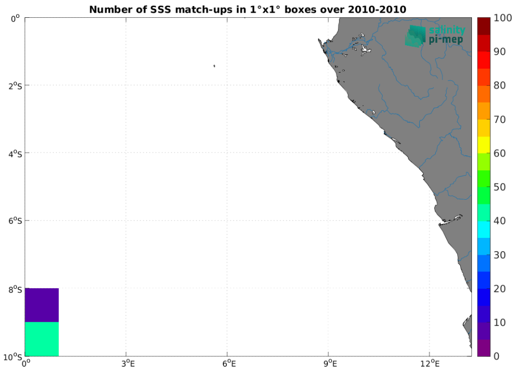
Figure 5: Number of SSS match-ups between TSG (SAMOS) SSS and the CCI SSS L4 Merged-OI v5.5 - 30-day running (ESA) SSS product for the Congo river plume Pi-MEP region over 1^\circ \times 1^\circ boxes and for the full satellite product period.
