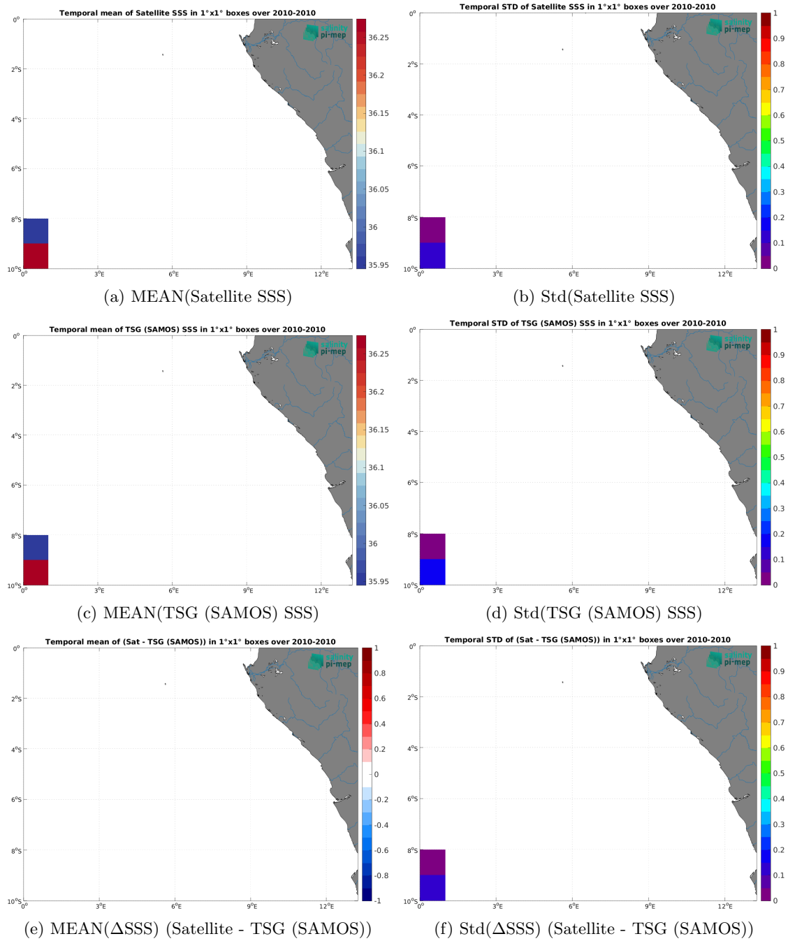
Figure 7: Temporal mean (left) and Std (right) of SSS from CCI SSS L4 Merged-OI v5.5 - 30-day running (ESA) (top), TSG (SAMOS) (middle), and of \Delta SSS (Satellite - TSG (SAMOS)). Only match-up pairs are used to generate these maps.
