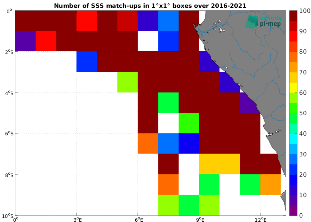
Figure 5: Number of SSS match-ups between TSG (LEGOS-DM) SSS and the CCI SSS L4 Merged-OI v5.5 - 30-day running (ESA) SSS product for the Congo river plume Pi-MEP region over 1^\circ \times 1^\circ boxes and for the full satellite product period.
