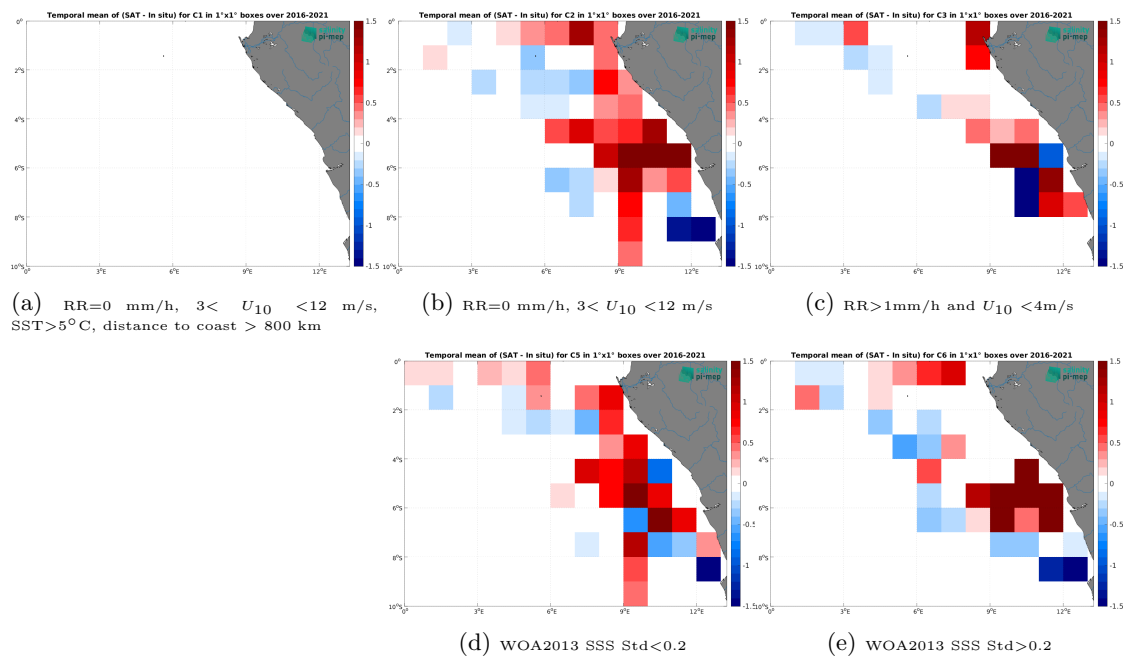
Figure 14: Temporal mean gridded over spatial boxes of size 1^\circ \times 1^\circ of \Delta SSS (CCI SSS L4 Merged-OI v5.5 - 30-day running (ESA) - TSG (LEGOS-DM)) for 5 different subdatasets corresponding to:RR=0 mm/h, 3 < U_{10} < 12 m/s, SST >5^\circ C, distance to coast > 800 km (a), RR=0 mm/h, 3 < U_{10} < 12 m/s (b), RR >1 mm/h and U_{10} < 4 m/s (c), WOA2013 SSS Std <0.2 (d), WOA2013 SSS Std >0.2 (e).
