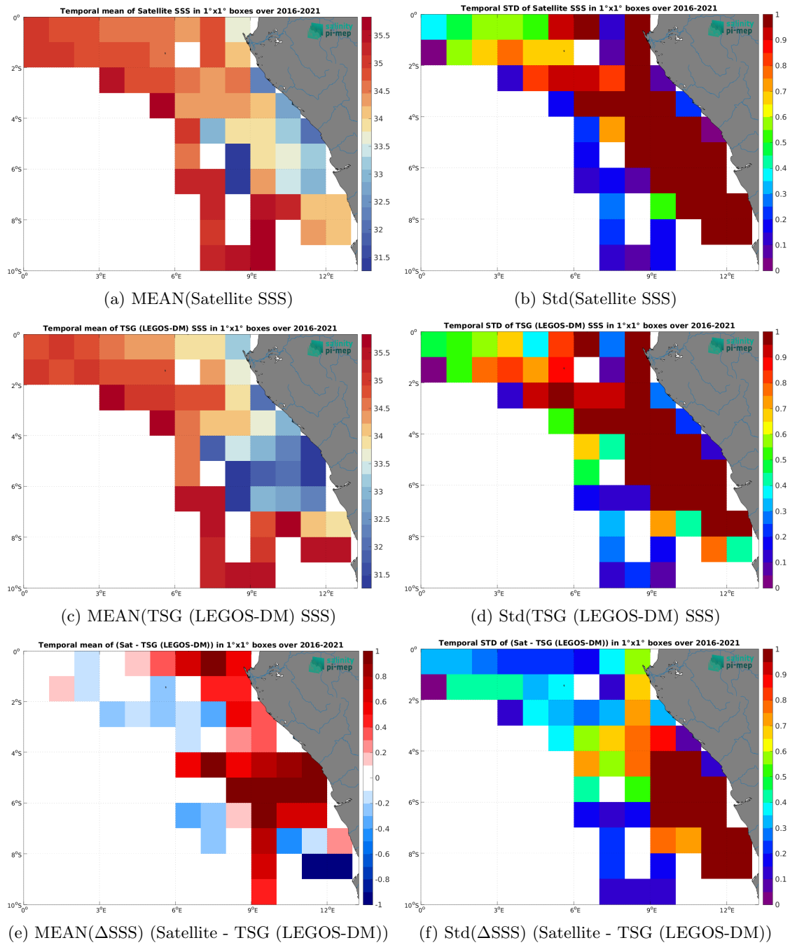
Figure 7: Temporal mean (left) and Std (right) of SSS from CCI SSS L4 Merged-OI v5.5 - 30-day running (ESA) (top), TSG (LEGOS-DM) (middle), and of \Delta SSS (Satellite - TSG (LEGOS-DM)). Only match-up pairs are used to generate these maps.
