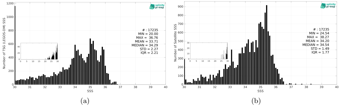
Figure 3: Histograms of SSS from TSG (LEGOS-DM) (a) and CCI SSS L4 Merged-OI v5.5 - 30-day running (ESA) (b) considering all match-up pairs per bins of 0.1 over the Congo river plume Pi-MEP region and for the full satellite product period.
