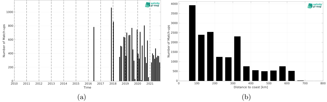
Figure 2: Number of match-ups between TSG (LEGOS-DM) and CCI SSS L4 Merged-OI v5.5 - 30-day running (ESA) SSS as a function of time (a) and as function of the distance to coast (b) over the Congo river plume Pi-MEP region and for the full satellite product period.
