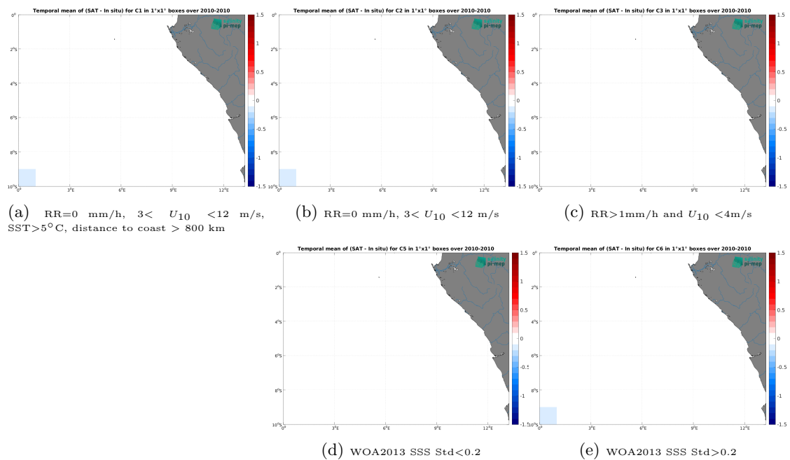
Figure 14: Temporal mean gridded over spatial boxes of size 1^\circ \times 1^\circ of \Delta SSS (CCI SSS L4 Merged-OI v4.41 - 7-day running (ESA) - TSG (SAMOS)) for 5 different subdatasets corresponding to:RR=0 mm/h, 3 < U_{10} < 12 m/s, SST > 5^\circ\text{C} , distance to coast > 800 km (a), RR=0 mm/h, 3 < U_{10} < 12 m/s (b), RR > 1 mm/h and U_{10} < 4 m/s (c), WOA2013 SSS Std < 0.2 (d), WOA2013 SSS Std > 0.2 (e).
