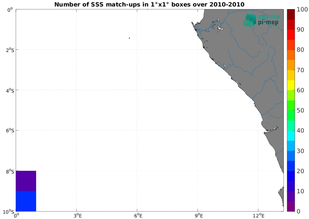
Figure 5: Number of SSS match-ups between TSG (SAMOS) SSS and the CCI SSS L4 Merged-OI v4.41 - 7-day running (ESA) SSS product for the Congo river plume Pi-MEP region over 1^\circ \times 1^\circ boxes and for the full satellite product period.
