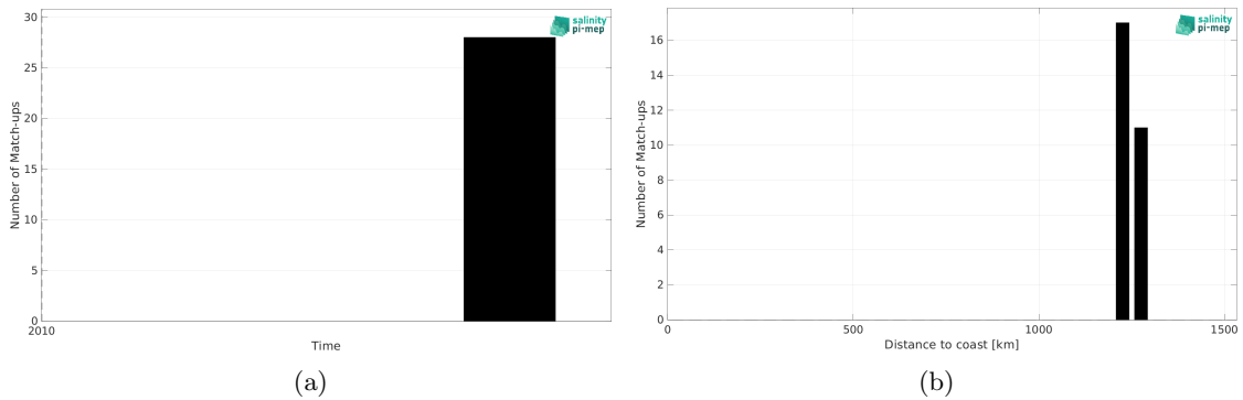
Figure 2: Number of match-ups between TSG (SAMOS) and CCI SSS L4 Merged-OI v4.41 - 7-day running (ESA) SSS as a function of time (a) and as function of the distance to coast (b) over the Congo river plume Pi-MEP region and for the full satellite product period.
