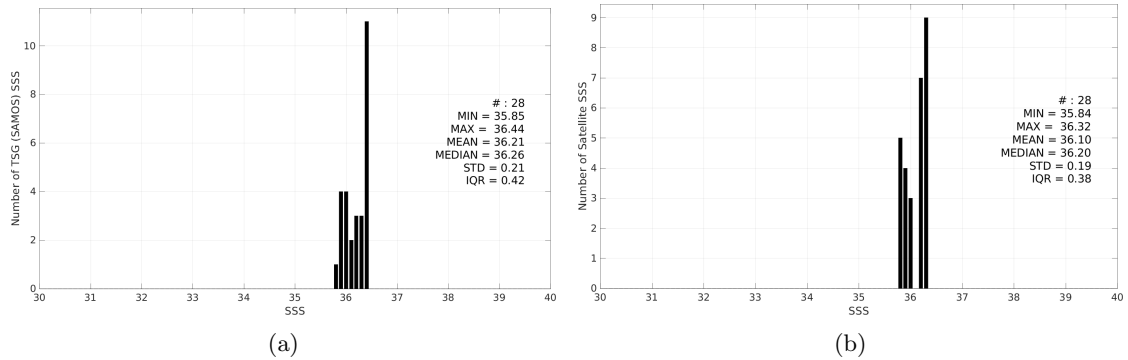
Figure 3: Histograms of SSS from TSG (SAMOS) (a) and CCI SSS L4 Merged-OI v4.41 - 7-day running (ESA) (b) considering all match-up pairs per bins of 0.1 over the Congo river plume Pi-MEP region and for the full satellite product period.
