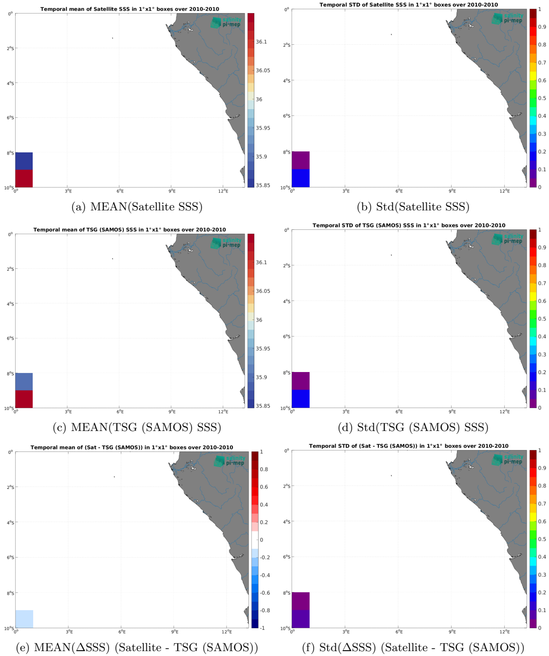
Figure 7: Temporal mean (left) and Std (right) of SSS from CCI SSS L4 Merged-OI v4.41 - 7-day running (ESA) (top), TSG (SAMOS) (middle), and of \Delta SSS (Satellite - TSG (SAMOS)). Only match-up pairs are used to generate these maps.
