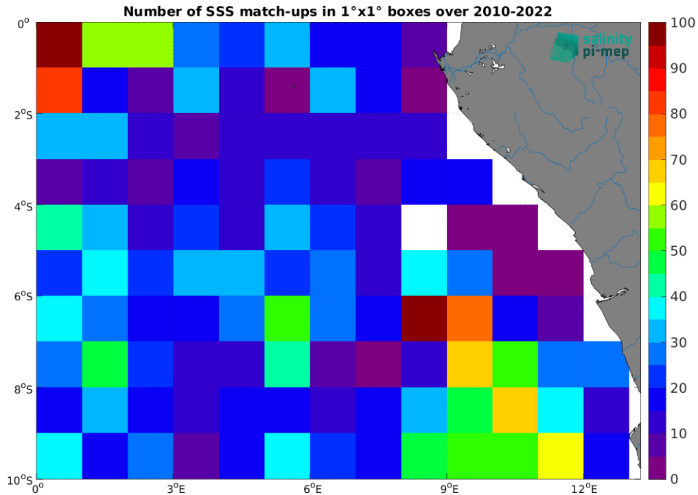
Figure 5: Number of SSS match-ups between Argo SSS and the CCI SSS L4 Merged-OI v4.41 - 7-day running (ESA) SSS product for the Congo river plume Pi-MEP region over 1^\circ \times 1^\circ boxes and for the full satellite product period.
