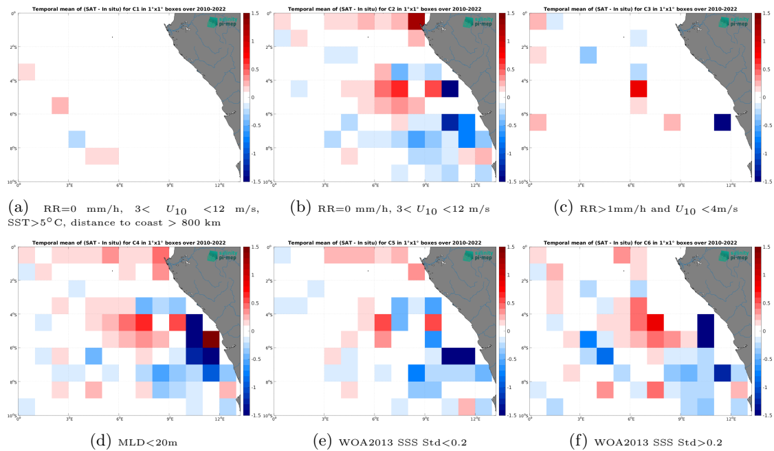
Figure 14: Temporal mean gridded over spatial boxes of size 1^\circ \times 1^\circ of \Delta SSS (CCI SSS L4 Merged-OI v4.41 - 7-day running (ESA) - Argo) for 6 different subdatasets corresponding to:RR=0 mm/h, 3 < U_{10} < 12 m/s, SST >5^\circ C, distance to coast > 800 km (a), RR=0 mm/h, 3 < U_{10} < 12 m/s (b), RR >1 mm/h and U_{10} < 4 m/s (c),MLD <20 m (d),WOA2013 SSS Std <0.2 (e),WOA2013 SSS Std >0.2 (f).
