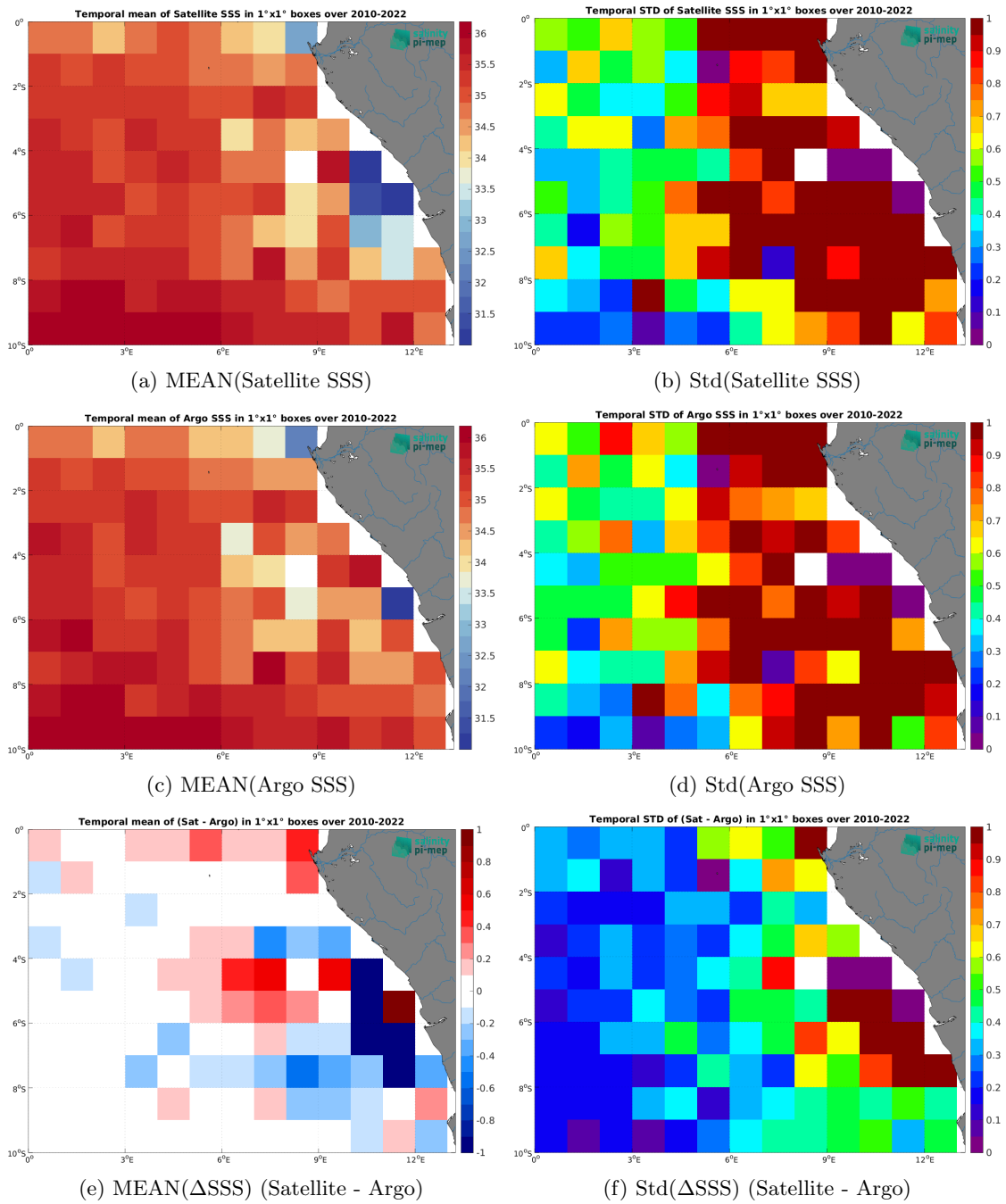
Figure 7: Temporal mean (left) and Std (right) of SSS from CCI SSS L4 Merged-OI v4.41 - 7-day running (ESA) (top), Argo (middle), and of \Delta SSS (Satellite - Argo). Only match-up pairs are used to generate these maps.
