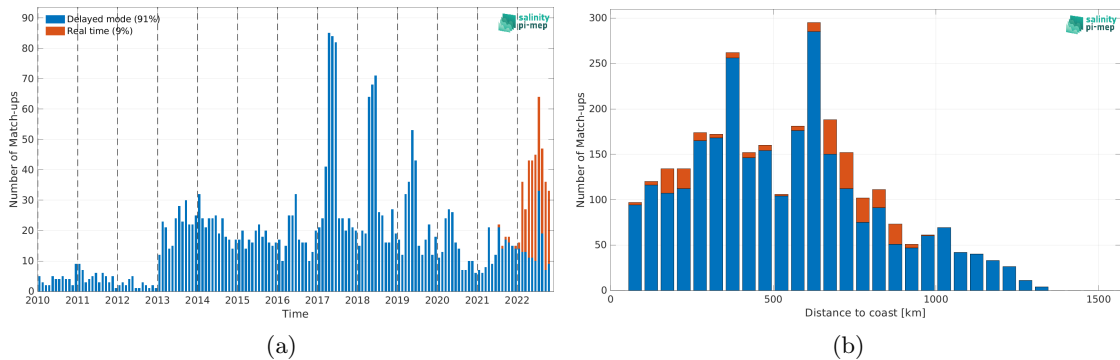
Figure 2: Number of match-ups between Argo and CCI SSS L4 Merged-OI v4.41 - 7-day running (ESA) SSS as a function of time (a) and as function of the distance to coast (b) over the Congo river plume Pi-MEP region and for the full satellite product period.
