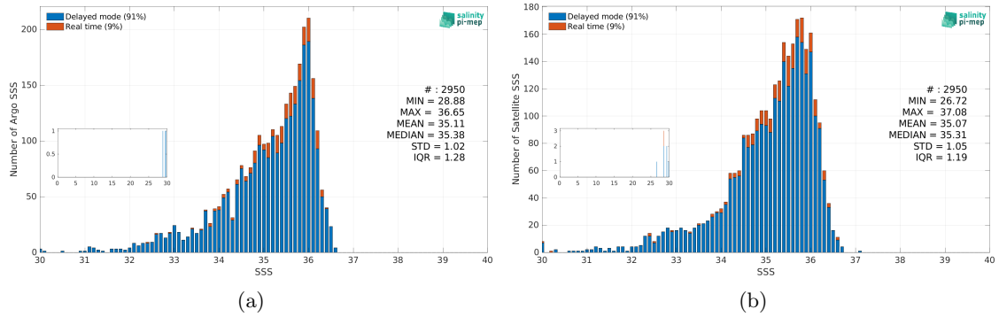
Figure 3: Histograms of SSS from Argo (a) and CCI SSS L4 Merged-OI v4.41 - 7-day running (ESA) (b) considering all match-up pairs per bins of 0.1 over the Congo river plume Pi-MEP region and for the full satellite product period.
