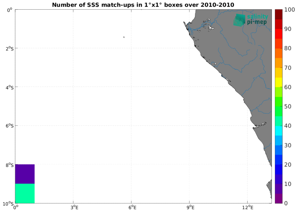
Figure 5: Number of SSS match-ups between TSG (SAMOS) SSS and the CCI SSS L4 Merged-OI v4.41 - 30-day running (ESA) SSS product for the Congo river plume Pi-MEP region over 1^\circ \times 1^\circ boxes and for the full satellite product period.
