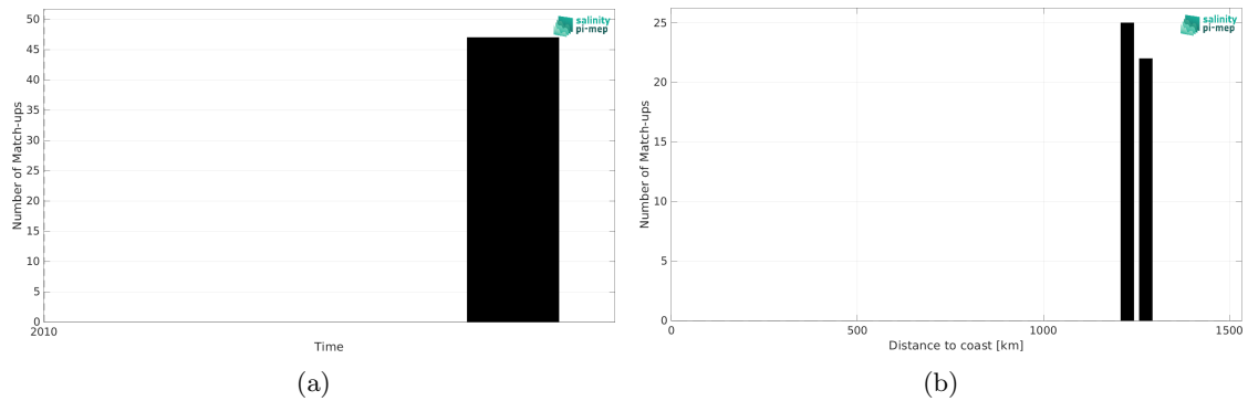
Figure 2: Number of match-ups between TSG (SAMOS) and CCI SSS L4 Merged-OI v4.41 - 30-day running (ESA) SSS as a function of time (a) and as function of the distance to coast (b) over the Congo river plume Pi-MEP region and for the full satellite product period.
