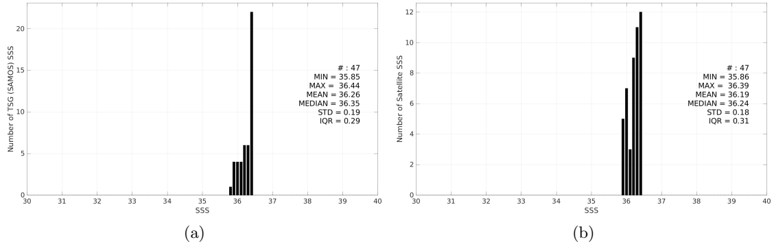
Figure 3: Histograms of SSS from TSG (SAMOS) (a) and CCI SSS L4 Merged-OI v4.41 - 30-day running (ESA) (b) considering all match-up pairs per bins of 0.1 over the Congo river plume Pi-MEP region and for the full satellite product period.
